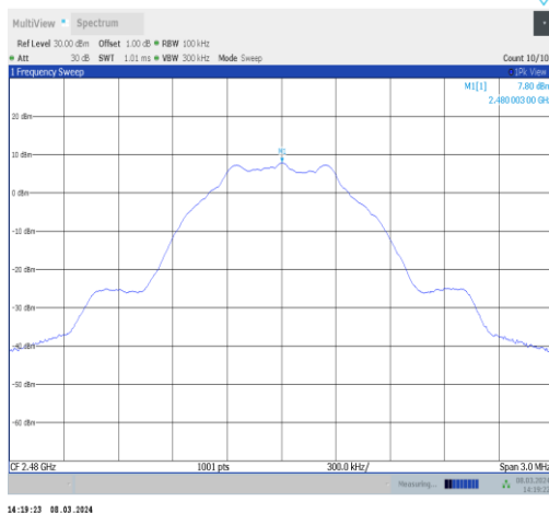
BLE_1M-Ant10-2480-0~Reference-PASS
