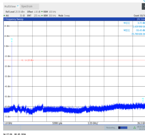
BLE_1M-Ant10-2440-1000~26500-PASS
