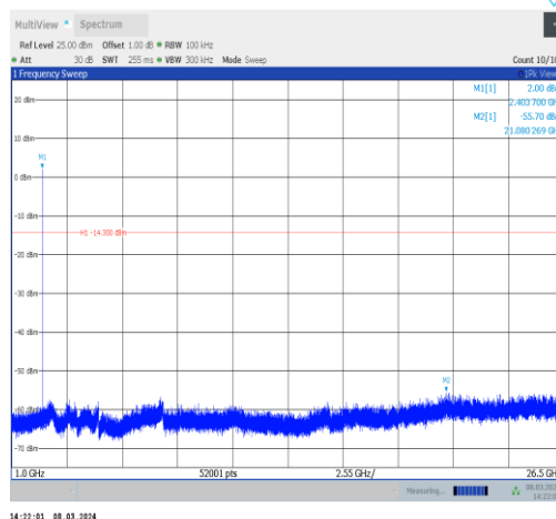
BLE_2M-Ant10-2404-1000~26500-PASS
