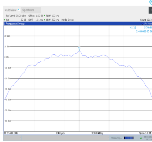
BLE_2M-Ant10-2404-0~Reference-PASS
