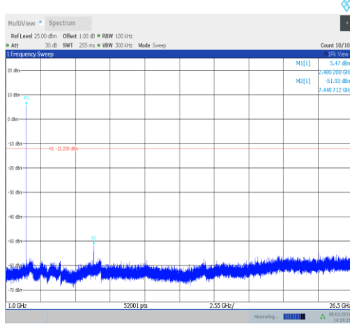
BLE_1M-Ant10-2480-1000~26500-PASS
