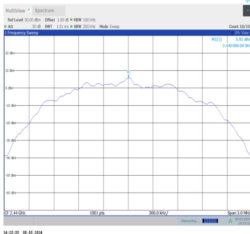
BLE_2M-Ant10-2440-0~Reference-PASS
