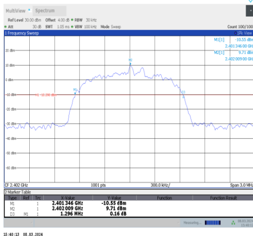
3DH5-Ant10-2402
