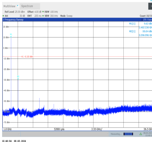
3DH5-Ant10-2402-1000~26500-PASS
