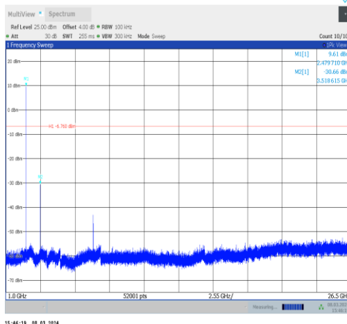
3DH5-Ant10-2480-1000~26500-PASS
