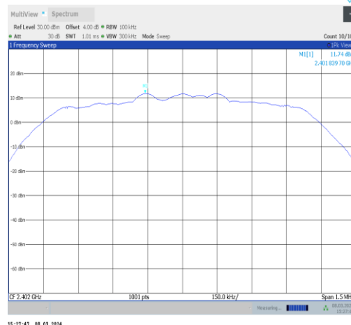
2DH5-Ant10-2402-0~Reference-PASS
