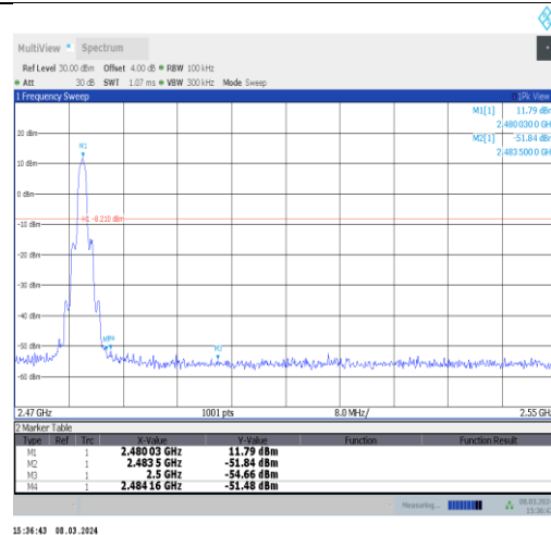
2DH5-Ant10-2480-PASS
