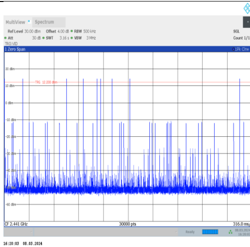
DH5-Ant10-Hop-PASS
