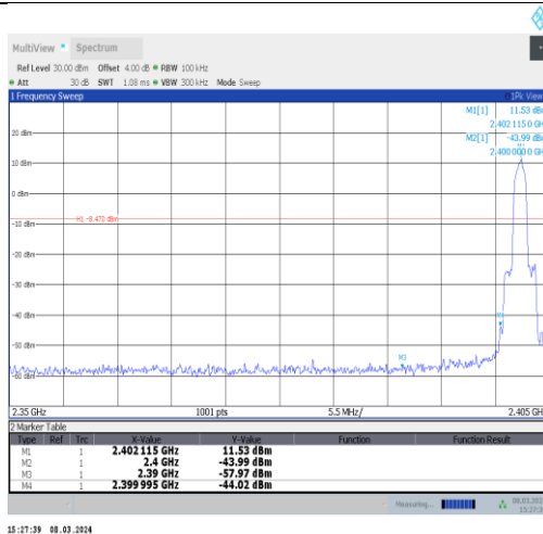
2DH5-Ant10-2402-PASS
