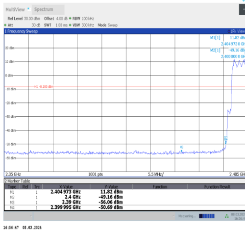
2DH5-Ant10-Hop_2402-PASS
