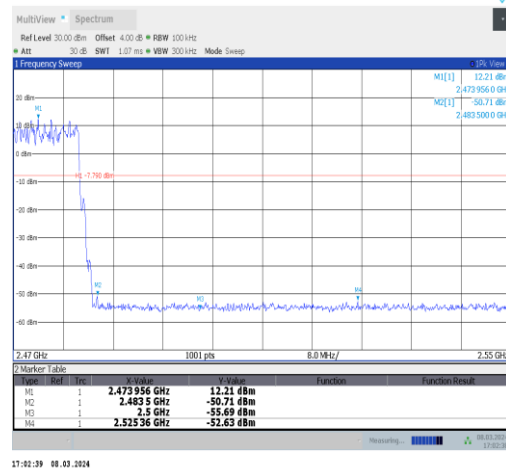
2DH5-Ant10-Hop_2480-PASS
