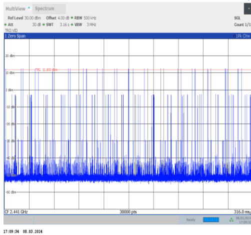
3DH1-Ant10-Hop-PASS
