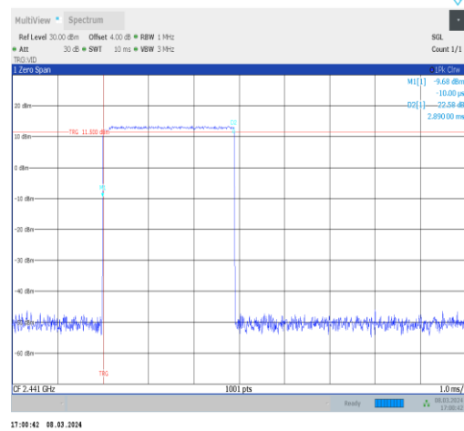
2DH5-Ant10-Hop-PASS
