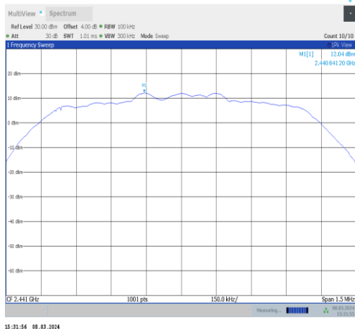
2DH5-Ant10-2441-0~Reference-PASS
