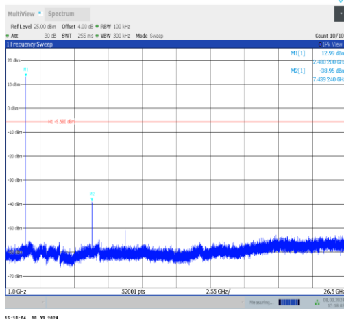
DH5-Ant10-2480-1000~26500-PASS
