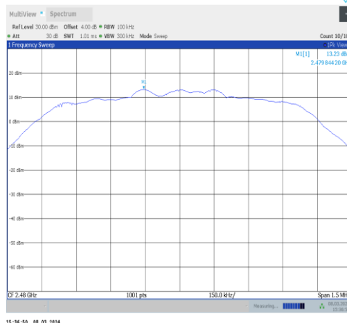
2DH5-Ant10-2480-0~Reference-PASS
