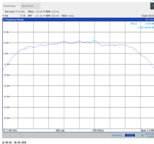
3DH5-Ant10-2402-0~Reference-PASS
