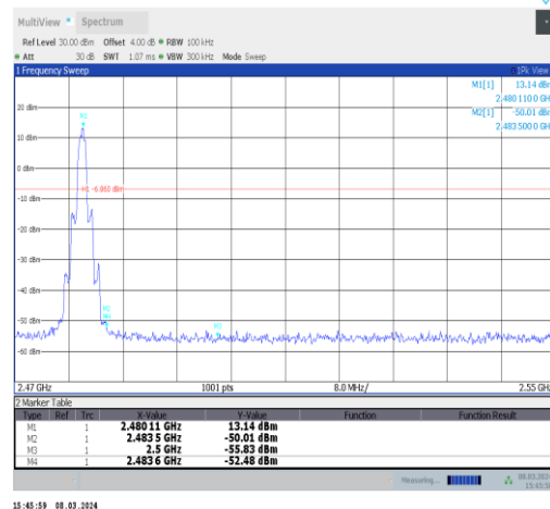
3DH5-Ant10-2480-PASS
