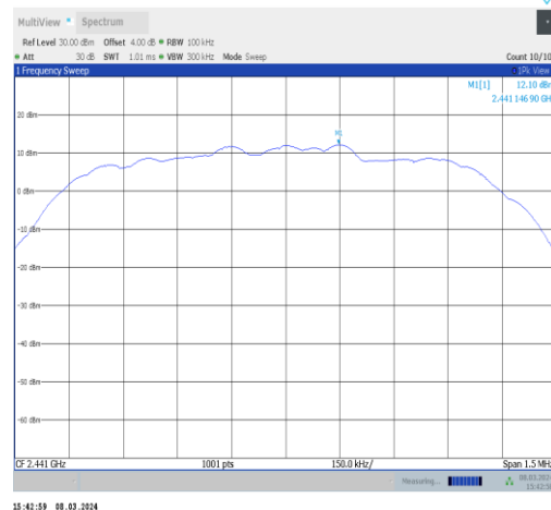
3DH5-Ant10-2441-0~Reference-PASS
