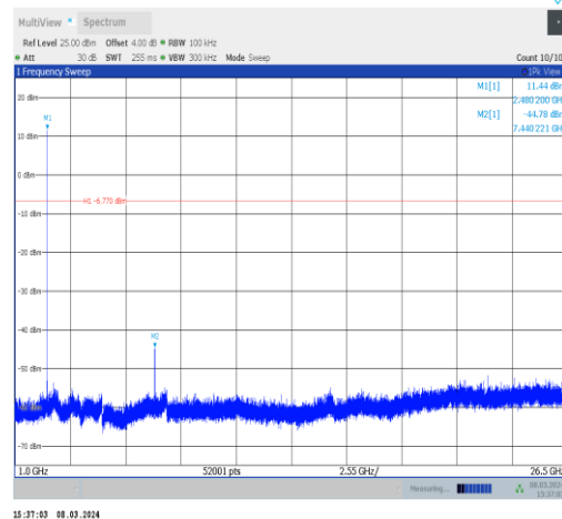
2DH5-Ant10-2480-1000~26500-PASS
