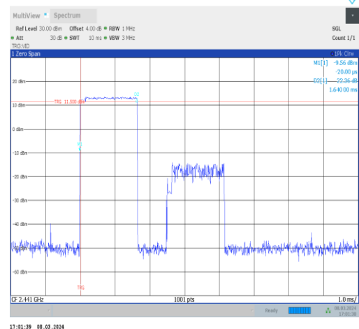
2DH3-Ant10-Hop-PASS
