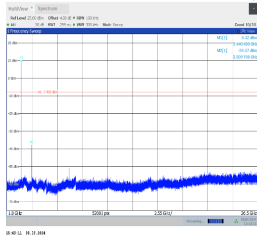
3DH5-Ant10-2441-1000~26500-PASS
