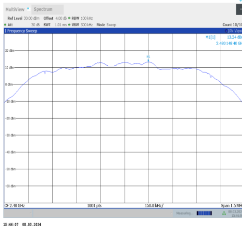
3DH5-Ant10-2480-0~Reference-PASS
