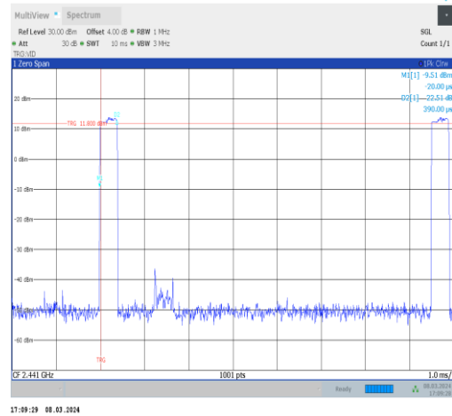
3DH1-Ant10-Hop-PASS
