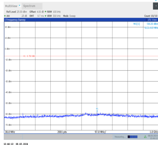
3DH5-Ant10-2480-30~1000-PASS
