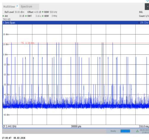
2DH5-Ant10-Hop-PASS
