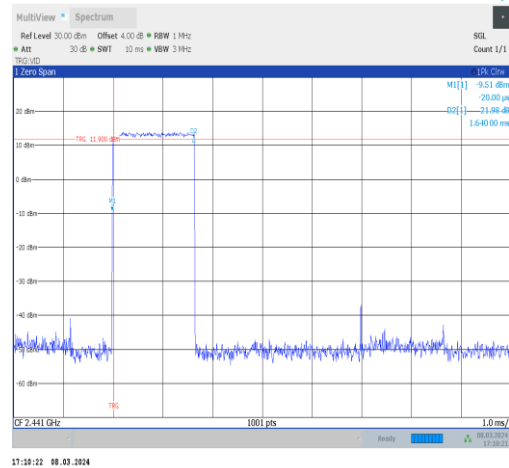
3DH3-Ant10-Hop-PASS
