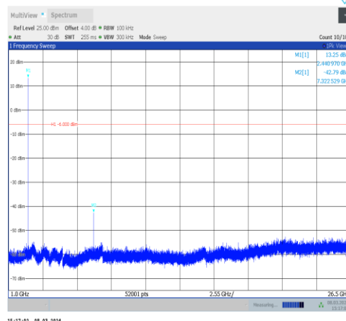
DH5-Ant10-2441-1000~26500-PASS
