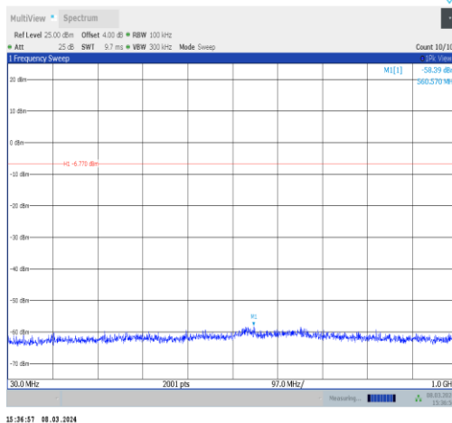
2DH5-Ant10-2480-30~1000-PASS
