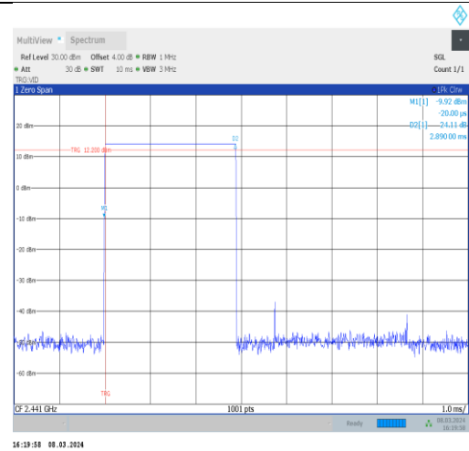
DH5-Ant10-Hop-PASS
