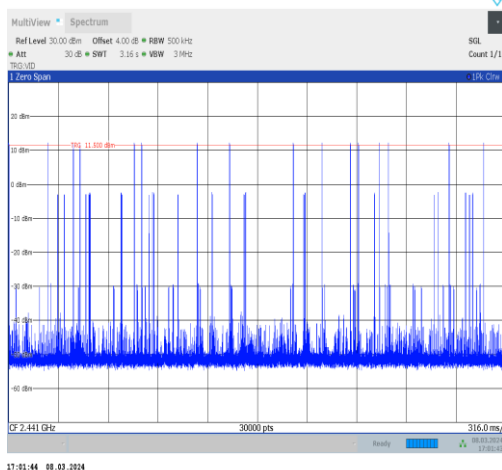
2DH3-Ant10-Hop-PASS
