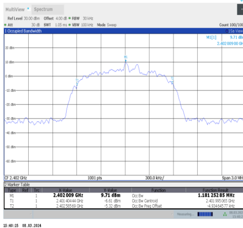
3DH5-Ant10-2402
