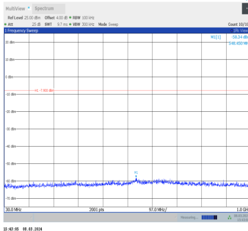
3DH5-Ant10-2441-30~1000-PASS
