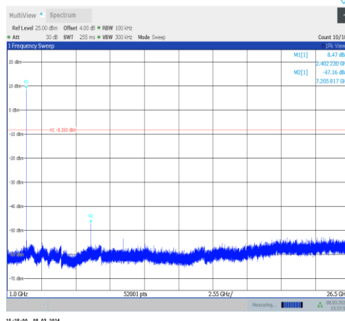
2DH5-Ant10-2402-1000~26500-PASS
