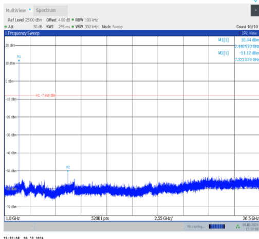
2DH5-Ant10-2441-1000~26500-PASS
