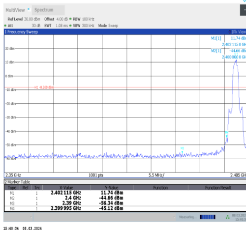
3DH5-Ant10-2402-PASS
