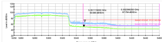
802.11ac VHT80 -Channel 58: Peak + Average
