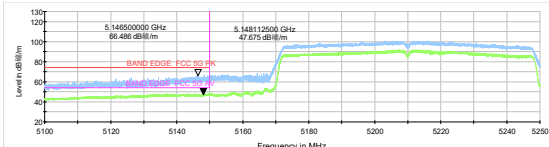
802.11ac VHT80 –Channel 42: Peak + Average
