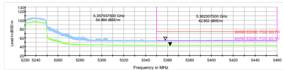
802.11n HT40-Channel 46: Peak + Average
