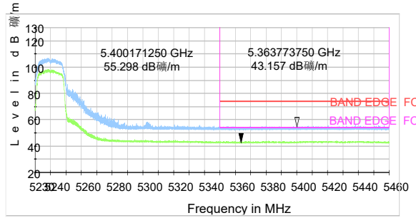
802.11n HT20-Channel 48: Peak + Average
