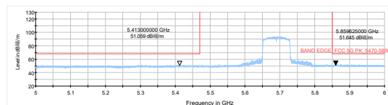
802.11ac VHT80-Channel 138: Peak
