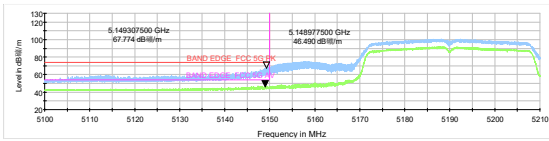
802.11ac VHT40-Channel 38: Peak + Average
