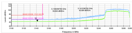
802.11ac VHT80 -Channel 58: Peak + Average
