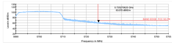
802.11a-Channel 144: Peak
