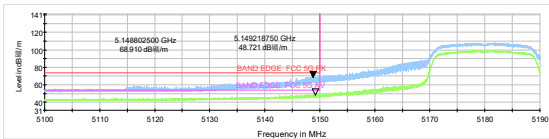
802.11n HT40-Channel 38: Peak + Average
