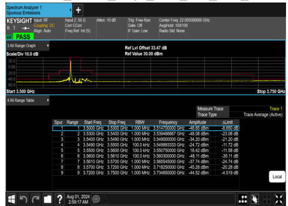
N48(10M)_DFT-s- OFDM_QPSK_Edge_1RB_Left_Low_CH
