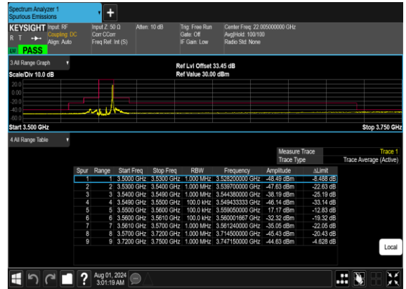
N48(10M)_DFT-s- OFDM_QPSK_Edge_1RB_Right_Low_CH
