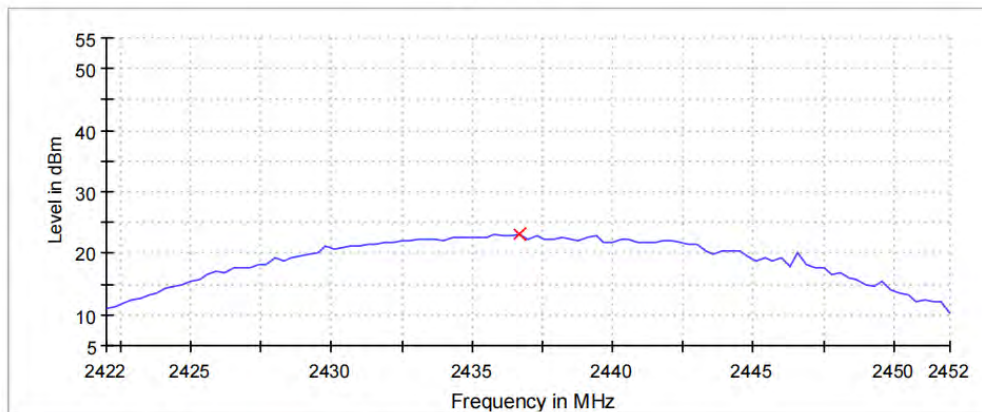
Peak Power
