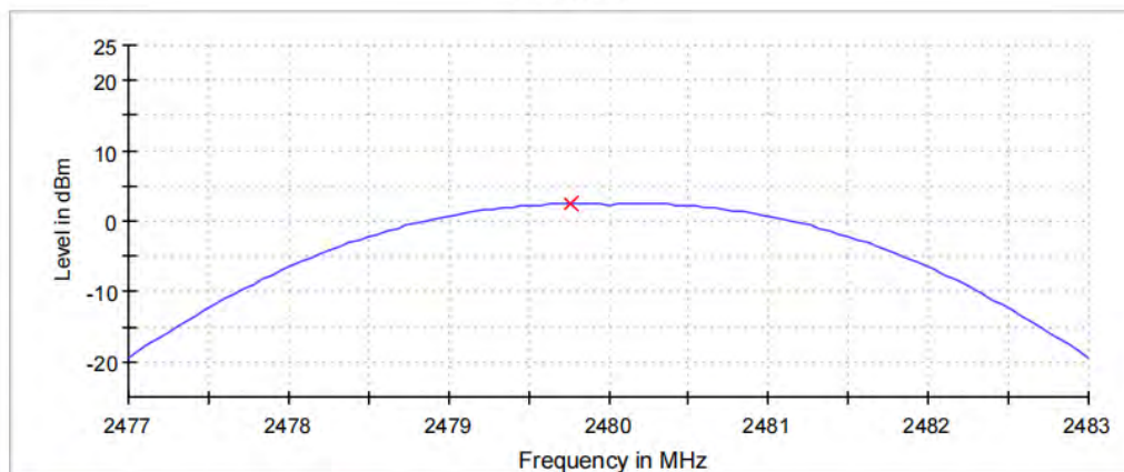
Peak Power
