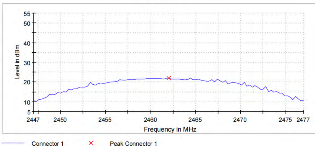
Peak Power
