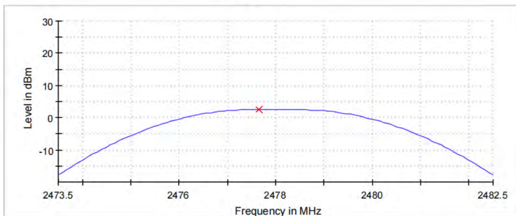
Peak Power
