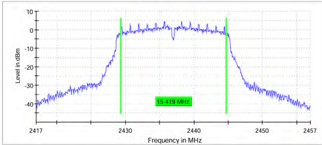
6 dB Bandwidth
