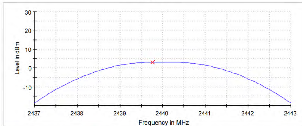
Peak Power
