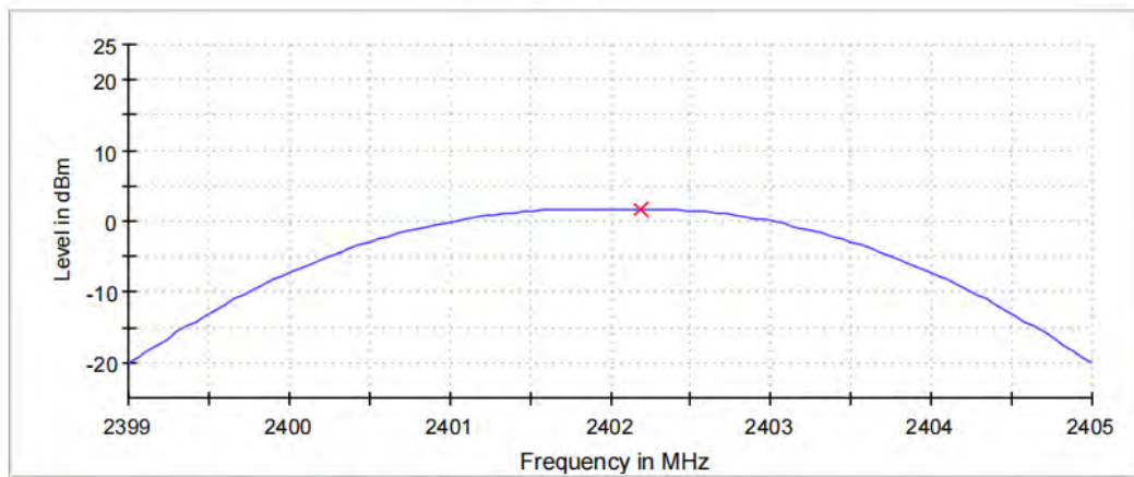
Peak Power
