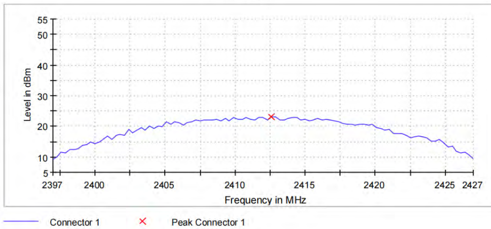
Peak Power
