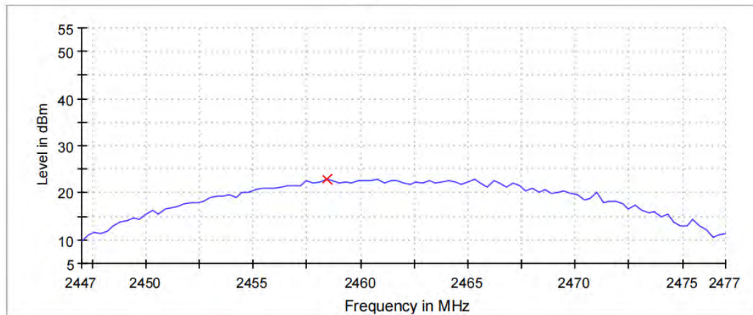
Peak Power
