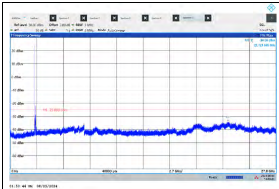
NTN-N41-PC3-15-50-L-DFT-QPSK-Edge_1RB_ Left-Ant1-PASS
