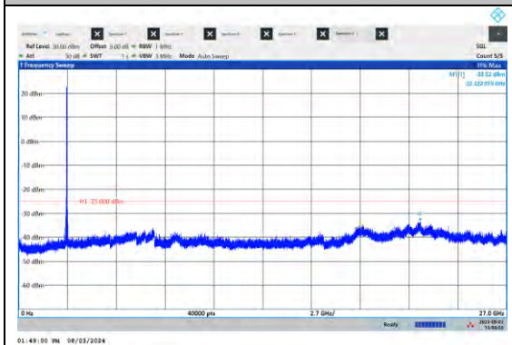
NTN-N41-PC3-15-50-H-DFT-QPSK-Edge_1RB_ Left-Ant1-PAS
