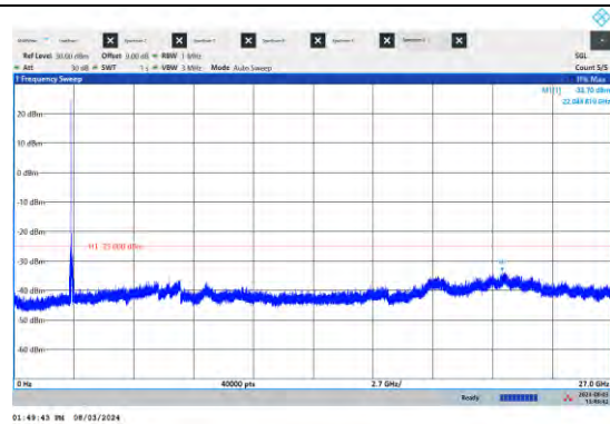
NTN-N41-PC3-15-50-M-DFT-QPSK-Edge_1RB_ Left-Ant1-PASS
