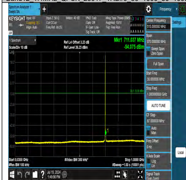
Band12 1.4MHz QPSK 23095 1RB#0 30~1000 30~1000
