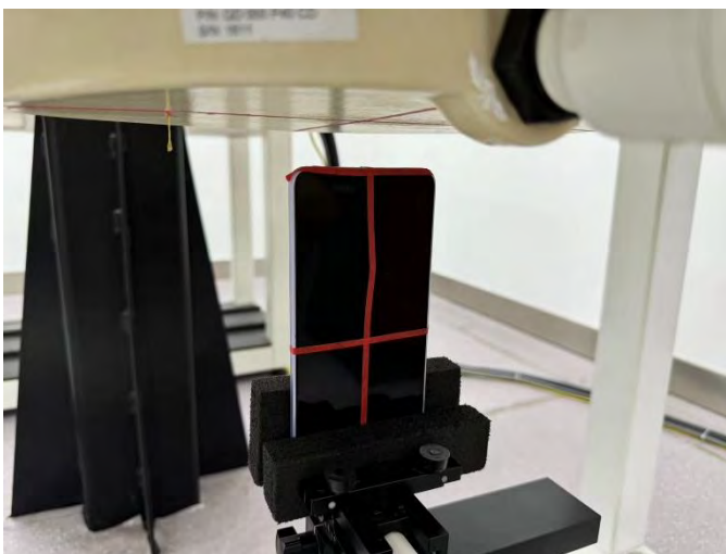
Top Side of EUT with 2.0 cm Gap (Body-Worn Mode)
