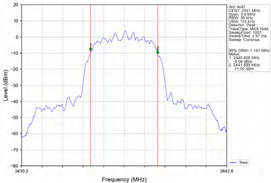
Pi/4DQPSK_2DH5_MCH_2441MHz_Ant7_NTNV
