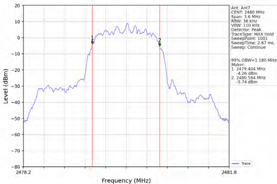
Pi/4DQPSK_2DH5_HCH_2480MHz_Ant7_NTNV
