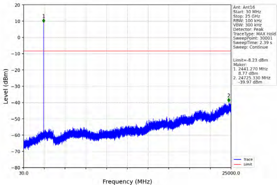
Pi/4DQPSK_2DH5_MCH_2441MHz_Ant16_NTNV
