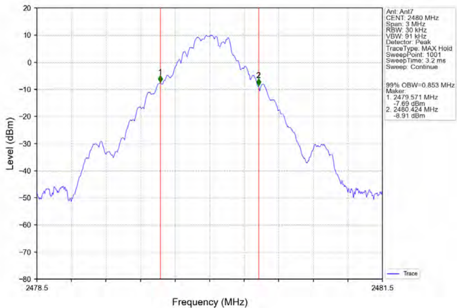
GFSK_DH5_HCH_2480MHz_Ant7_NTNV
