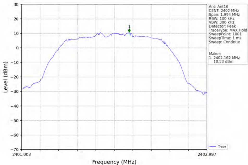
PI/4DQPSK_2DH5_LCH_2402MHz_Ant16_NTNV
