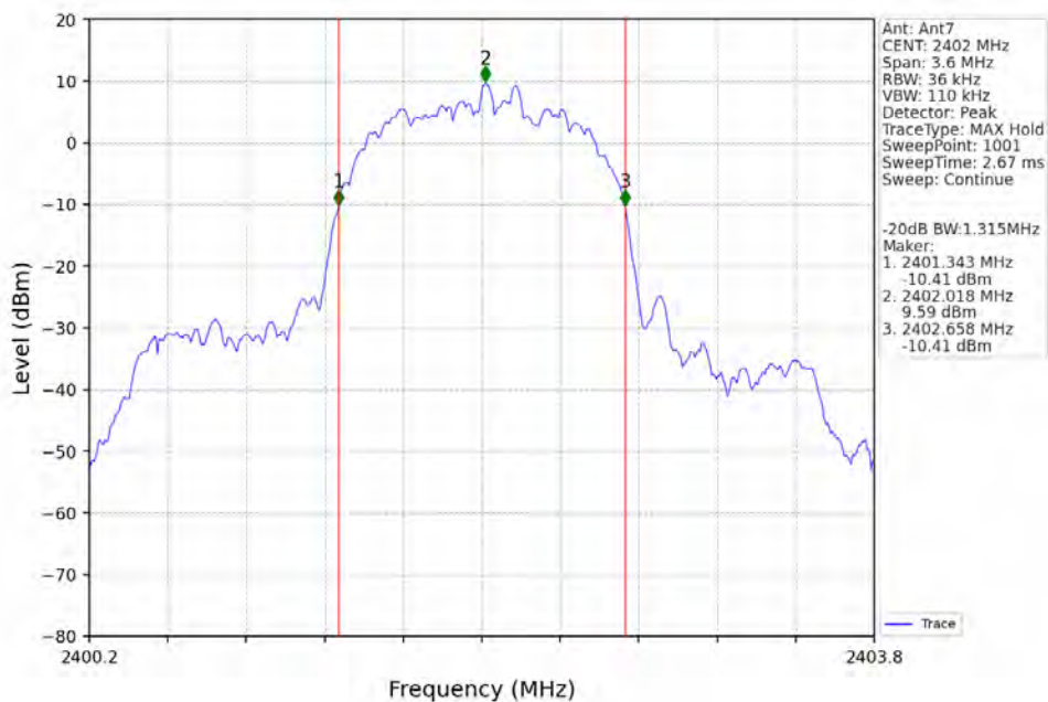
8DPSK_3DH5_MCH_2441MHz_Ant7_NTNV
