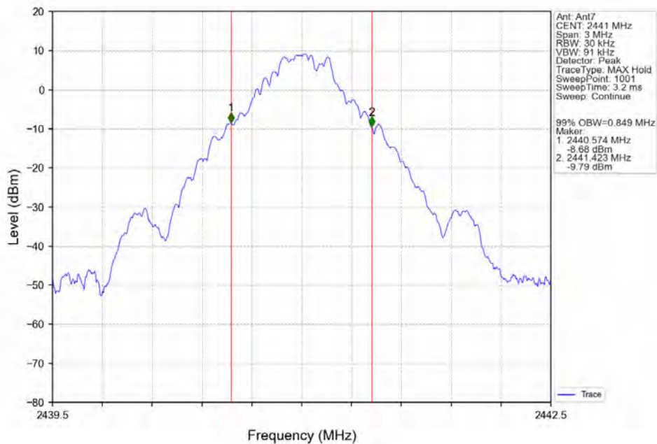
GFSK_DH5_MCH_2441MHz_Ant7_NTNV
