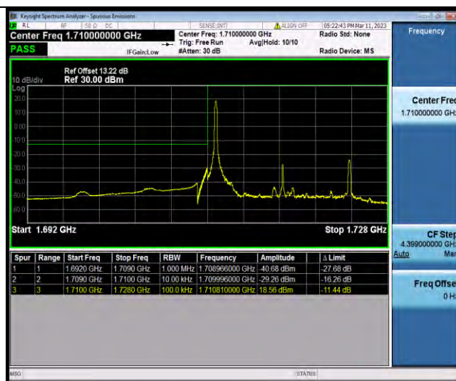
Band66-15MHz-64QAM-132047-75RB#0
