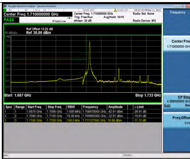
Band66-20MHz-64QAM-132072-100RB#0
