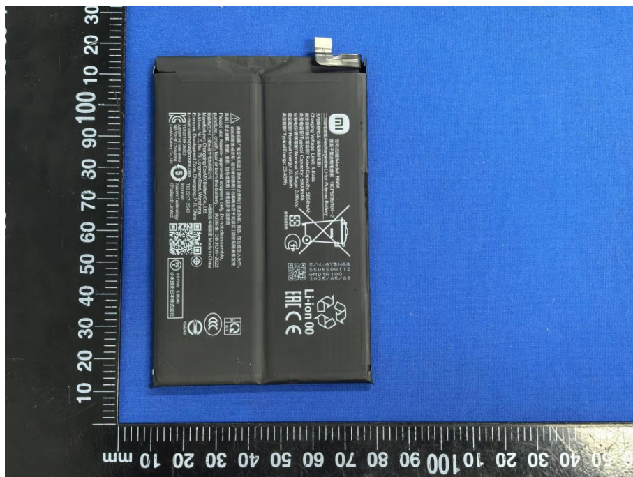
BATTERY 1 TOP VIEW
