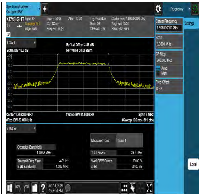
Band2-1.4MHz-16QAM-19193-6RB#0-PASS
