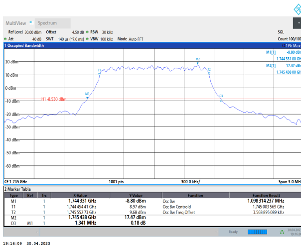
Band66-1.4MHz-QPSK-132322-6RB#0
