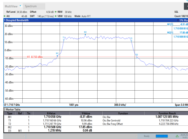
Band4-1.4MHz-QPSK-20175-6RB#0
