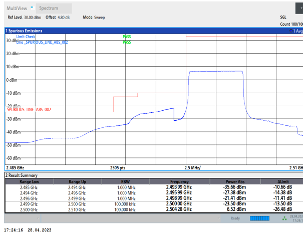
Band7-5MHz-QPSK-20775-25RB#0
