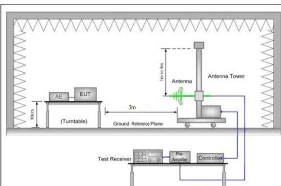
Figure 2. Above 30MHz
