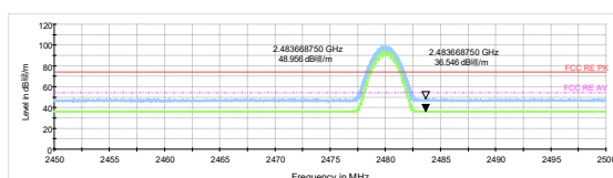
3DH5-Channel 78: Peak + Average
