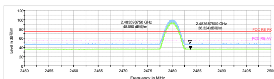
DH5-Channel 78: Peak + Average
