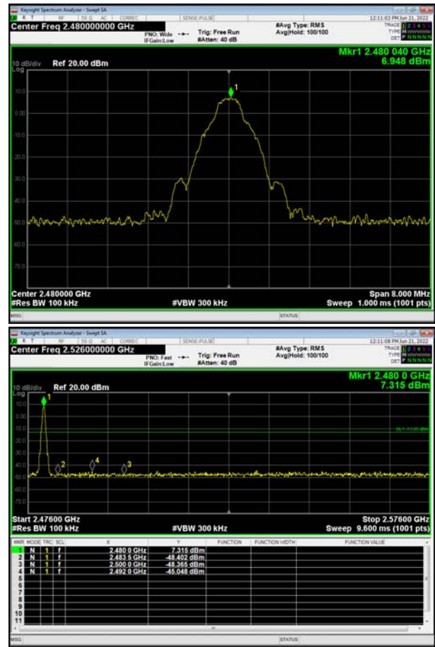
BT DH5 CH78, Carrier frequency (MHz): 2480
