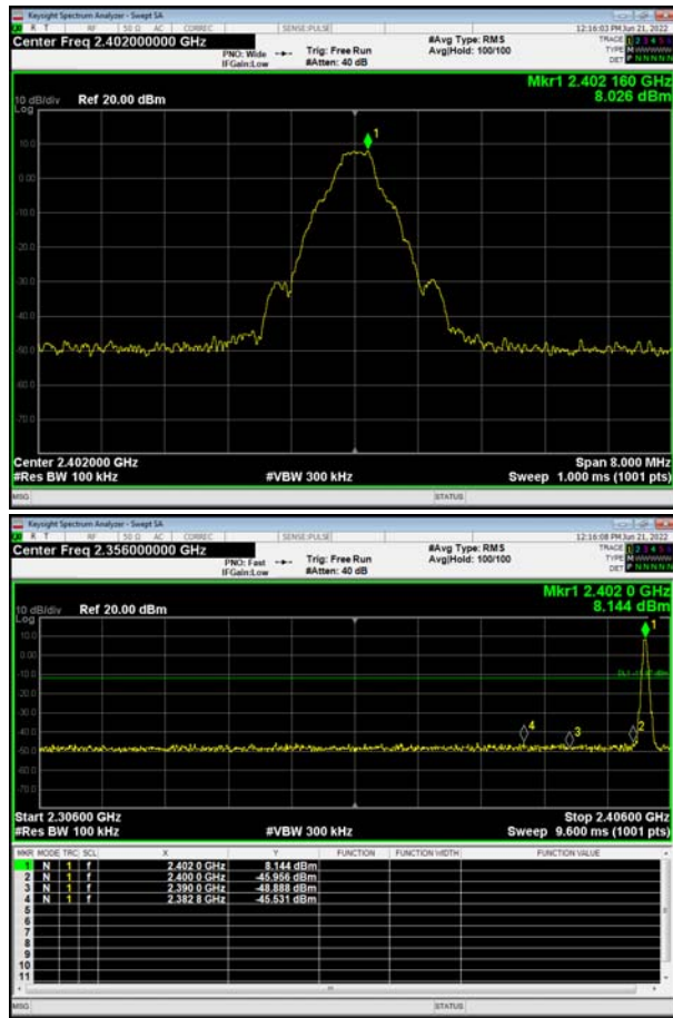
BT DH5 CH0, Carrier frequency (MHz): 2402
