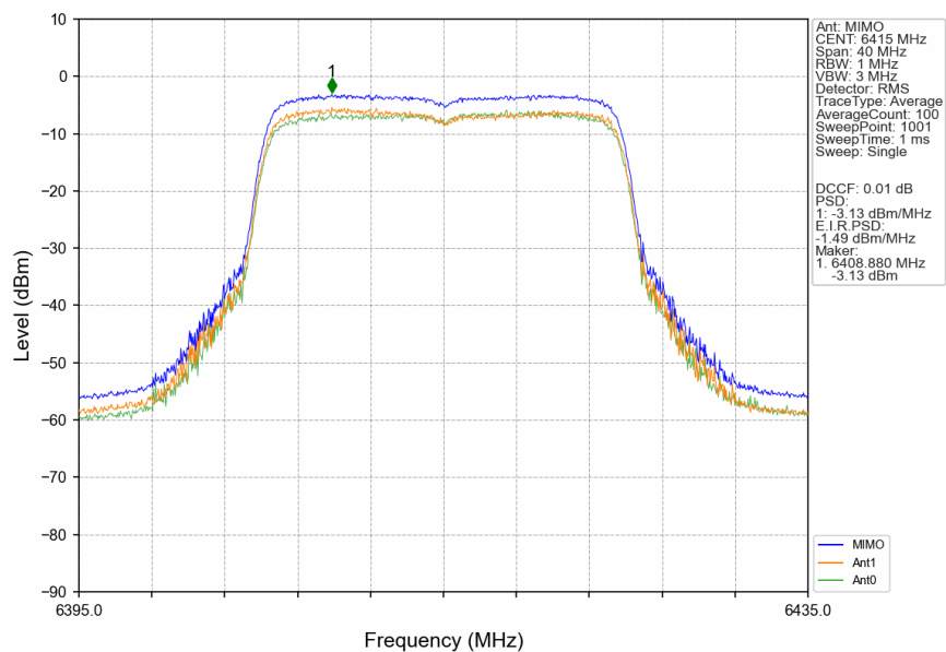
802.11be(EHT20)_HCH_6415MHz_RU242_Left_MIMO_NTNV
