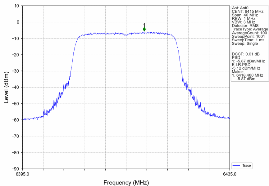
802.11be(EHT20)_HCH_6415MHz_RU242_Left_MIMO_NTNV
