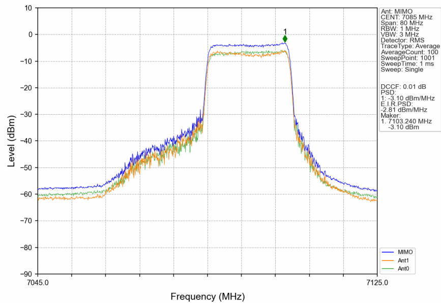
802.11be(EHT40)_HCH_7085MHz_RU242_Right_MIMO_NTNV
