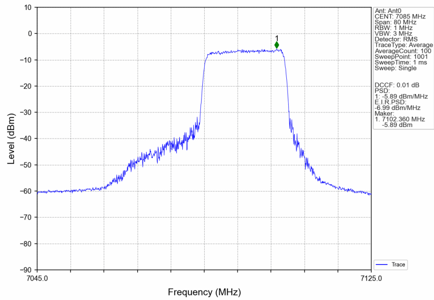
802.11be(EHT40)_HCH_7085MHz_RU242_Right_MIMO_NTNV
