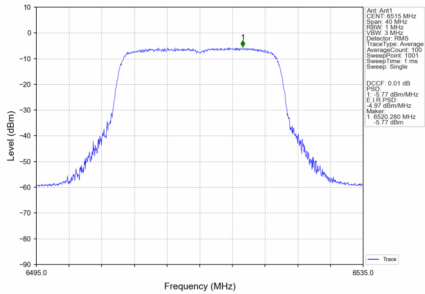
802.11ax(HEW20)_HCH_6515MHz_RU242_Left_MIMO_NTNV
