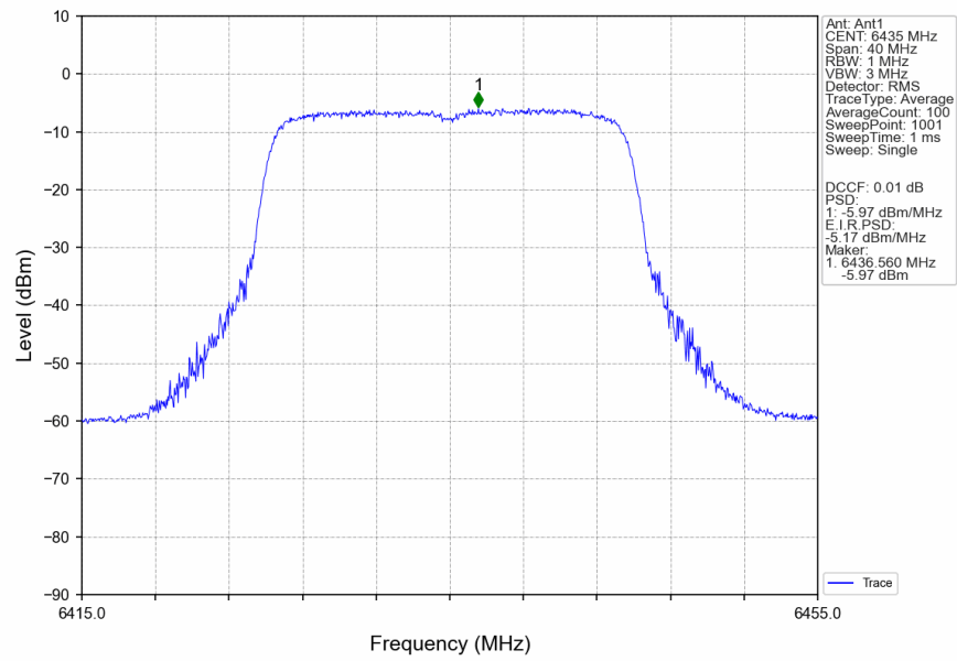
802.11ax(HEW20)_LCH_6435MHz_RU242_Left_MIMO_NTNV
