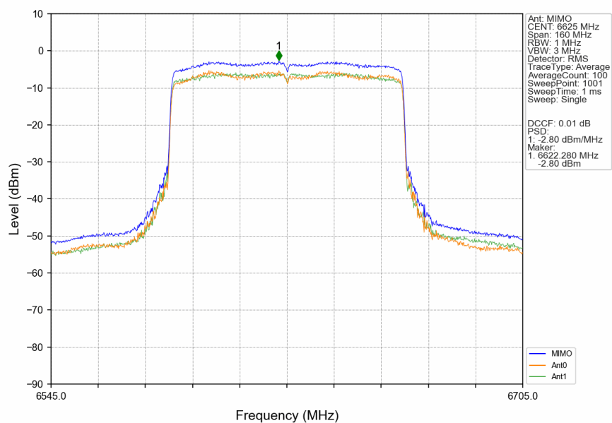
802.11ax(HEW80)_LCH_6625MHz_RU996_Left_MIMO_NTNV
