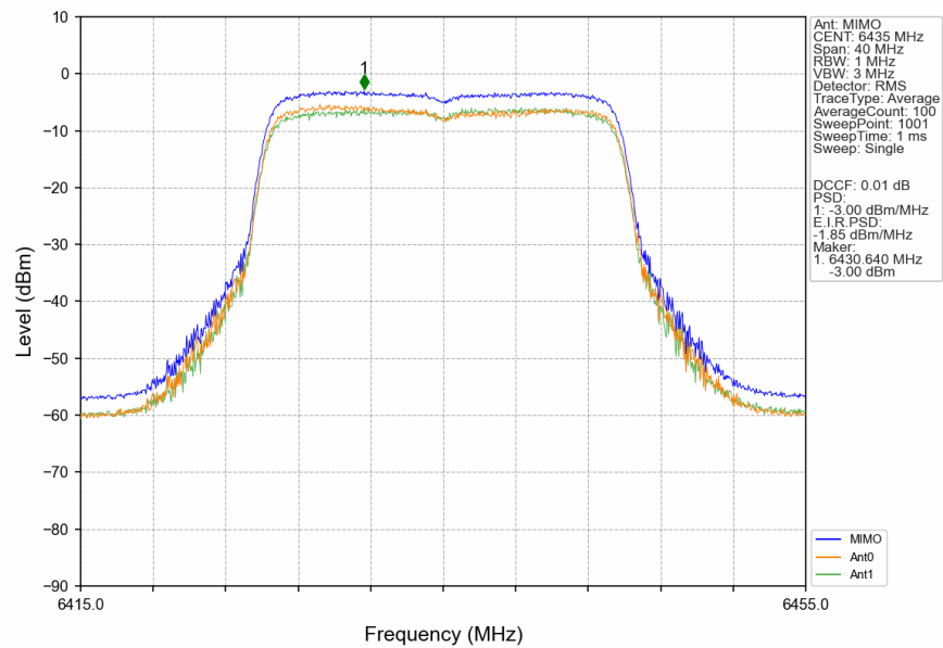
802.11ax(HEW20)_LCH_6435MHz_RU242_Left_MIMO_NTNV
