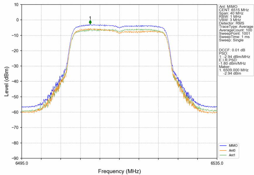
802.11ax(HEW20)_HCH_6515MHz_RU242_Left_MIMO_NTNV
