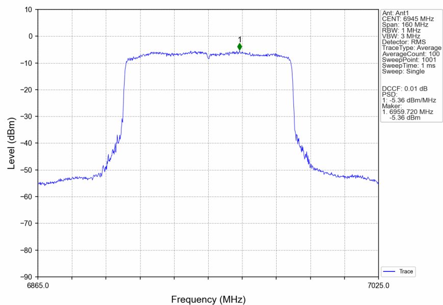
802.11ax(HEW80)_LCH_6945MHz_RU996_Left_MIMO_NTNV
