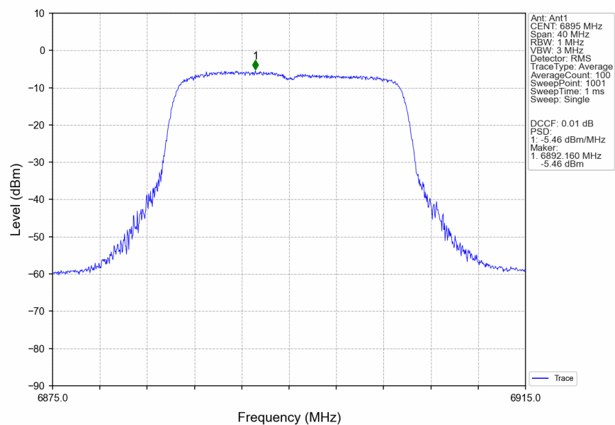
802.11ax(HEW20)_LCH_6895MHz_RU242_Left_MIMO_NTNV
