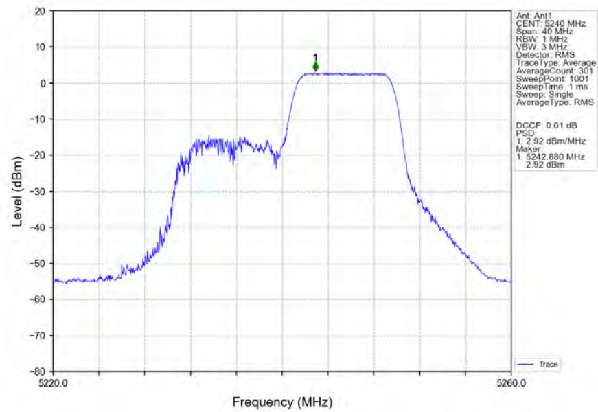
802.11be(EHT20)_HCH_5240MHz_RU106_Right_Ant1_NTN
