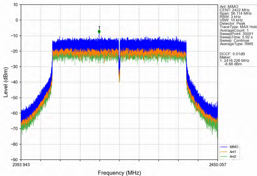
802.11ax(HEW40)_LCH_2422MHz_RU484_Left_MIMO_NTNV
