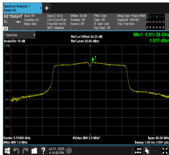
11N40MIMO-Ant7-5550-PASS
