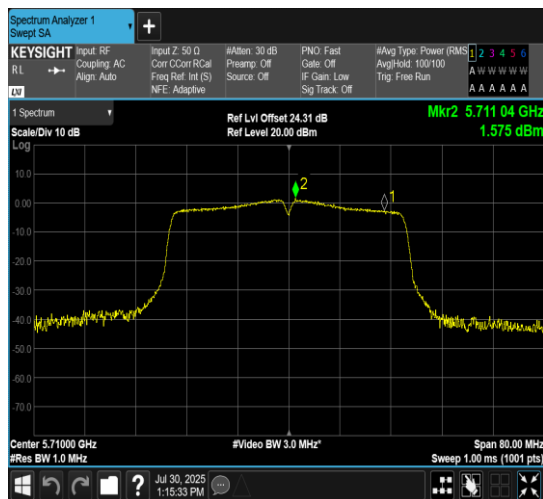
11N40MIMO-Ant10-5710_UNII-3-PASS
