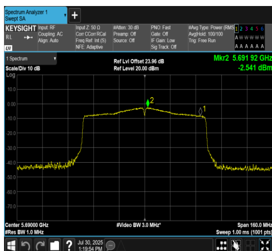
11AC80MIMO-Ant10-5690_UNII-3-PASS
