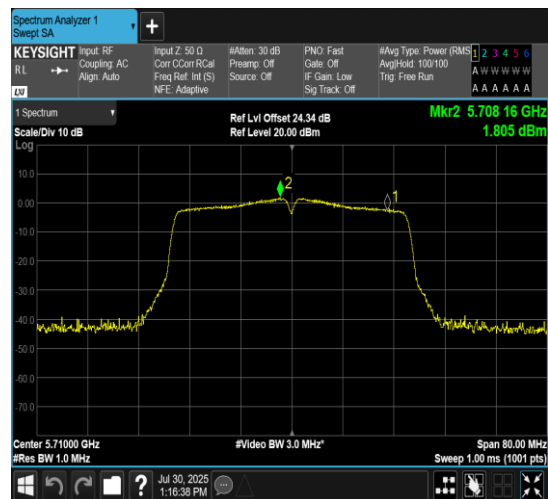
11N40MIMO-Ant7-5710_UNII-3-PASS
