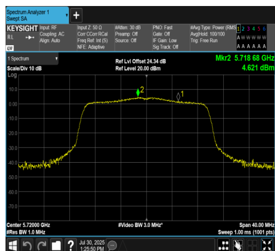
11AX20MIMO-Ant7-5720_UNII-3-PASS
