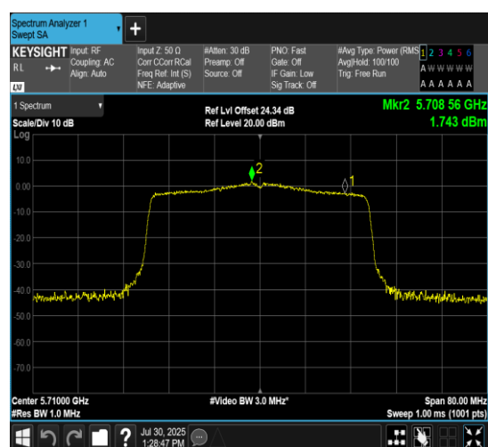
11AX40MIMO-Ant7-5710 UNII-3-PASS
