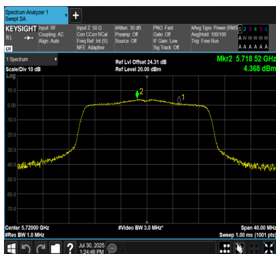
11AX20MIMO-Ant10-5720_UNII-3-PASS
