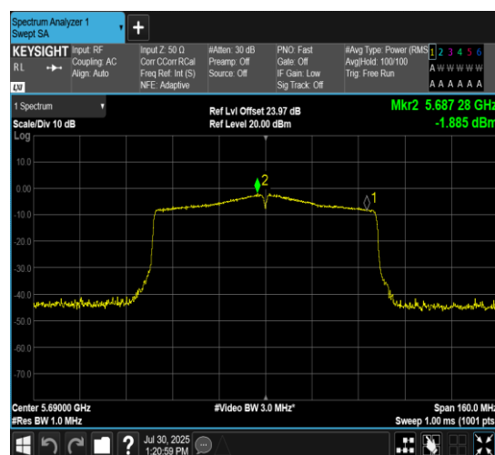
11AC80MIMO-Ant7-5690_UNII-3-PASS
