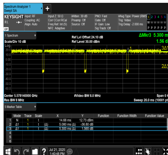
NTNV-11AX20MIMO-Ant7-5580-106Tone-RU53
