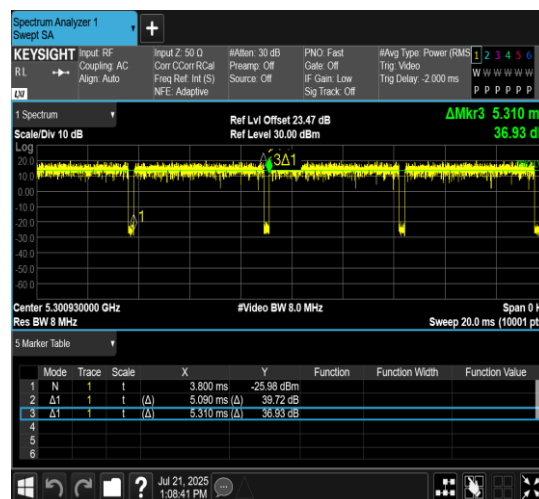
NTNV-11AX20MIMO-Ant7-5300-52Tone-RU38
