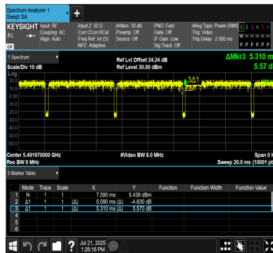
NTNV-11AX20MIMO-Ant7-5500-52Tone-RU37
