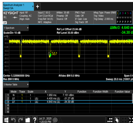
NTNV-11AX20MIMO-Ant7-5320-52Tone-RU40
