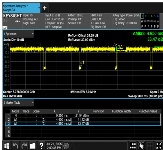
NTNV-11AX20MIMO-Ant10-5720-52Tone-RU40
