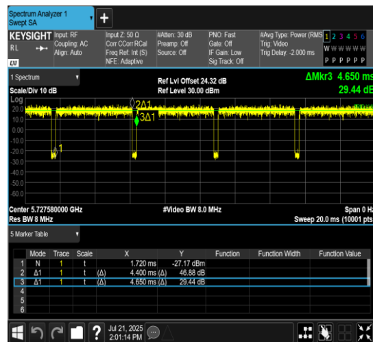
NTNV-11AX20MIMO-Ant7-5720-52Tone-RU40
