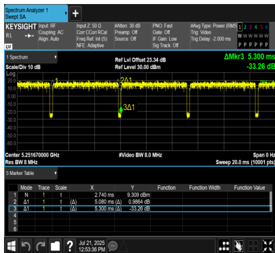
NTNV-11AX20MIMO-Ant10-5260-52Tone-RU37
