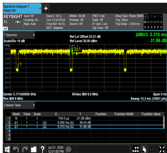
NTNV-11AX20MIMO-Ant7-5180-52Tone-RU37
