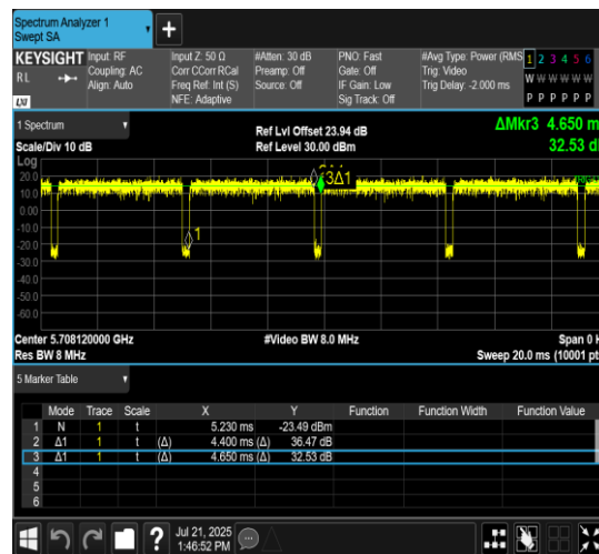
NTNV-11AX20MIMO-Ant7-5700-52Tone-RU40
