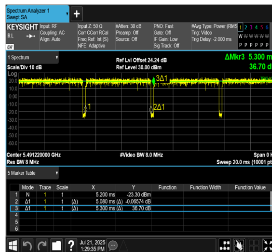
NTNV-11AX20MIMO-Ant7-5500-106Tone-RU53
