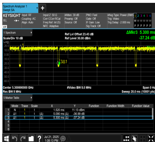
NTNV-11AX20MIMO-Ant10-5300-52Tone-RU38
