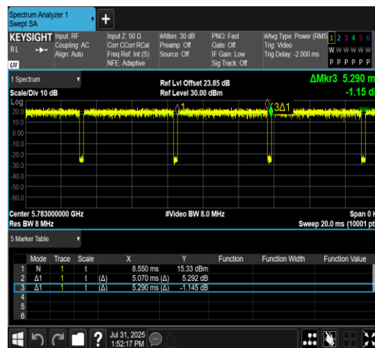
NTNV-11AX20MIMO-Ant7-5785-106Tone-RU53
