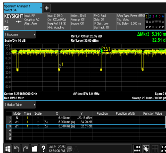
NTNV-11AX20MIMO-Ant7-5260-52Tone-RU37
