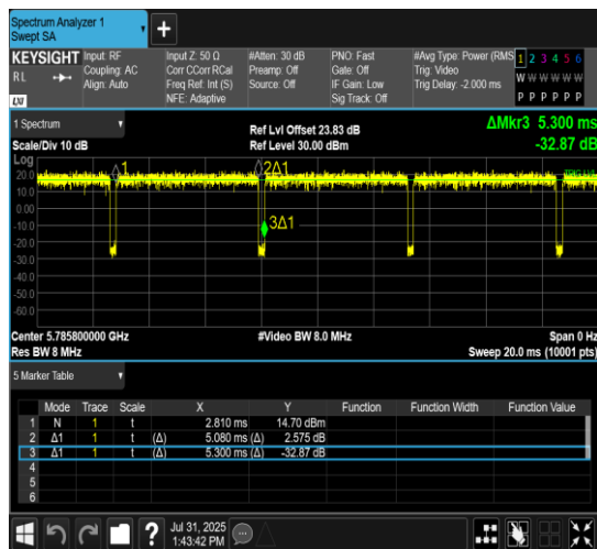
NTNV-11AX20MIMO-Ant10-5785-52Tone-RU38
