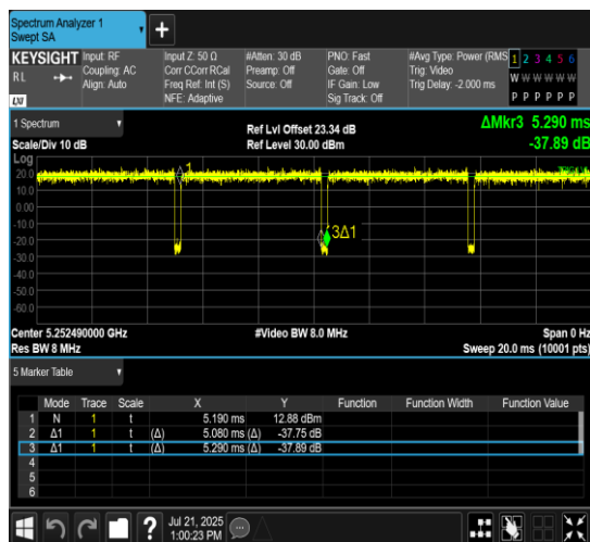
NTNV-11AX20MIMO-Ant10-5260-106Tone-RU53
