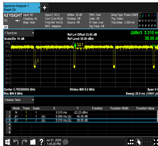
NTNV-11AX20MIMO-Ant7-5785-52Tone-RU38
