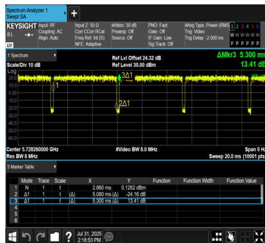
NTNV-11AX20MIMO-Ant7-5720-106Tone-RU54
