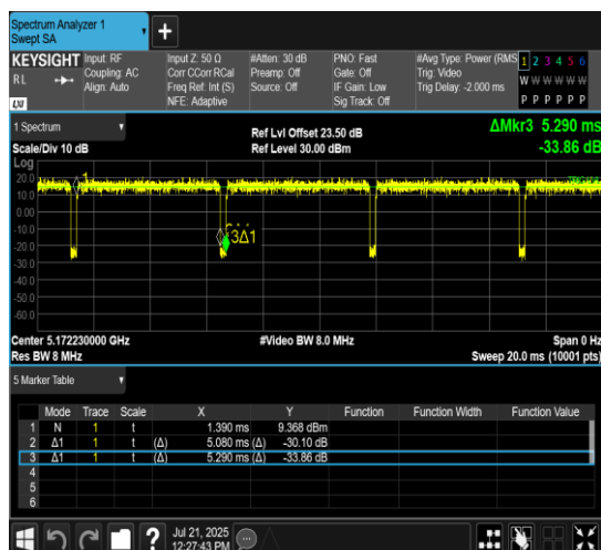
NTNV-11AX20MIMO-Ant10-5180-106Tone-RU53
