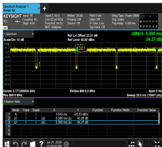
NTNV-11AX20MIMO-Ant7-5180-106Tone-RU53
