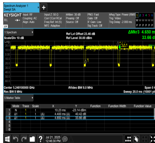
NTNV-11AX20MIMO-Ant7-5240-52Tone-RU40
