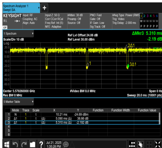
NTNV-11AX20MIMO-Ant10-5580-52Tone-RU38
