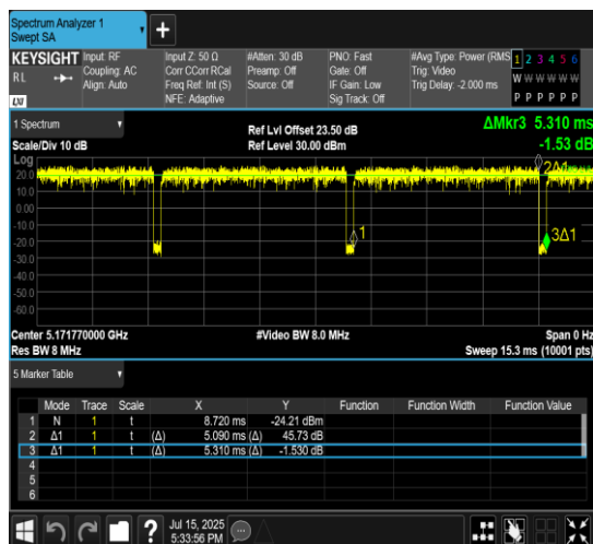
NTNV-11AX20MIMO-Ant10-5180-52Tone-RU37
