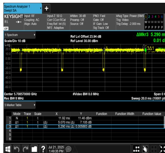
NTNV-11AX20MIMO-Ant7-5700-106Tone-RU54
