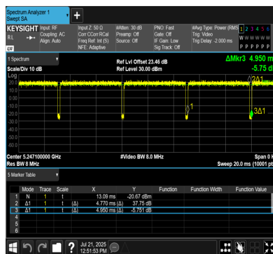
NTNV-11AX20MIMO-Ant7-5260-26Tone-RU0
