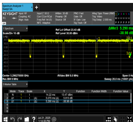
NTNV-11AX20MIMO-Ant10-5300-106Tone-RU53
