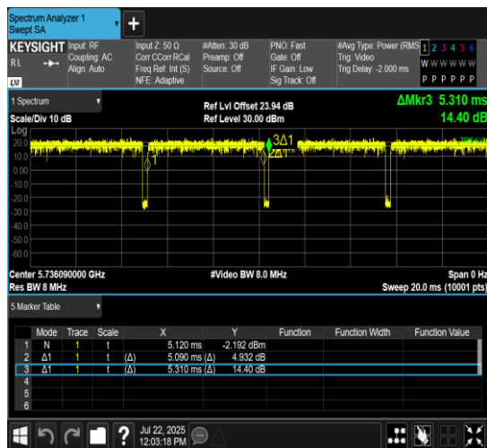
NTNV-11AX20MIMO-Ant10-5745-52Tone-RU37
