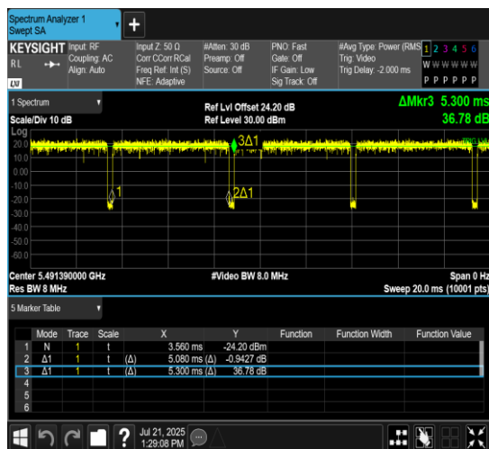
NTNV-11AX20MIMO-Ant10-5500-106Tone-RU53
