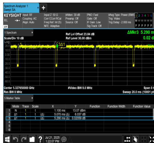
NTNV-11AX20MIMO-Ant7-5320-106Tone-RU54
