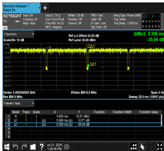
NTNV-11AX20MIMO-Ant10-5500-52Tone-RU37
