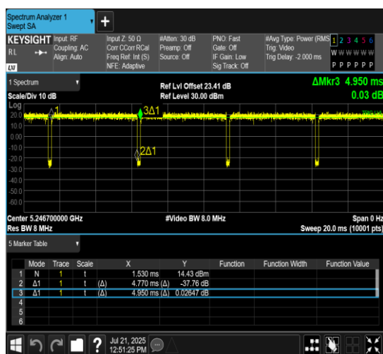
NTNV-11AX20MIMO-Ant10-5260-26Tone-RU0
