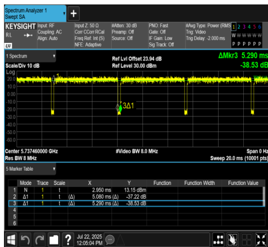
NTNV-11AX20MIMO-Ant10-5745-106Tone-RU53
