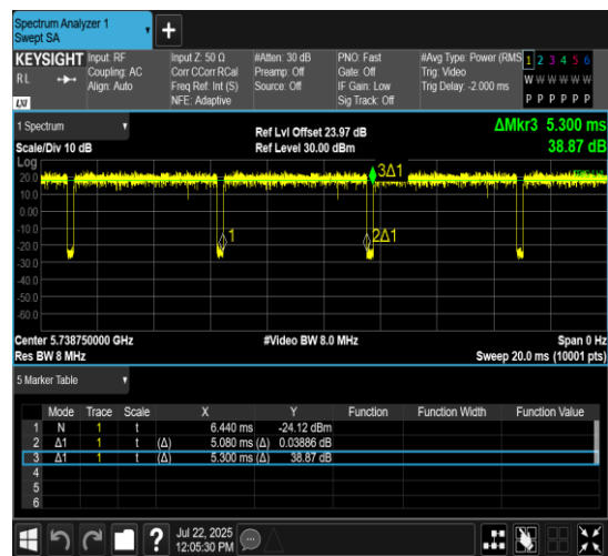
NTNV-11AX20MIMO-Ant7-5745-106Tone-RU53
