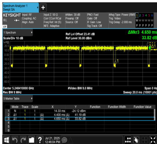
NTNV-11AX20MIMO-Ant10-5240-52Tone-RU40
