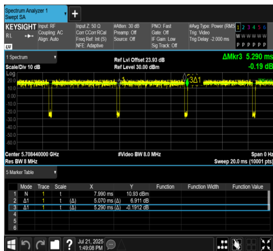
NTNV-11AX20MIMO-Ant10-5700-106Tone-RU54
