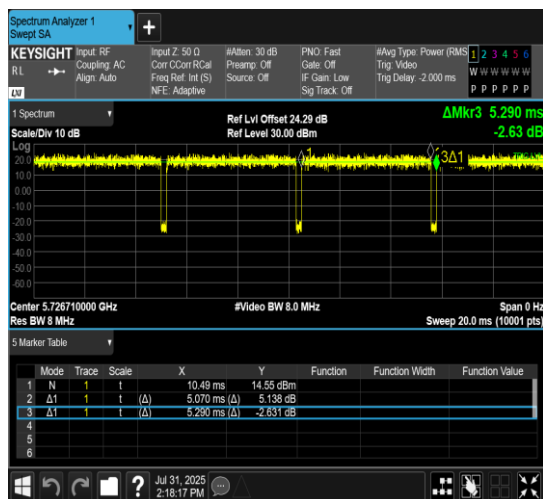
NTNV-11AX20MIMO-Ant10-5720-106Tone-RU54
