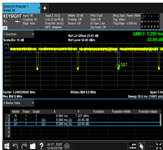
NTNV-11AX20MIMO-Ant10-5240-106Tone-RU54
