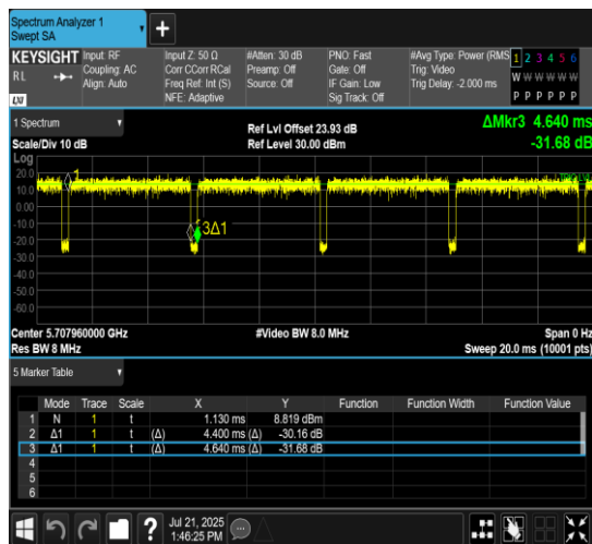
NTNV-11AX20MIMO-Ant10-5700-52Tone-RU40
