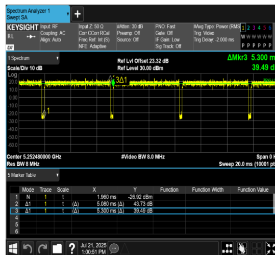
NTNV-11AX20MIMO-Ant7-5260-106Tone-RU53
