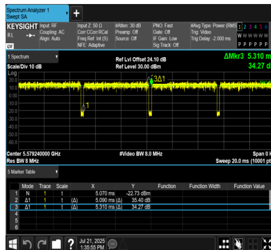
NTNV-11AX20MIMO-Ant7-5580-52Tone-RU38
