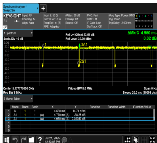
NTNV-11AX20MIMO-Ant7-5180-106Tone-RU53
