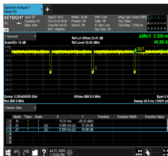
NTNV-11AX20MIMO-Ant7-5300-106Tone-RU53
