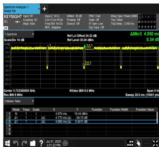
NTNV-11AX20MIMO-Ant7-5745-26Tone-RU0
