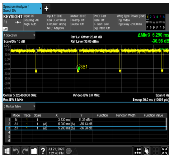
NTNV-11AX20MIMO-Ant10-5320-106Tone-RU54
