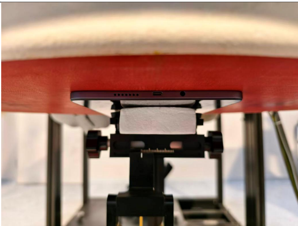
Body SAR Back Side 7mm
