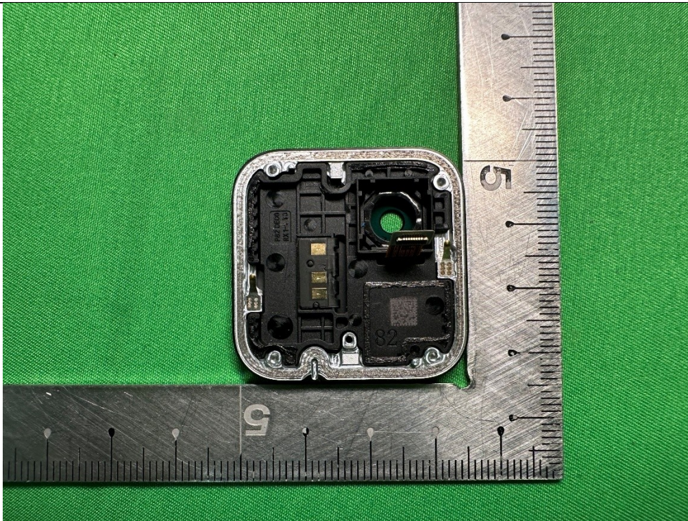
(18) EUT Photo Ant0: Wifi full band/Bluetooth antenna
