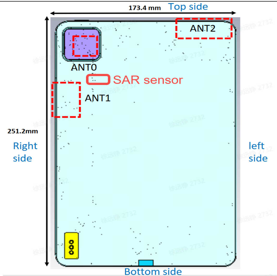
EUT Photo(DUT Antenna Locations)
