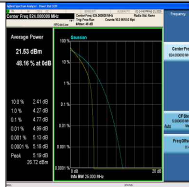
Band26(814-824)-1.4MHz-64QAM-26790-6RB#0-PASS
