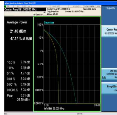
Band26(814-824)-5MHz-64QAM-26765-25RB#0-PASS
