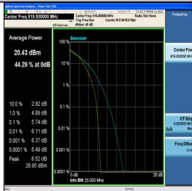
Band26(814-824)-5MHz-16QAM-26740-25RB#0-PASS
