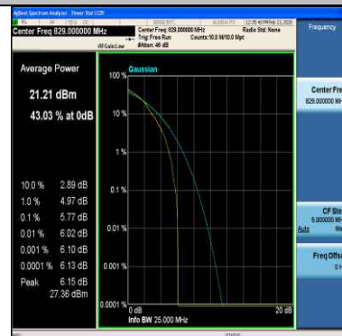
Band5-10MHz-16QAM-20450-1RB#0-PASS
