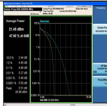
Band26(824-849)-1.4MHz-64QAM-26915-6RB#0-PASS
