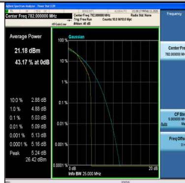
Band13-10MHz-QPSK-23230-50RB#0-PASS
