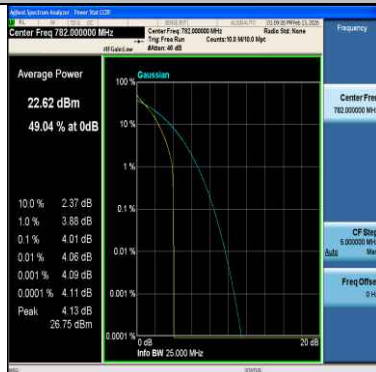
Band13-10MHz-64QAM-23230-1RB#0-PASS
