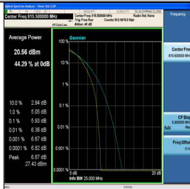
Band26(814-824)-3MHz-16QAM-26705-15RB#0-PASS
