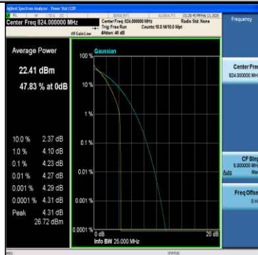
Band26(814-824)-15MHz-64QAM-26790-1RB#0-PASS
