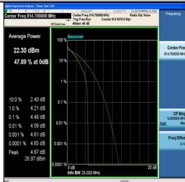
Band26(814-824)-1.4MHz-64QAM-26697-1RB#0-PASS
