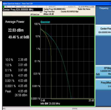
Band26(814-824)-3MHz-64QAM-26790-1RB#0-PASS
