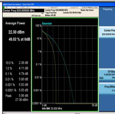
Band5-10MHz-QPSK-20450-1RB#0-PASS
