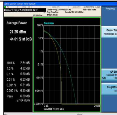
Band7-15MHz-QPSK-21100-75RB#0-PASS
