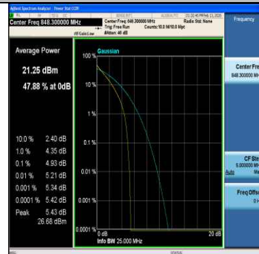
Band26(824-849)-1.4MHz-64QAM-27033-6RB#0-PASS
