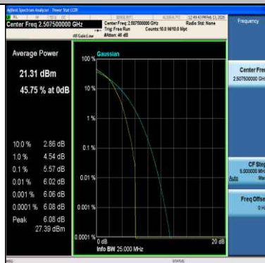
Band7-15MHz-64QAM-20825-1RB#0-PASS
