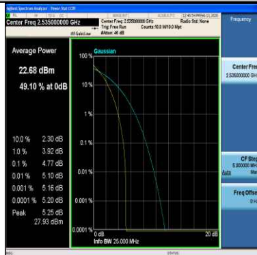
Band7-10MHz-64QAM-21100-1RB#0-PASS
