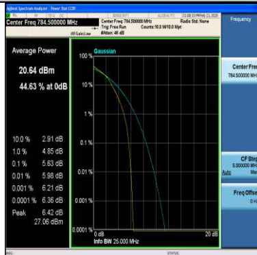
Band13-10MHz-QPSK-23230-1RB#0-PASS
