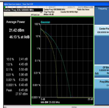
Band5-10MHz-QPSK-20525-50RB#0-PASS
