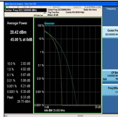
Band26(814-824)-3MHz-64QAM-26775-15RB#0-PASS
