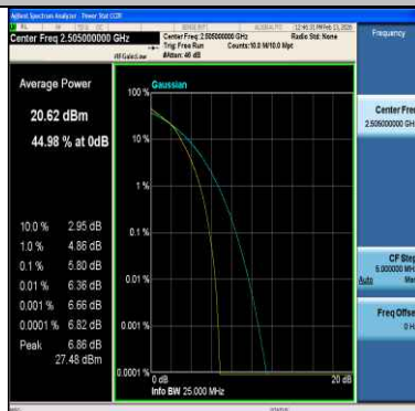
Band7-10MHz-16QAM-20800-50RB#0-PASS
