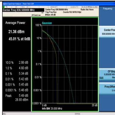
Band26(824-849)-1.4MHz-16QAM-26915-6RB#0-PASS
