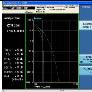
Band26(814-824)-5MHz-64QAM-26740-1RB#0-PASS
