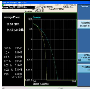
Band26(814-824)-5MHz-16QAM-26765-25RB#0-PASS
