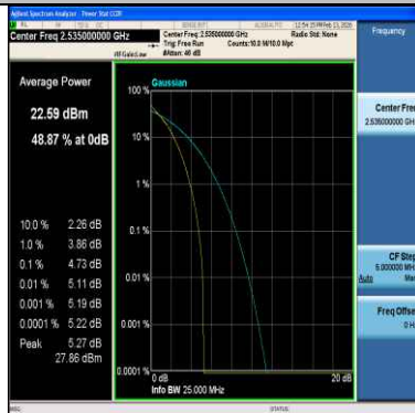
Band7-20MHz-64QAM-21100-1RB#0-PASS
