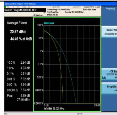
Band26(814-824)-10MHz-64QAM-26740-50RB#0-PASS
