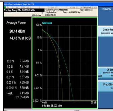
Band5-10MHz-64QAM-20600-50RB#0-PASS
