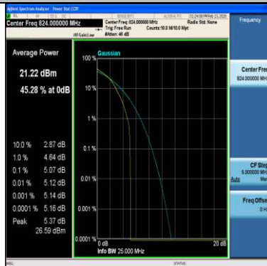
Band26(814-824)-5MHz-16QAM-26790-25RB#0-PASS
