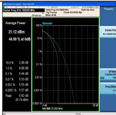
Band26(814-824)-1.4MHz-16QAM-26697-6RB#0-PASS
