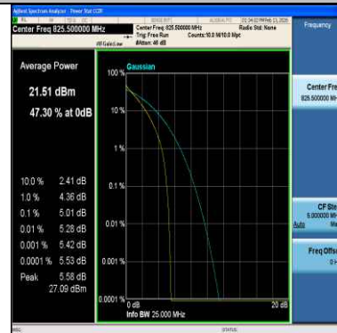
Band26(824-849)-3MHz-64QAM-26805-15RB#0-PASS
