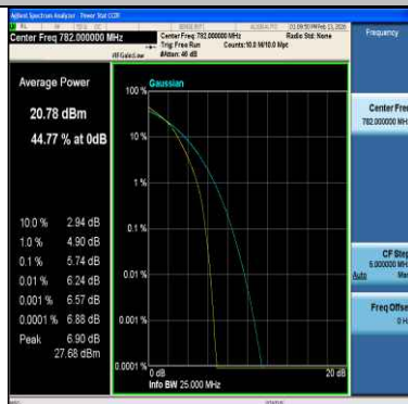
Band13-10MHz-16QAM-23230-50RB#0-PASS
