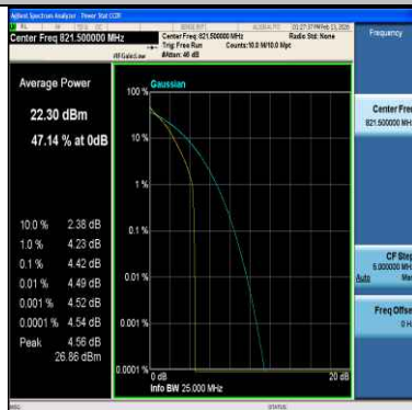
Band26(814-824)-15MHz-64QAM-26765-1RB#0-PASS
