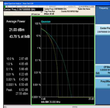
Band7-5MHz-QPSK-21425-25RB#0-PASS
