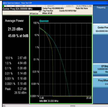
Band26(814-824)-3MHz-16QAM-26790-15RB#0-PASS
