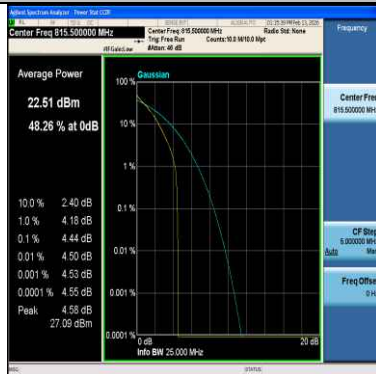
Band26(814-824)-3MHz-64QAM-26705-1RB#0-PASS
