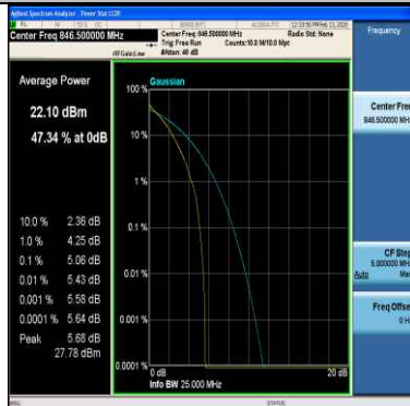
Band5-5MHz-64QAM-20625-1RB#0-PASS
