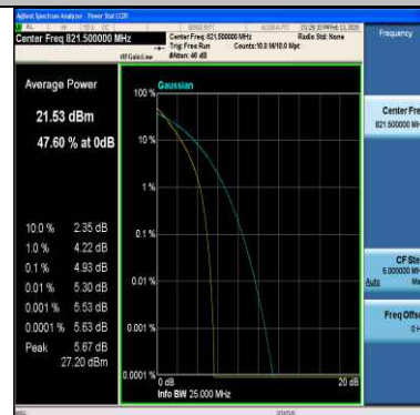
Band26(814-824)-15MHz-64QAM-26765-75RB#0-PASS
