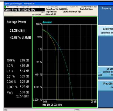
Band13-5MHz-QPSK-23255-25RB#0-PASS
