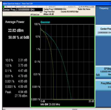
Band7-10MHz-64QAM-20800-1RB#0-PASS
