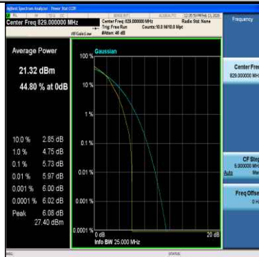
Band5-10MHz-16QAM-20450-50RB#0-PASS
