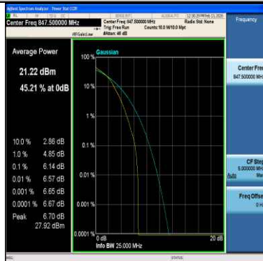
Band5-3MHz-16QAM-20635-15RB#0-PASS
