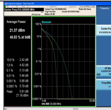
Band26(814-824)-3MHz-64QAM-26705-15RB#0-PASS
