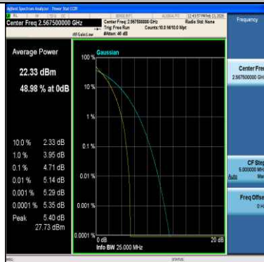
Band7-5MHz-64QAM-21425-1RB#0-PASS
