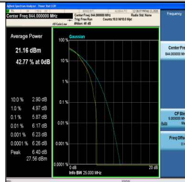
Band5-10MHz-QPSK-20600-50RB#0-PASS
