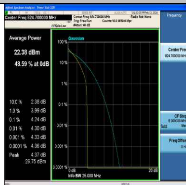
Band26(824-849)-1.4MHz-64QAM-26797-1RB#0-PASS
