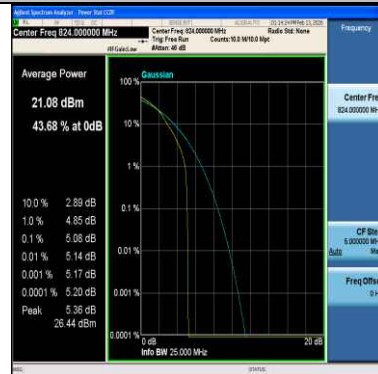
Band26(814-824)-1.4MHz-QPSK-26790-6RB#0-PASS
