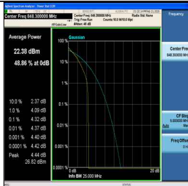
Band26(824-849)-1.4MHz-64QAM-27033-1RB#0-PASS
