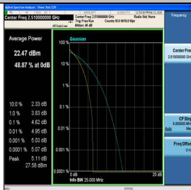
Band7-20MHz-QPSK-20850-1RB#0-PASS
