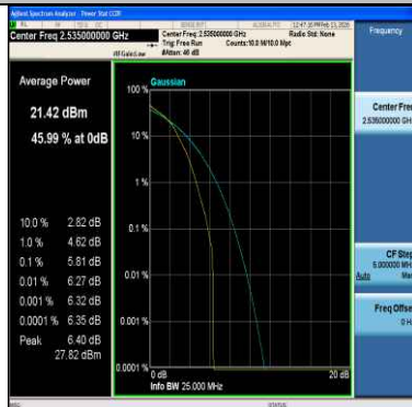
Band7-10MHz-16QAM-21100-50RB#0-PASS
