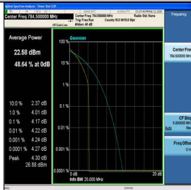
Band13-5MHz-64QAM-23255-1RB#0-PASS
