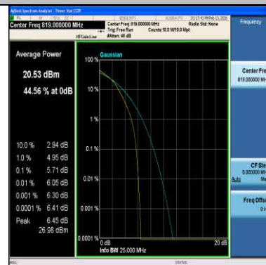
Band26(814-824)-3MHz-64QAM-26740-15RB#0-PASS
