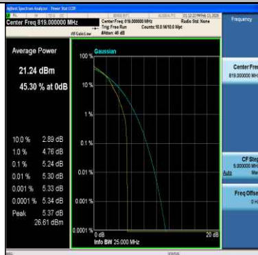
Band26(814-824)-1.4MHz-16QAM-26740-6RB#0-PASS
