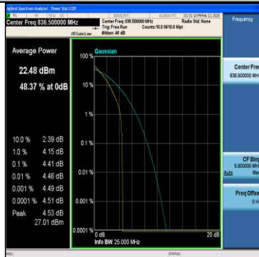
Band26(824-849)-1.4MHz-64QAM-26915-1RB#0-PASS
