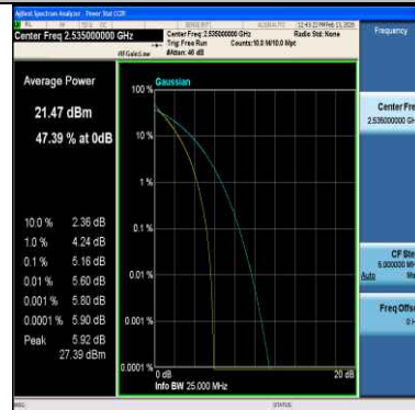
Band7-5MHz-64QAM-21100-25RB#0-PASS
