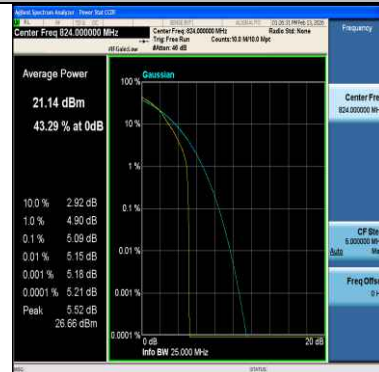
Band26(814-824)-10MHz-QPSK-26790-50RB#0-PASS
