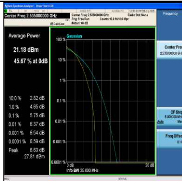
Band7-5MHz-16QAM-21100-25RB#0-PASS
