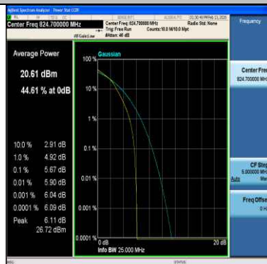
Band26(824-849)-1.4MHz-16QAM-26797-6RB#0-PASS
