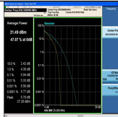
Band26(824-849)-3MHz-64QAM-26915-15RB#0-PASS
