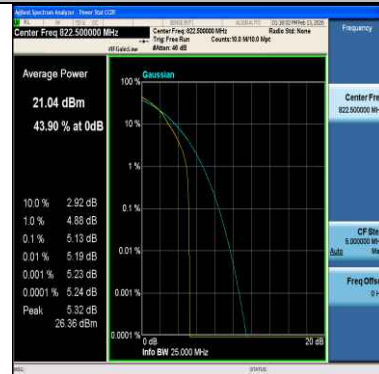
Band26(814-824)-3MHz-QPSK-26775-15RB#0-PASS
