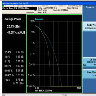
Band26(814-824)-5MHz-16QAM-26715-25RB#0-PASS
