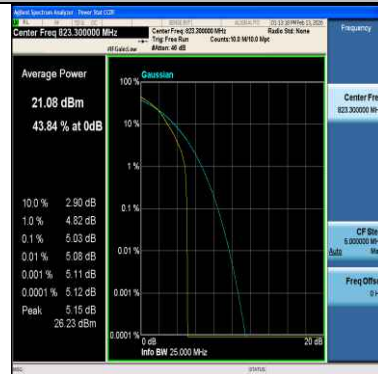
Band26(814-824)-1.4MHz-QPSK-26783-6RB#0-PASS
