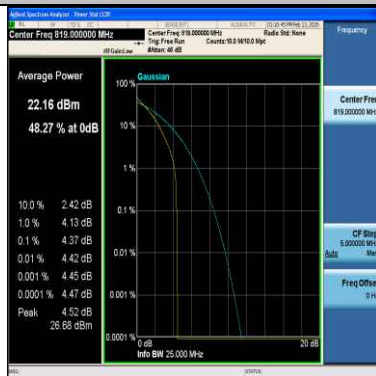
Band26(814-824)-3MHz-64QAM-26740-1RB#0-PASS
