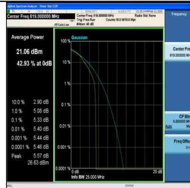
Band26(814-824)-10MHz-QPSK-26740-50RB#0-PASS
