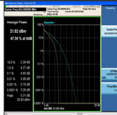
Band26(814-824)-3MHz-64QAM-26790-15RB#0-PASS
