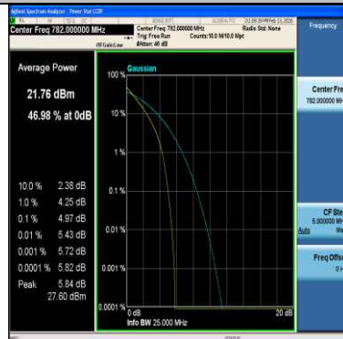
Band13-10MHz-64QAM-23230-50RB#0-PASS
