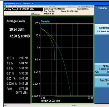
Band26(814-824)-5MHz-QPSK-26715-25RB#0-PASS
