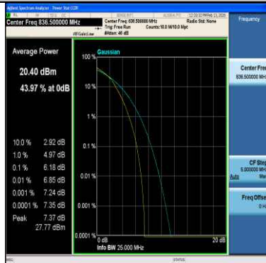
Band5-5MHz-16QAM-20525-25RB#0-PASS
