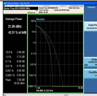
Band5-5MHz-QPSK-20525-25RB#0-PASS
