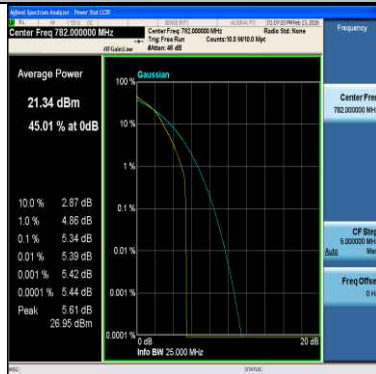
Band13-5MHz-16QAM-23230-25RB#0-PASS
