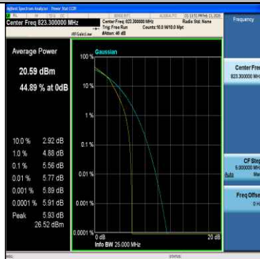
Band26(814-824)-1.4MHz-16QAM-26783-6RB#0-PASS
