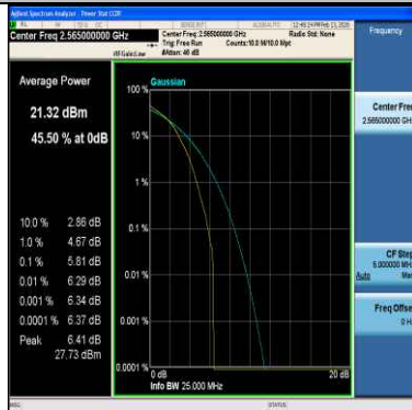
Band7-10MHz-16QAM-21400-50RB#0-PASS
