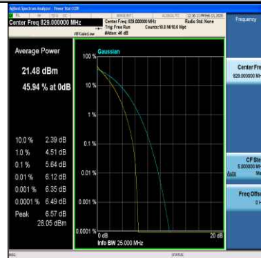
Band5-10MHz-64QAM-20450-50RB#0-PASS
