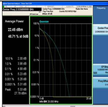
Band7-15MHz-64QAM-21100-1RB#0-PASS
