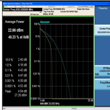
Band26(824-849)-3MHz-64QAM-26915-1RB#0-PASS
