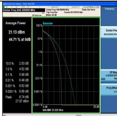
Band5-5MHz-16QAM-20625-25RB#0-PASS
