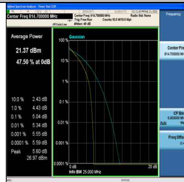
Band26(814-824)-1.4MHz-64QAM-26697-6RB#0-PASS
