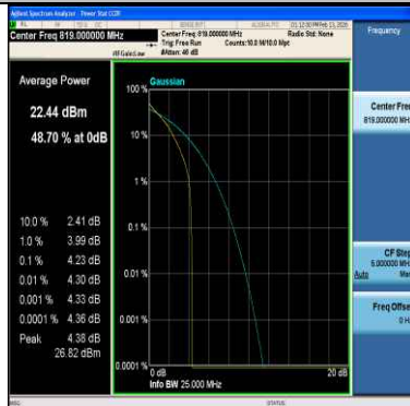
Band26(814-824)-1.4MHz-64QAM-26740-1RB#0-PASS
