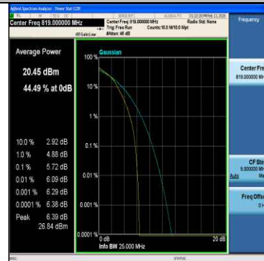
Band26(814-824)-5MHz-64QAM-26740-25RB#0-PASS
