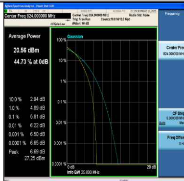
Band26(814-824)-15MHz-16QAM-26790-75RB#0-PASS
