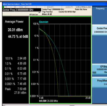
Band7-20MHz-16QAM-21350-100RB#0-PASS
