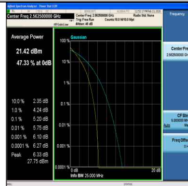
Band7-15MHz-64QAM-21375-75RB#0-PASS
