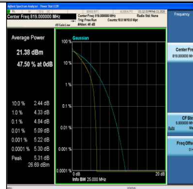
Band26(814-824)-1.4MHz-64QAM-26740-6RB#0-PASS
