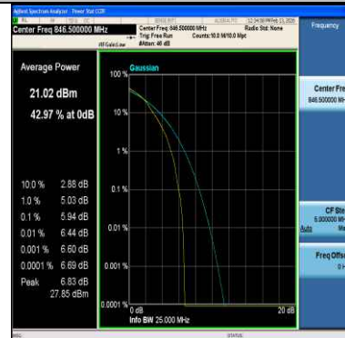
Band5-5MHz-QPSK-20625-25RB#0-PASS
