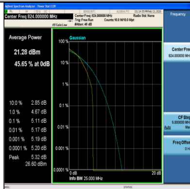
Band26(814-824)-1.4MHz-16QAM-26790-6RB#0-PASS
