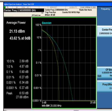
Band7-10MHz-16QAM-21400-1RB#0-PASS
