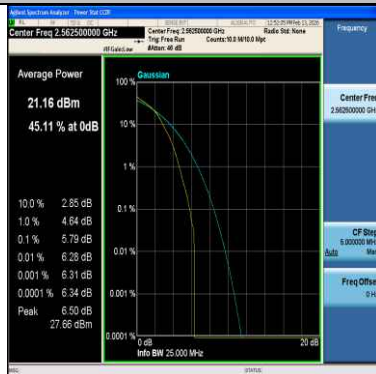
Band7-15MHz-16QAM-21375-75RB#0-PASS
