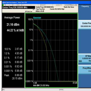
Band5-5MHz-16QAM-20525-25RB#0-PASS
