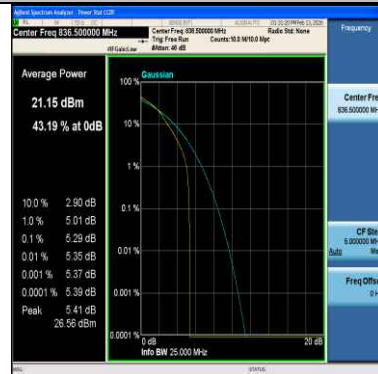
Band26(824-849)-1.4MHz-QPSK-26915-6RB#0-PASS
