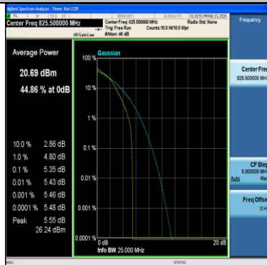
Band26(824-849)-3MHz-16QAM-26805-15RB#0-PASS
