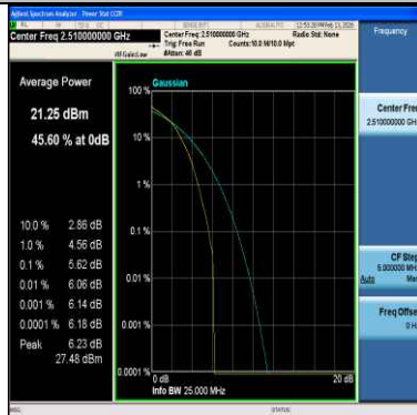
Band7-20MHz-16QAM-20850-100RB#0-PASS
