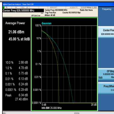
Band5-5MHz-64QAM-20425-1RB#0-PASS
