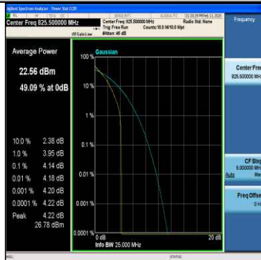
Band26(824-849)-3MHz-64QAM-26805-1RB#0-PASS
