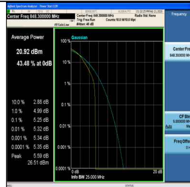
Band26(824-849)-1.4MHz-QPSK-27033-6RB#0-PASS
