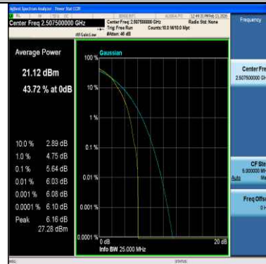
Band7-15MHz-QPSK-20825-75RB#0-PASS
