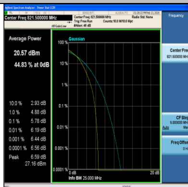
Band26(814-824)-15MHz-16QAM-26765-75RB#0-PASS
