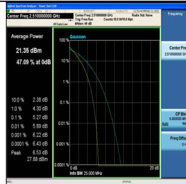
Band7-20MHz-64QAM-20850-100RB#0-PASS
