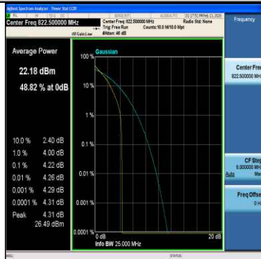
Band26(814-824)-3MHz-64QAM-26775-1RB#0-PASS
