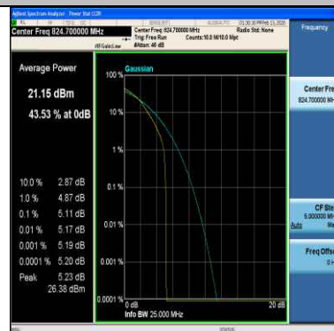
Band26(824-849)-1.4MHz-QPSK-26797-6RB#0-PASS
