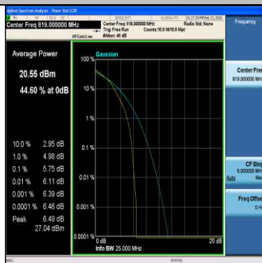
Band26(814-824)-3MHz-16QAM-26740-15RB#0-PASS
