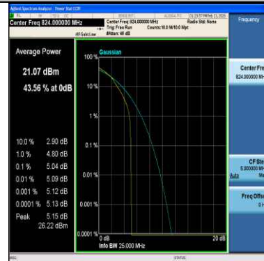
Band26(814-824)-5MHz-QPSK-26790-25RB#0-PASS
