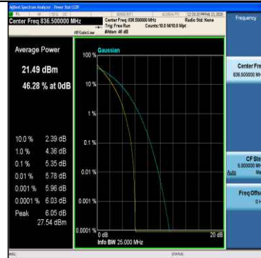
Band5-5MHz-64QAM-20525-25RB#0-PASS
