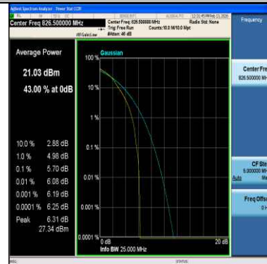
Band5-5MHz-QPSK-20425-25RB#0-PASS
