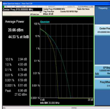
Band26(814-824)-10MHz-16QAM-26740-50RB#0-PASS
