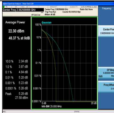
Band7-15MHz-64QAM-21375-1RB#0-PASS
