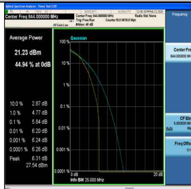
Band5-10MHz-16QAM-20600-50RB#0-PASS
