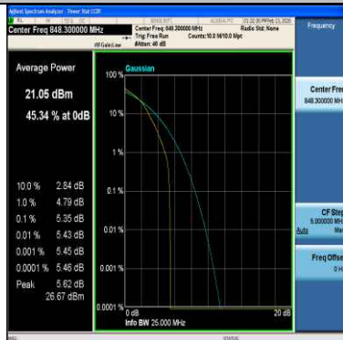
Band26(824-849)-1.4MHz-16QAM-27033-6RB#0-PASS
