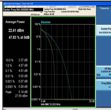
Band5-10MHz-64QAM-20600-1RB#0-PASS
