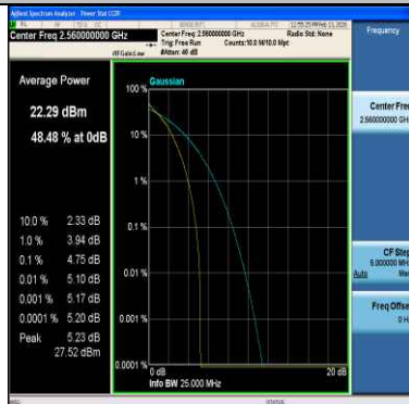
Band7-20MHz-64QAM-21350-1RB#0-PASS
