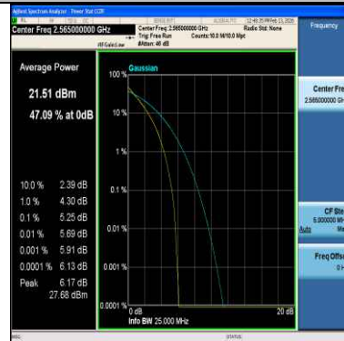
Band7-10MHz-64QAM-21400-50RB#0-PASS
