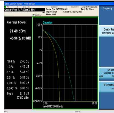
Band5-3MHz-64QAM-20635-15RB#0-PASS
