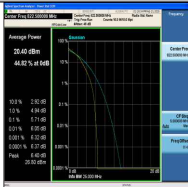
Band26(814-824)-3MHz-16QAM-26775-15RB#0-PASS
