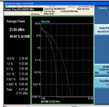
Band5-5MHz-64QAM-20625-25RB#0-PASS
