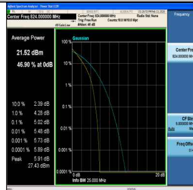
Band26(814-824)-10MHz-64QAM-26790-50RB#0-PASS
