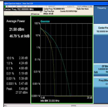
Band13-5MHz-64QAM-23230-25RB#0-PASS
