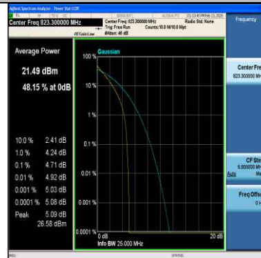
Band26(814-824)-1.4MHz-64QAM-26783-6RB#0-PASS
