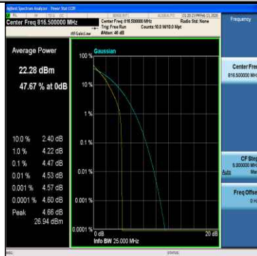
Band26(814-824)-5MHz-64QAM-26715-1RB#0-PASS
