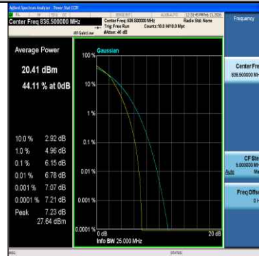
Band5-5MHz-64QAM-20525-25RB#0-PASS
