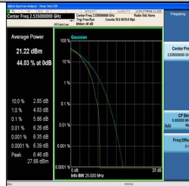
Band7-20MHz-QPSK-21100-100RB#0-PASS
