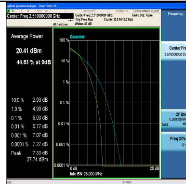
Band7-20MHz-16QAM-21100-1RB#0-PASS
