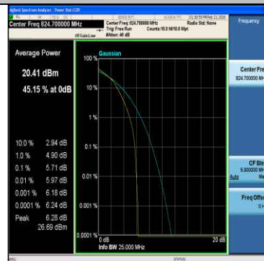
Band26(824-849)-1.4MHz-64QAM-26797-6RB#0-PASS
