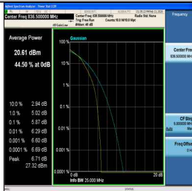
Band26(824-849)-3MHz-16QAM-26915-15RB#0-PASS
