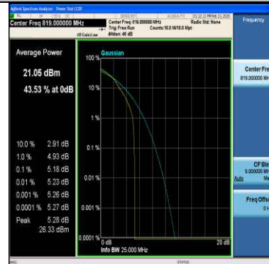
Band26(814-824)-1.4MHz-QPSK-26740-6RB#0-PASS
