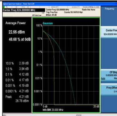
Band26(814-824)-10MHz-64QAM-26790-1RB#0-PASS
