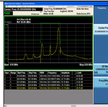
Band26(814-824)-3MHz-64QAM-26775-1RB#14-PASS
