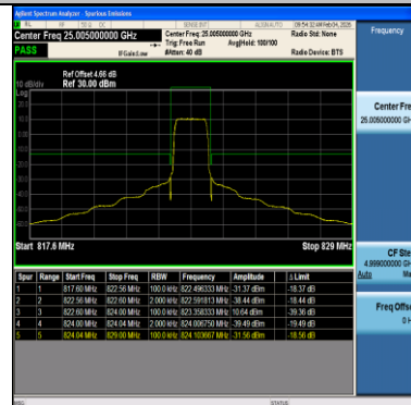
Band26(814-824)-1.4MHz-64QAM-26783-6RB#0-PASS
