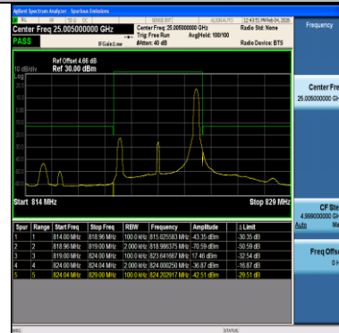
Band26(814-824)-5MHz-QPSK-26765-25RB#0-PASS
