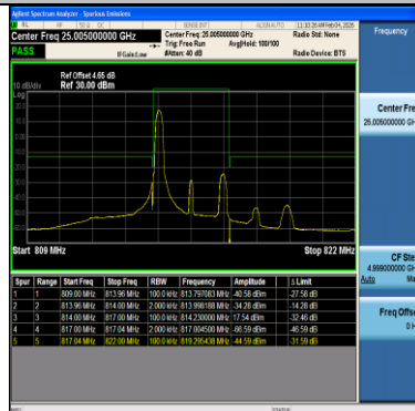
Band26(814-824)-3MHz-16QAM-26705-1RB#0-PASS
