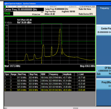
Band26(814-824)-3MHz-QPSK-26790-15RB#0-PASS
