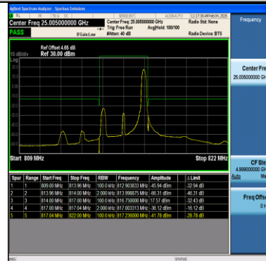
Band26(814-824)-3MHz-QPSK-26705-15RB#0-PASS
