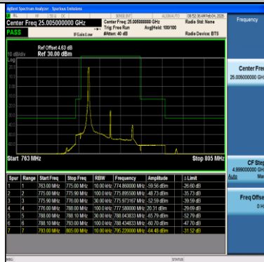
Band13-10MHz-64QAM-23230-1RB#0-PASS
