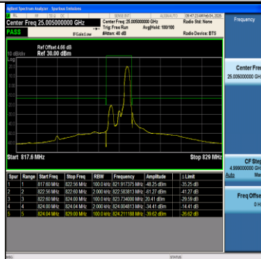
Band26(814-824)-1.4MHz-64QAM-26783-1RB#5-PASS
