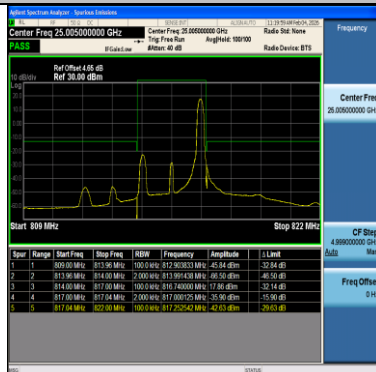
Band26(814-824)-3MHz-16QAM-26705-15RB#0-PASS
