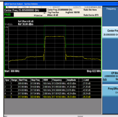
Band26(814-824)-3MHz-64QAM-26705-15RB#0-PASS
