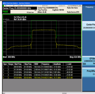
Band26(814-824)-5MHz-64QAM-26715-25RB#0-PASS
