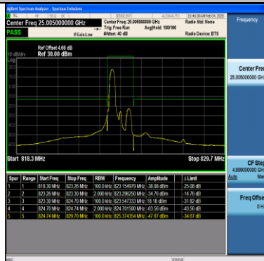
Band26(814-824)-1.4MHz-16QAM-26790-1RB#5-PASS
