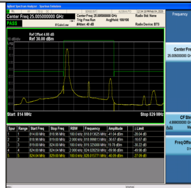
Band26(814-824)-5MHz-64QAM-26765-1RB#0-PASS
