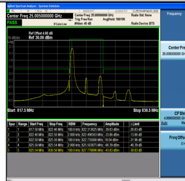
Band26(814-824)-3MHz-64QAM-26790-1RB#0-PASS
