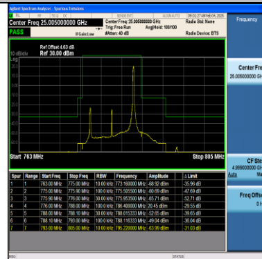
Band13-10MHz-64QAM-23230-1RB#49-PASS
