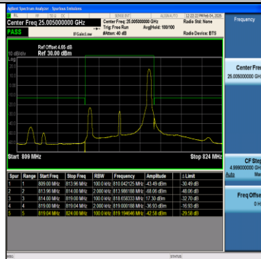
Band26(814-824)-5MHz-16QAM-26715-1RB#24-PASS
