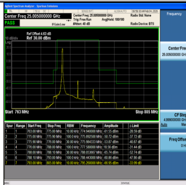
Band13-10MHz-16QAM-23230-1RB#49-PASS
