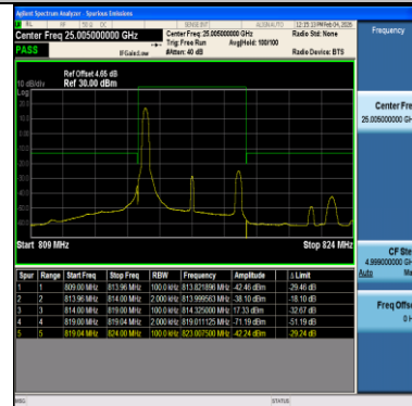
Band26(814-824)-5MHz-QPSK-26715-1RB#24-PASS
