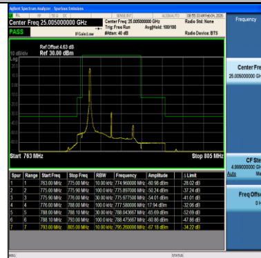
Band13-10MHz-QPSK-23230-1RB#49-PASS
