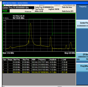
Band26(814-824)-5MHz-16QAM-26765-1RB#0-PASS
