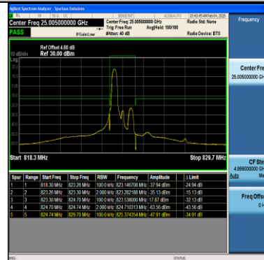
Band26(814-824)-1.4MHz-QPSK-26790-1RB#5-PASS
