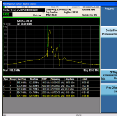
Band26(814-824)-1.4MHz-64QAM-26790-1RB#0-PASS
