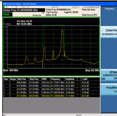
Band26(814-824)-3MHz-64QAM-26705-1RB#14-PASS
