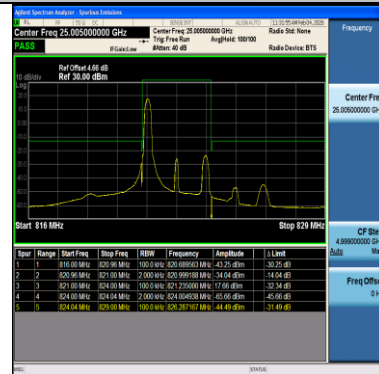
Band26(814-824)-3MHz-QPSK-26775-1RB#14-PASS
