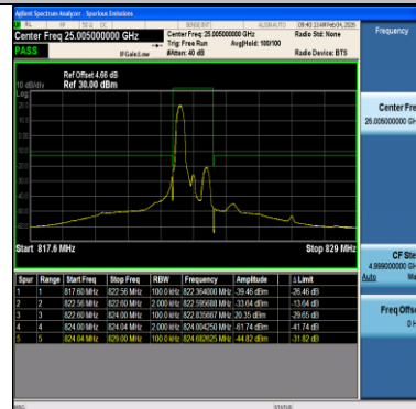
Band26(814-824)-1.4MHz-64QAM-26783-1RB#0-PASS
