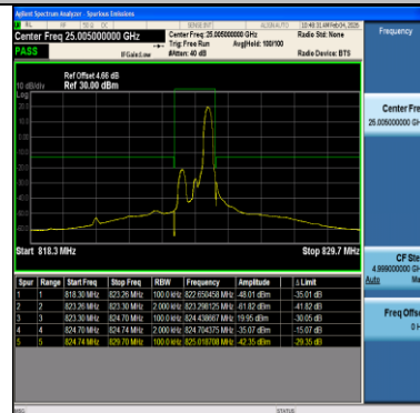
Band26(814-824)-1.4MHz-64QAM-26790-1RB#5-PASS
