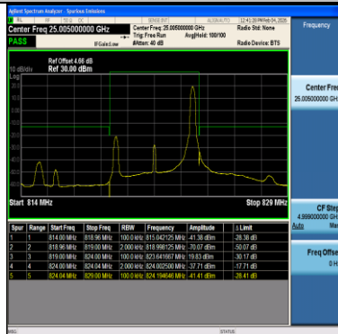
Band26(814-824)-5MHz-64QAM-26765-1RB#24-PASS
