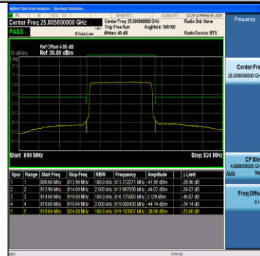
Band26(814-824)-5MHz-QPSK-26765-1RB#0-PASS
