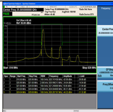
Band26(814-824)-3MHz-16QAM-26775-1RB#14-PASS
