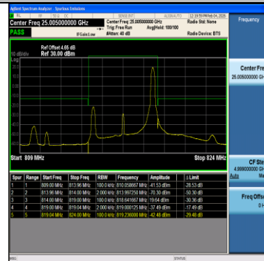
Band26(814-824)-5MHz-64QAM-26715-1RB#24-PASS
