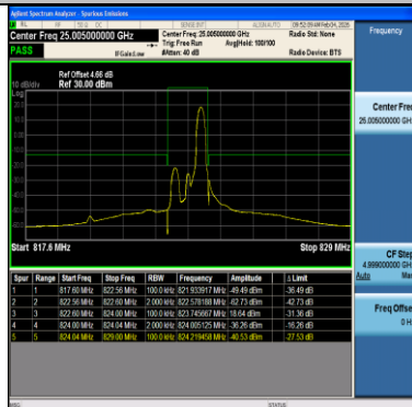
Band26(814-824)-1.4MHz-16QAM-26783-6RB#0-PASS
