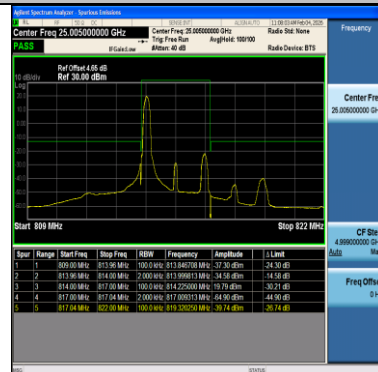
Band26(814-824)-3MHz-64QAM-26705-1RB#0-PASS
