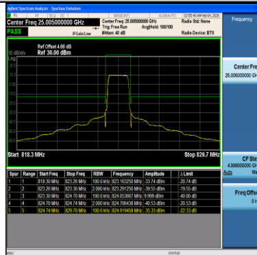
Band26(814-824)-1.4MHz-64QAM-26790-6RB#0-PASS
