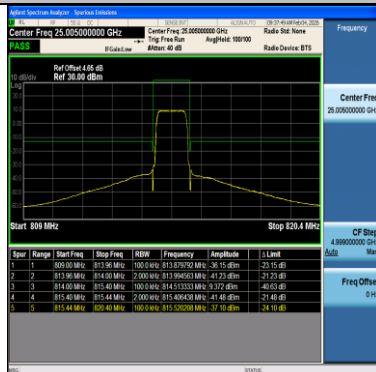
Band26(814-824)-1.4MHz-16QAM-26783-1RB#0-PASS
