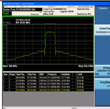
Band26(814-824)-1.4MHz-64QAM-26697-6RB#0-PASS
