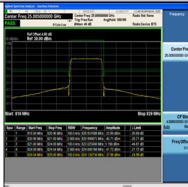
Band26(814-824)-3MHz-16QAM-26790-1RB#0-PASS
