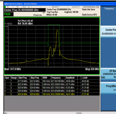
Band26(814-824)-1.4MHz-QPSK-26783-6RB#0-PASS
