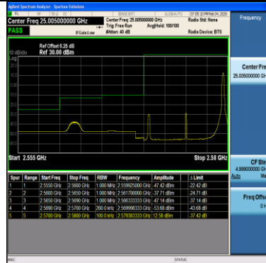
Band38-10MHz-64QAM-37800-1RB#49-PASS
