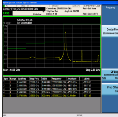
Band38-10MHz-16QAM-37800-1RB#49-PASS
