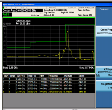
Band38-5MHz-64QAM-37775-1RB#0-PASS
