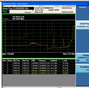
Band38-5MHz-QPSK-37775-25RB#0-PASS
