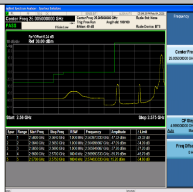
Band38-5MHz-64QAM-37775-1RB#24-PASS
