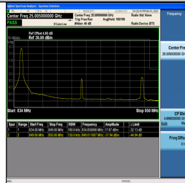
Band26(824-849)-15MHz-64QAM-26965-1RB#0-PASS
