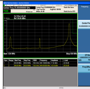
Band26(824-849)-15MHz-QPSK-26965-75RB#0-PASS
