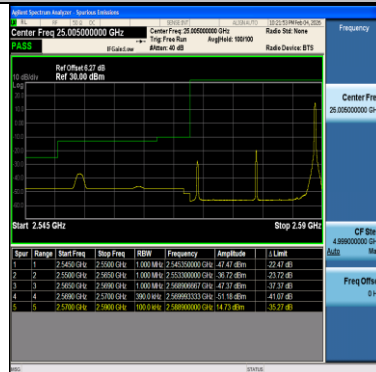
Band38-20MHz-64QAM-37850-1RB#99-PASS
