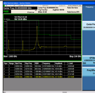
Band38-15MHz-QPSK-38175-75RB#0-PASS
