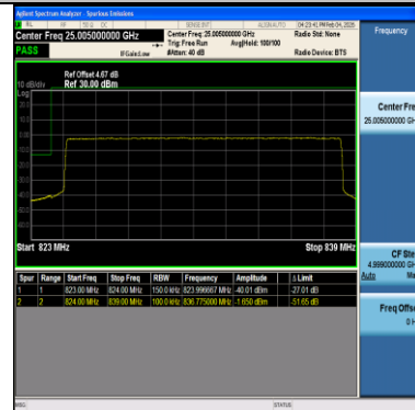
Band26(824-849)-15MHz-QPSK-26965-1RB#0-PASS
