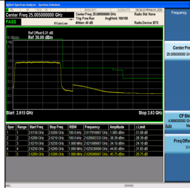
Band38-10MHz-16QAM-37800-1RB#0-PASS
