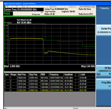
Band38-15MHz-64QAM-38175-75RB#0-PASS
