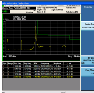
Band38-15MHz-64QAM-38175-1RB#74-PASS
