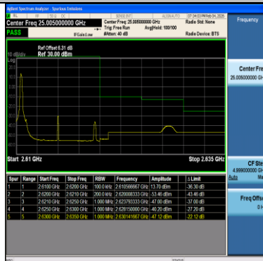
Band38-10MHz-QPSK-38200-1RB#49-PASS
