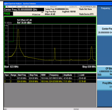
Band26(824-849)-15MHz-QPSK-26865-1RB#74-PASS
