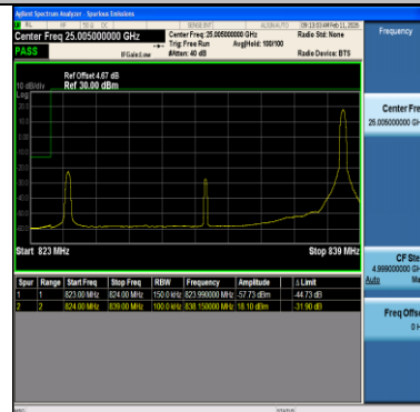
Band26(824-849)-15MHz-64QAM-26865-1RB#74-PASS
