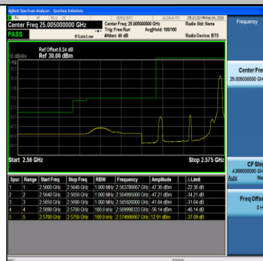
Band38-5MHz-16QAM-37775-25RB#0-PASS
