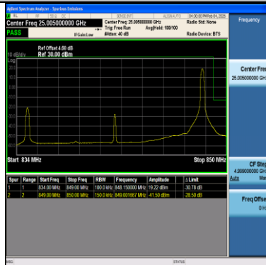
Band26(824-849)-15MHz-64QAM-26965-1RB#74-PASS
