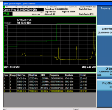
Band38-20MHz-16QAM-37850-100RB#0-PASS
