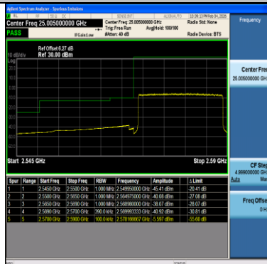
Band38-20MHz-64QAM-37850-100RB#0-PASS
