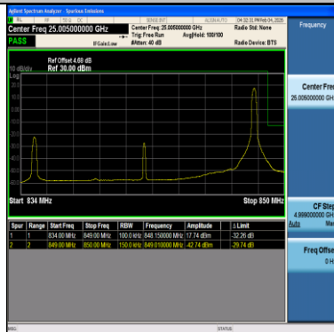
Band26(824-849)-15MHz-16QAM-26965-75RB#0-PASS
