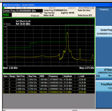
Band38-5MHz-16QAM-37775-1RB#24-PASS
