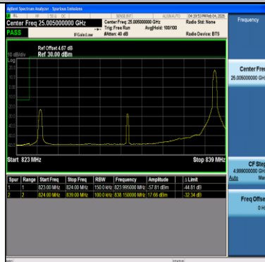
Band26(824-849)-15MHz-16QAM-26865-1RB#74-PASS
