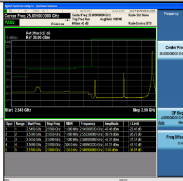
Band38-20MHz-QPSK-37850-100RB#0-PASS
