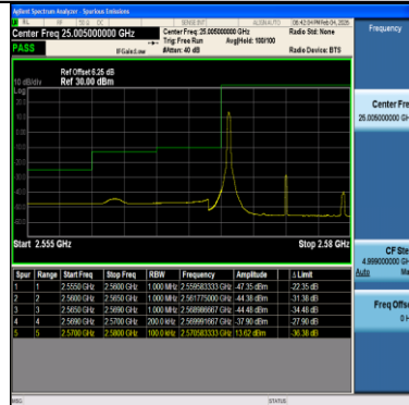
Band38-10MHz-QPSK-37800-1RB#49-PASS
