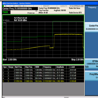
Band38-10MHz-16QAM-38200-1RB#0-PASS
