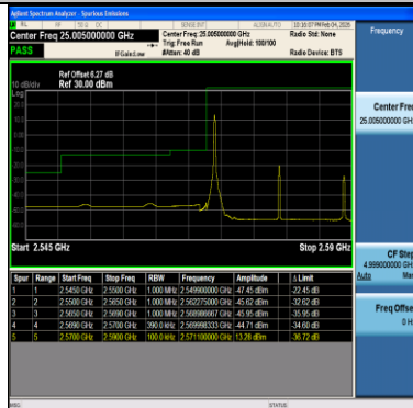
Band38-20MHz-16QAM-37850-1RB#99-PASS
