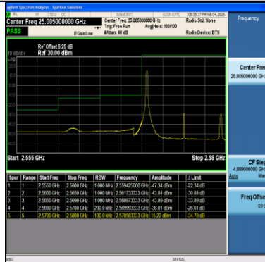
Band38-10MHz-64QAM-37800-1RB#0-PASS
