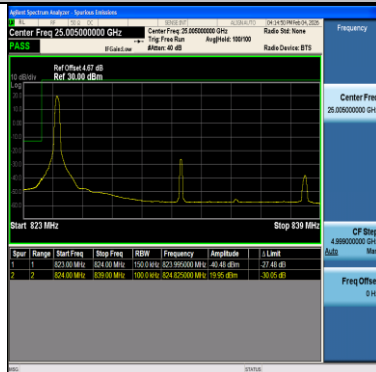
Band26(824-849)-15MHz-64QAM-26865-1RB#0-PASS
