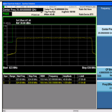
Band26(824-849)-15MHz-16QAM-26965-1RB#0-PASS
