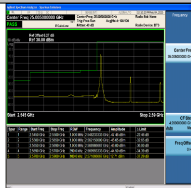
Band38-20MHz-16QAM-37850-1RB#0-PASS
