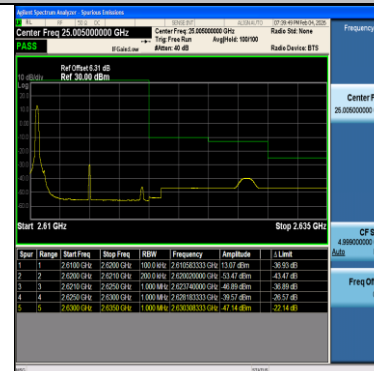
Band38-10MHz-16QAM-38200-1RB#49-PASS
