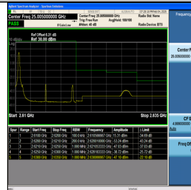
Band38-10MHz-64QAM-38200-1RB#0-PASS
