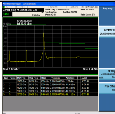
Band38-15MHz-16QAM-38175-75RB#0-PASS
