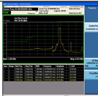
Band38-5MHz-QPSK-37775-1RB#24-PASS
