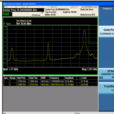
Band66-10MHz-64QAM-132622-1RB#49-PASS
