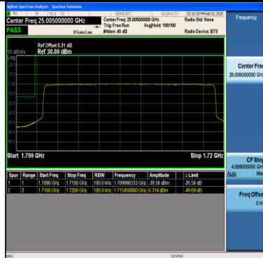
Band66-10MHz-64QAM-132022-50RB#0-PASS
