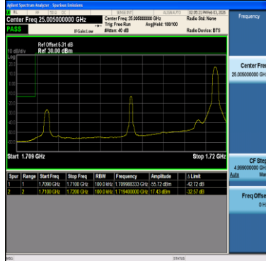
Band66-10MHz-QPSK-132022-50RB#0-PASS
