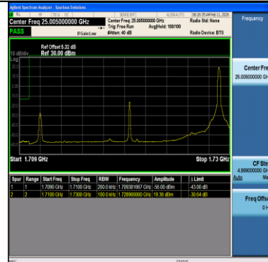
Band66-20MHz-64QAM-132072-1RB#99-PASS
