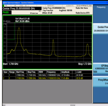
Band66-10MHz-16QAM-132022-1RB#49-PASS
