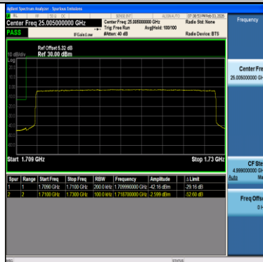
Band66-20MHz-16QAM-132572-1RB#0-PASS
