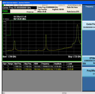
Band66-15MHz-QPSK-132047-75RB#0-PASS
