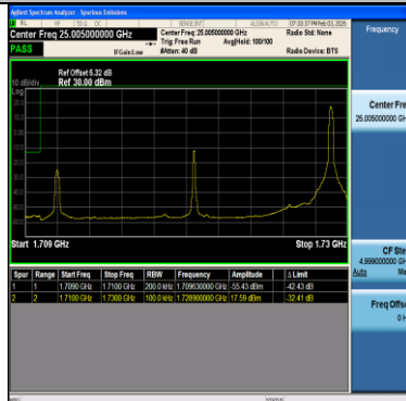
Band66-20MHz-16QAM-132072-1RB#99-PASS
