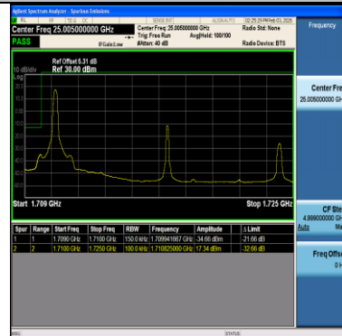
Band66-15MHz-QPSK-132047-1RB#74-PASS
