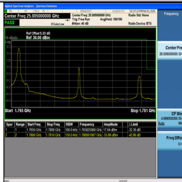
Band66-15MHz-QPSK-132597-1RB#74-PASS
