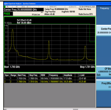
Band66-15MHz-16QAM-132597-1RB#74-PASS
