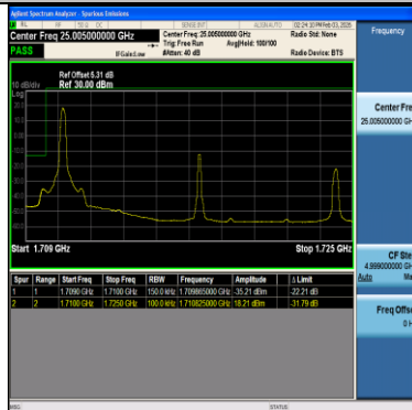
Band66-15MHz-64QAM-132047-1RB#0-PASS
