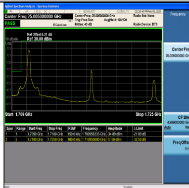
Band66-15MHz-16QAM-132047-1RB#74-PASS
