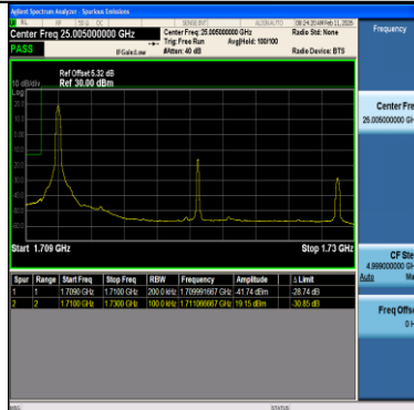
Band66-20MHz-64QAM-132072-1RB#0-PASS
