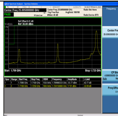
Band66-15MHz-64QAM-132047-1RB#74-PASS
