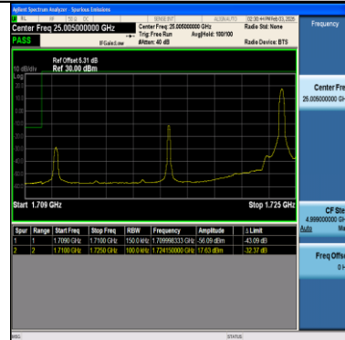
Band66-15MHz-16QAM-132047-75RB#0-PASS
