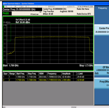
Band66-20MHz-64QAM-132072-100RB#0-PASS
