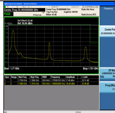
Band66-10MHz-16QAM-132622-1RB#49-PASS
