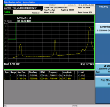
Band66-10MHz-16QAM-132022-50RB#0-PASS
