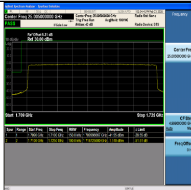
Band66-15MHz-16QAM-132597-1RB#0-PASS
