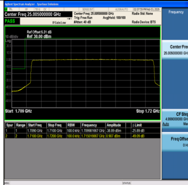
Band66-10MHz-64QAM-132022-50RB#0-PASS
