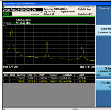
Band66-10MHz-QPSK-132622-1RB#49-PASS
