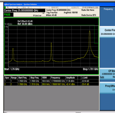
Band66-20MHz-16QAM-132572-1RB#99-PASS
