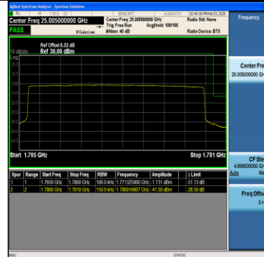
Band66-20MHz-16QAM-132072-1RB#0-PASS
