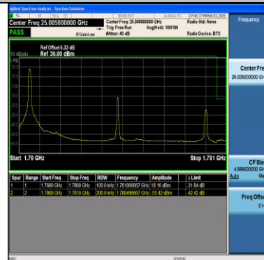
Band66-20MHz-64QAM-132572-1RB#0-PASS
