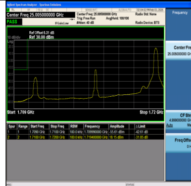
Band66-10MHz-64QAM-132022-1RB#49-PASS
