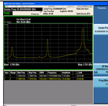
Band66-15MHz-QPSK-132597-75RB#0-PASS
