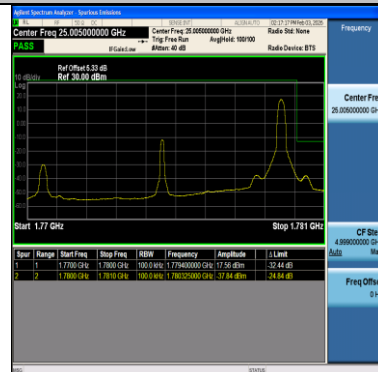
Band66-10MHz-QPSK-132622-50RB#0-PASS
