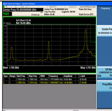
Band66-15MHz-64QAM-132597-1RB#74-PASS
