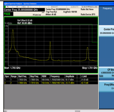
Band66-15MHz-64QAM-132597-1RB#0-PASS
