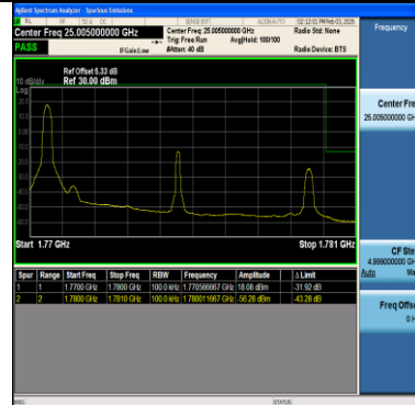
Band66-10MHz-QPSK-132622-1RB#0-PASS
