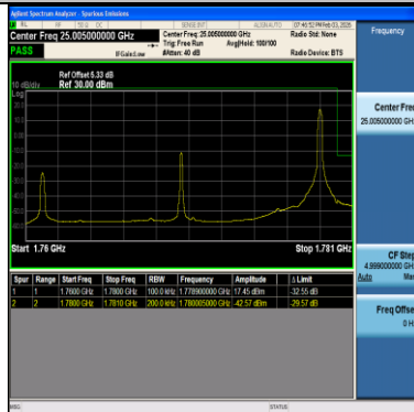
Band66-20MHz-16QAM-132572-100RB#0-PASS
