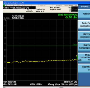
Band5-10MHz-QPSK-20600-1RB#0-3000~10000-PASS
