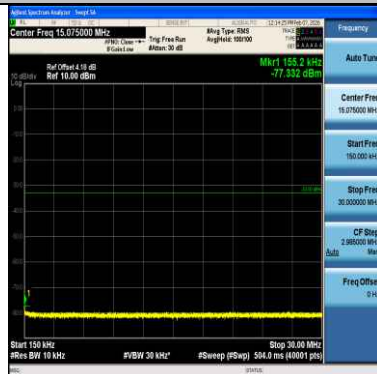
Band4-20MHz-QPSK-20050-1RB#0-0.15~30-PASS
