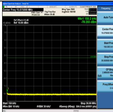
Band2-3MHz-QPSK-18615-1RB#0-0.15~30-PASS
