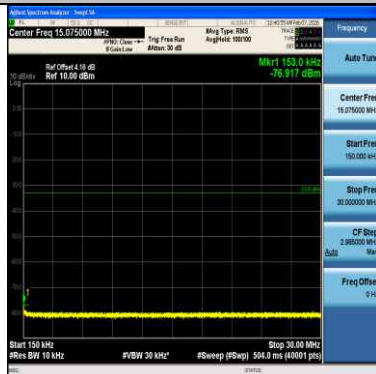
Band4-3MHz-QPSK-19965-1RB#0-0.15~30-PASS
