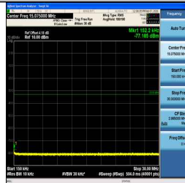
Band4-15MHz-QPSK-20325-1RB#0-0.15~30-PASS
