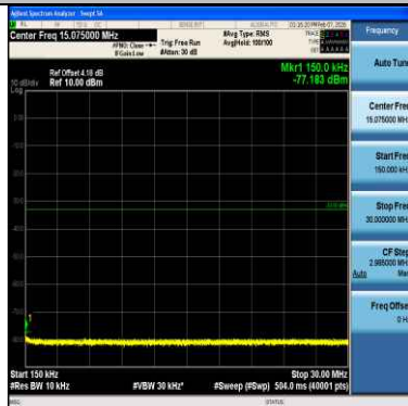
Band2-3MHz-QPSK-19185-1RB#0-1000~3000-PASS
