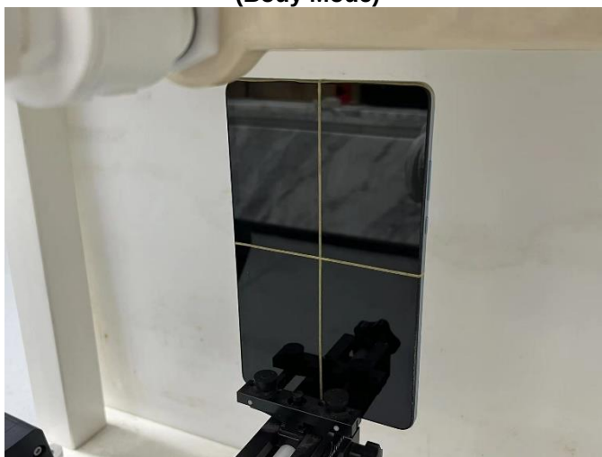
Bottom Side of EUT with 1.5 cm Gap (Body Mode)
