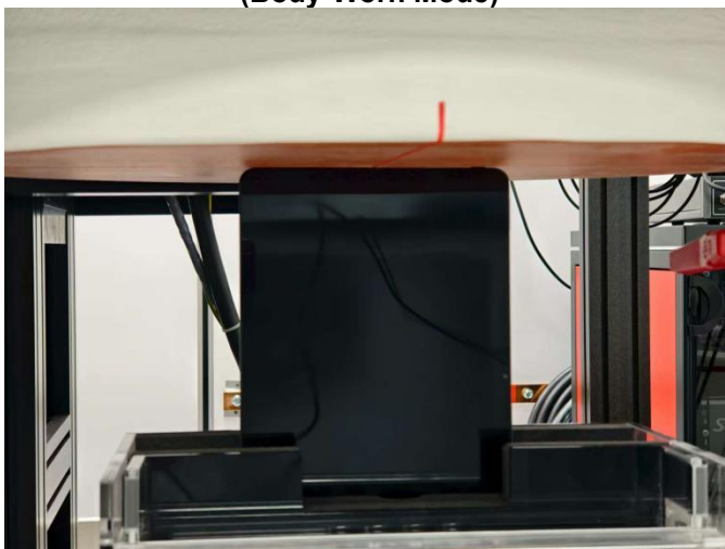
Top Side of EUT with 0 cm Gap (Body-Worn Mode)
