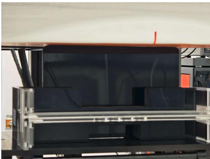
Left Side of EUT with 0 cm Gap (Body-Worn Mode)
