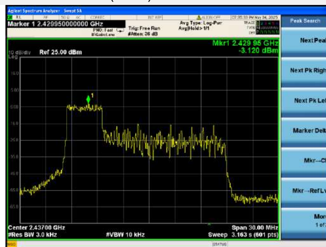
802.11be-20 MHz(RU52) MIDDLE CHANNEL
