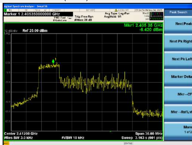
802.11be-20 MHz(RU52) LOW CHANNEL
