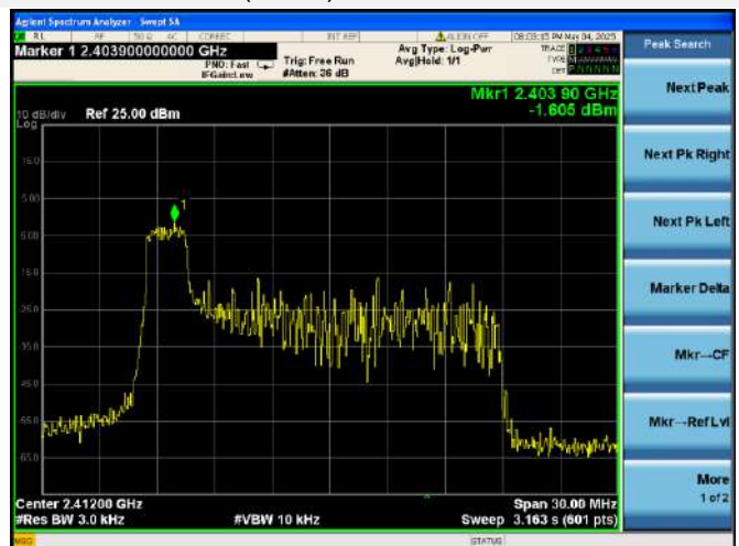
802.11be-20 MHz(RU26) LOW CHANNEL
