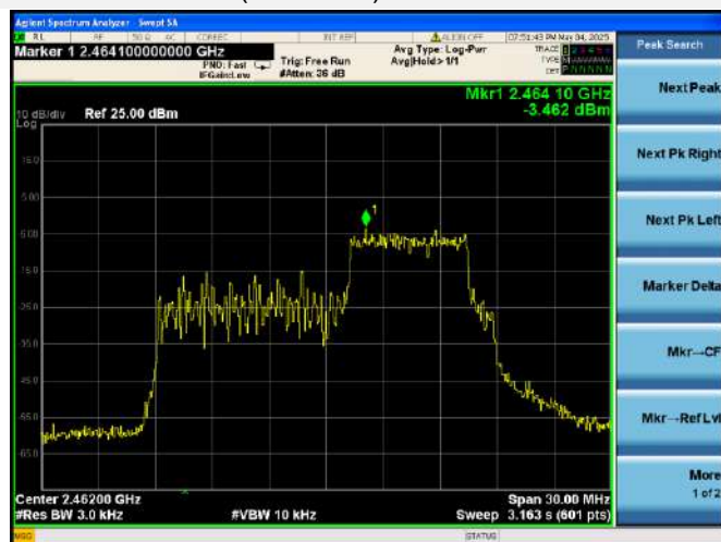
802.11be-20 MHz(RU52+26) HIGH CHANNEL
