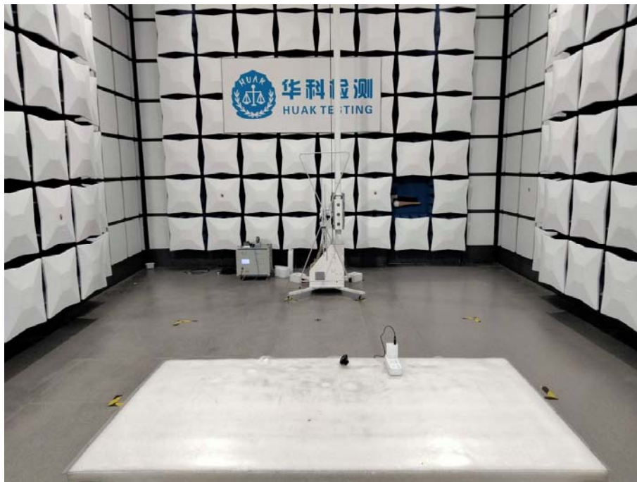
Test Model: BV-081 Radiated Emissions
