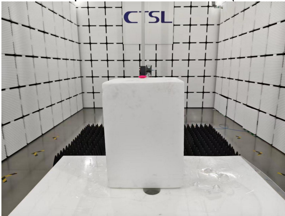
Photo 3 Test Setup Photos of Radiated Emission Test (Above 1GHz)
