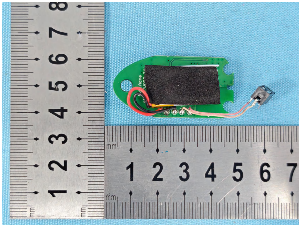
Photo 4 Internal photos of EUT Mian Test Model: TOG-025
