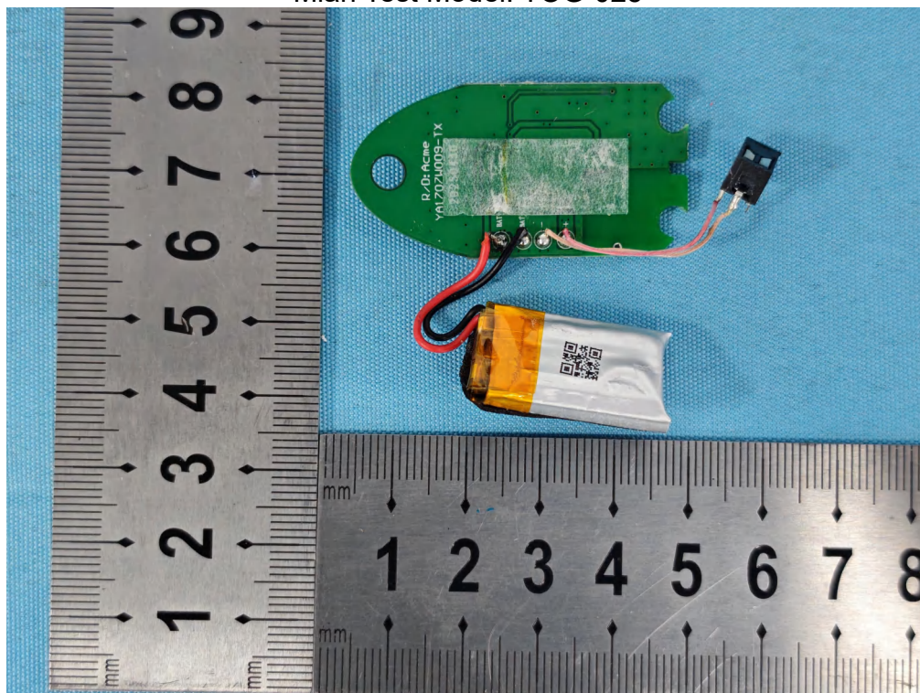
Photo 5 Internal photos of EUT Mian Test Model: TOG-025
