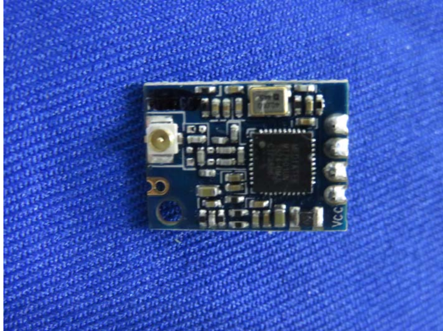
Figure 22 PCB of The EUT- Front View (WiFi Module)
