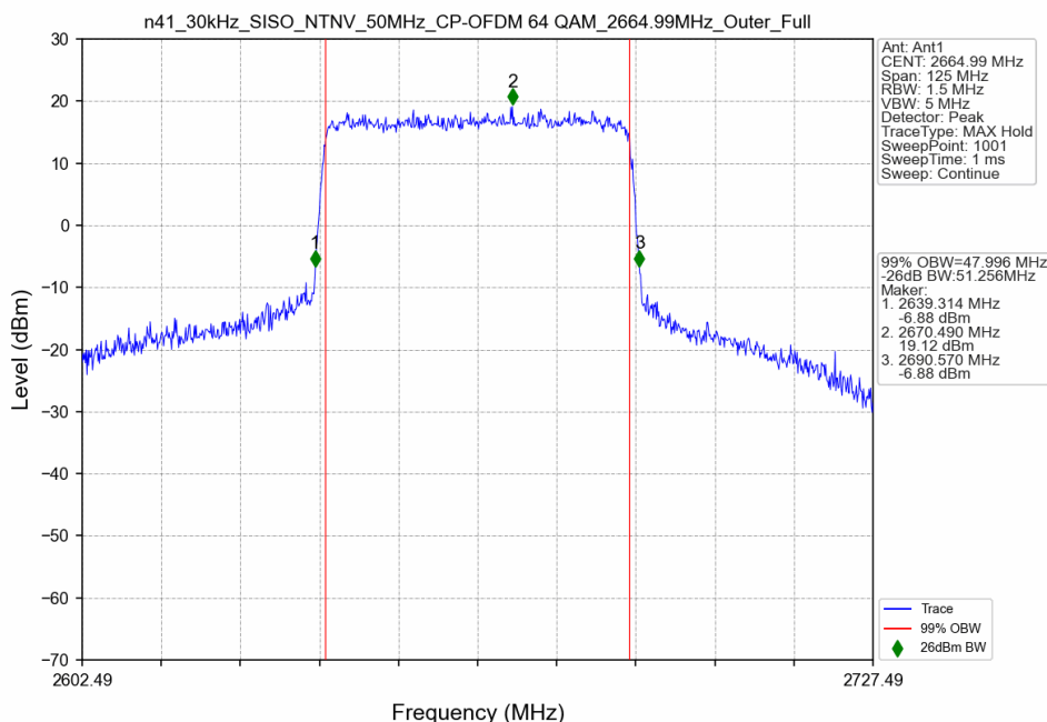
n41_30kHz_SISO_NTNV_50MHz_CP-OFDM 64 QAM_2664.99MHz_Outer_Full
