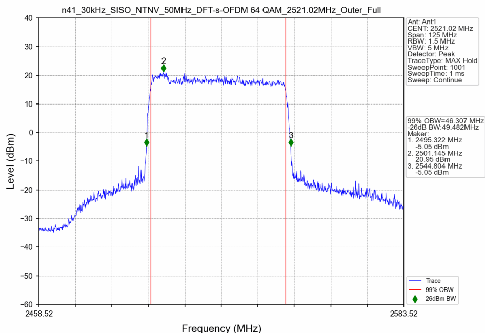
n41_30kHz_SISO_NTNV_50MHz_DFT-s-OFDM 64 QAM_2521.02MHz_Outer_Full
