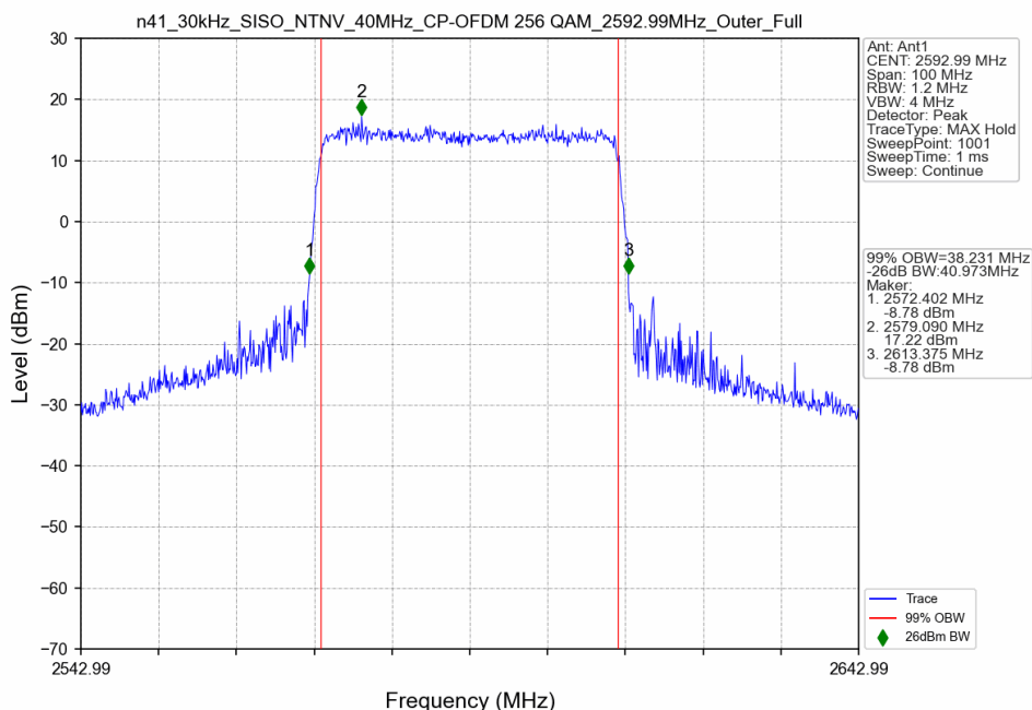
n41_30kHz_SISO_NTNV_40MHz_CP-OFDM 256 QAM_2592.99MHz_Outer_Full
