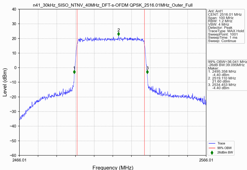
n41_30kHz_SISO_NTNV_40MHz_DFT-s-OFDM QPSK_2516.01MHz_Outer_Full
