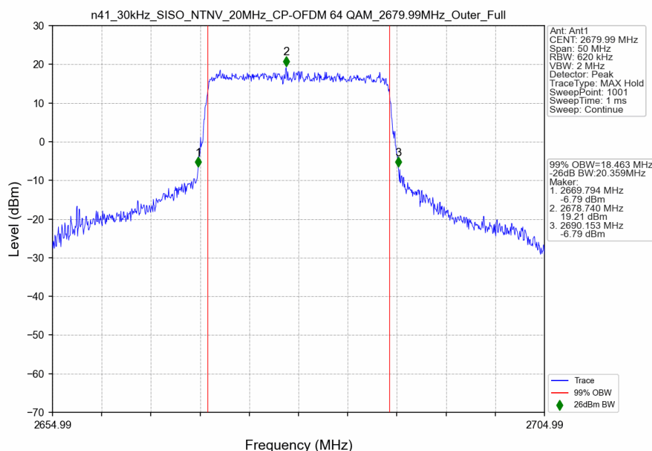
n41_30kHz_SISO_NTNV_20MHz_CP-OFDM 64 QAM_2679.99MHz_Outer_Full
