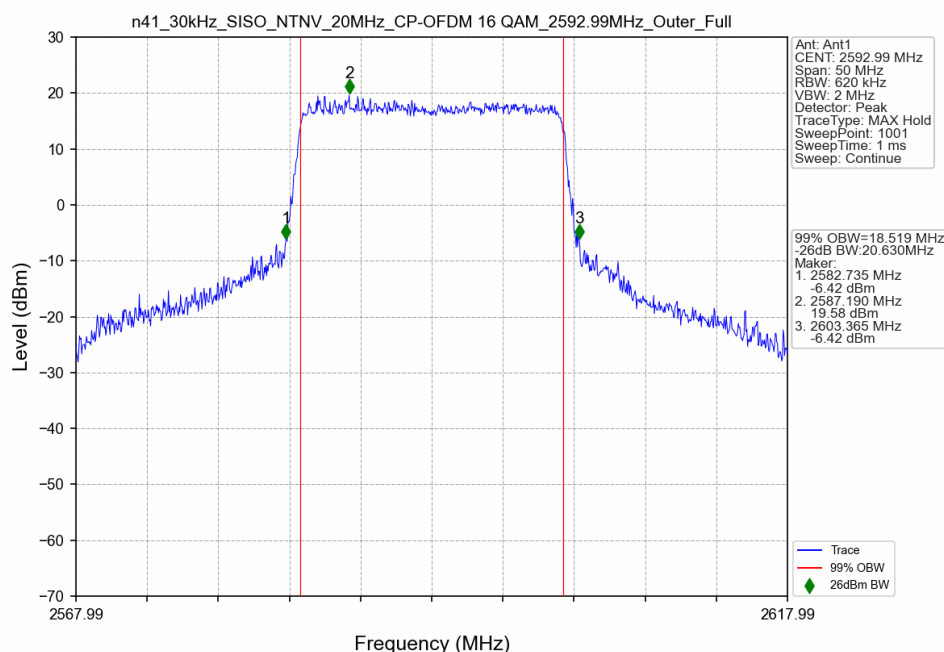
n41_30kHz_SISO_NTNV_20MHz_CP-OFDM 16 QAM_2592.99MHz_Outer_Full
