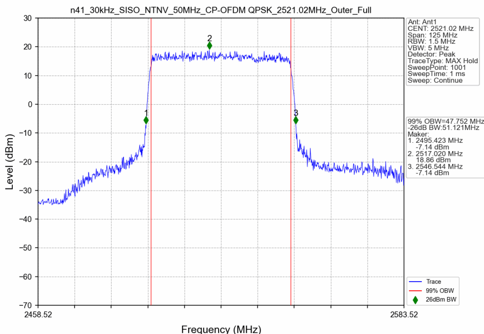
n41_30kHz_SISO_NTNV_50MHz_CP-OFDM QPSK_2521.02MHz_Outer_Full
