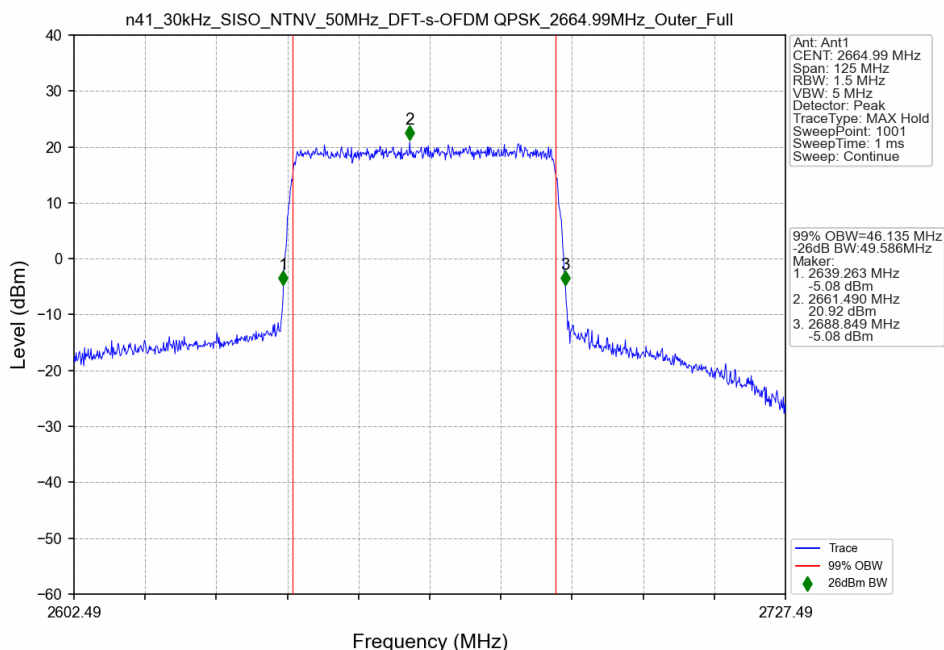
n41_30kHz_SISO_NTNV_50MHz_DFT-s-OFDM QPSK_2664.99MHz_Outer_Full
