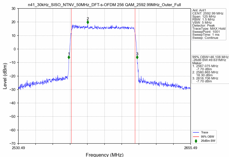
n41_30kHz_SISO_NTNV_50MHz_DFT-s-OFDM 256 QAM_2592.99MHz_Outer_Full
