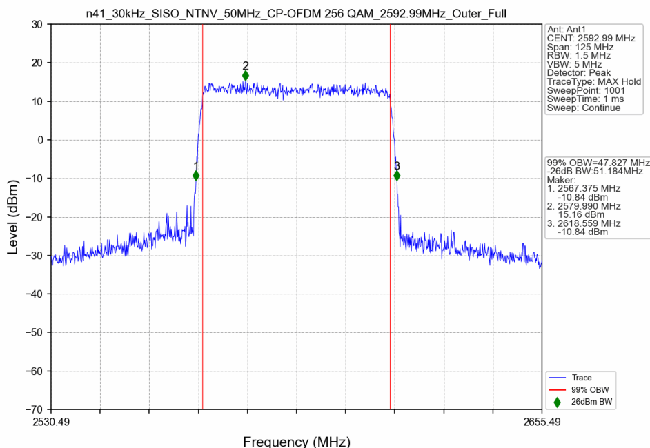
n41_30kHz_SISO_NTNV_50MHz_CP-OFDM 256 QAM_2592.99MHz_Outer_Full
