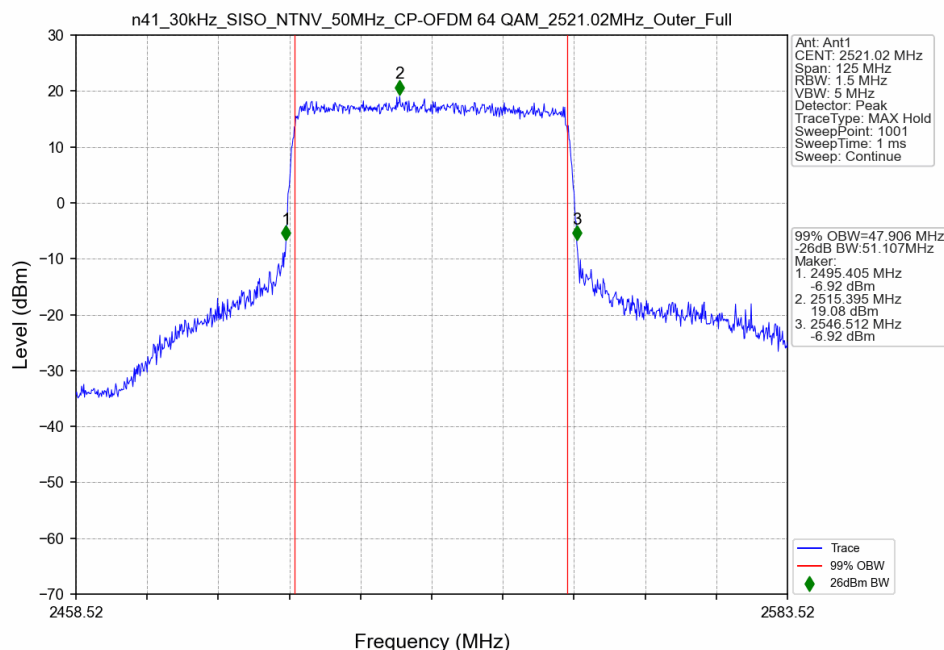
n41_30kHz_SISO_NTNV_50MHz_CP-OFDM 64 QAM_2521.02MHz_Outer_Full
