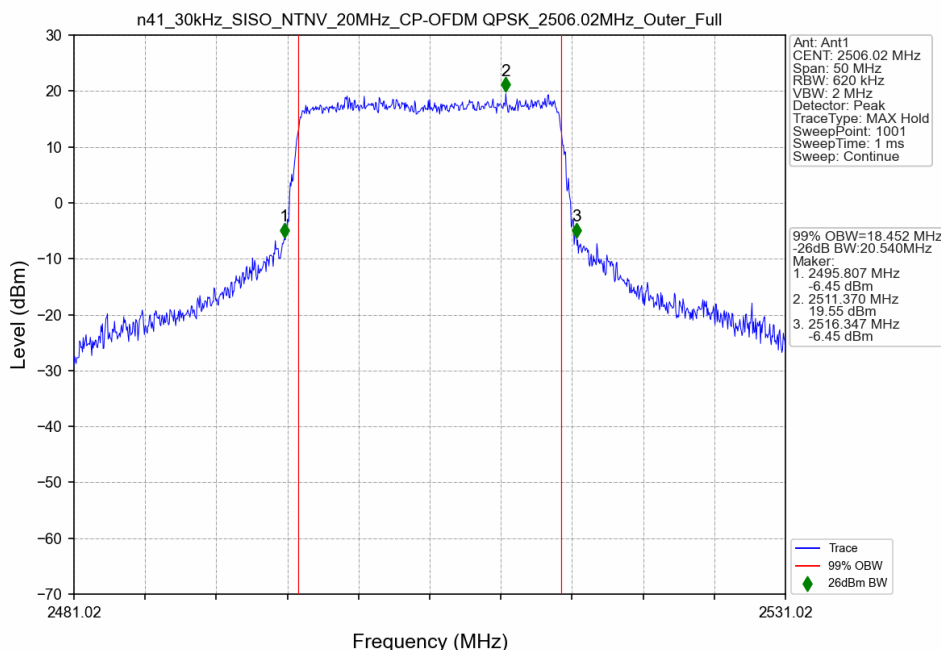
n41_30kHz_SISO_NTNV_20MHz_CP-OFDM QPSK_2506.02MHz_Outer_Full
