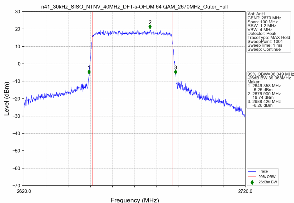
n41_30kHz_SISO_NTNV_40MHz_DFT-s-OFDM 64 QAM_2670MHz_Outer_Full
