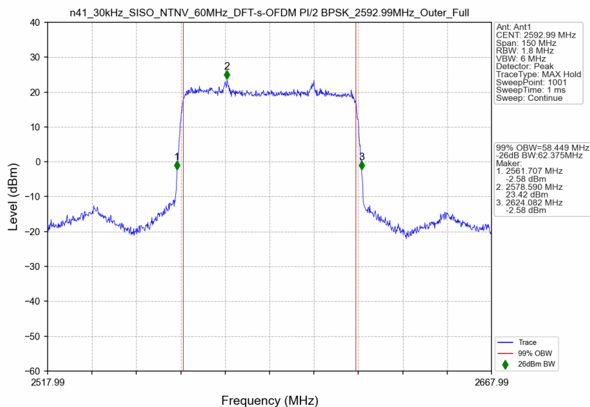
n41_30kHz_SISO_NTNV_60MHz_DFT-s-OFDM PI/2 BPSK_2592.99MHz_Outer_Full
