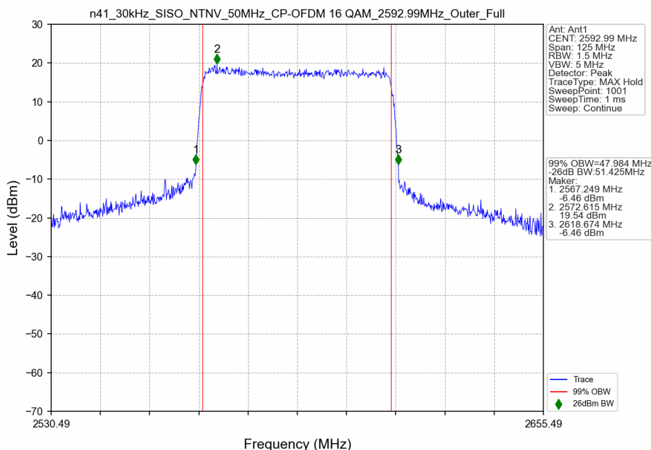
n41_30kHz_SISO_NTNV_50MHz_CP-OFDM 16 QAM_2592.99MHz_Outer_Full
