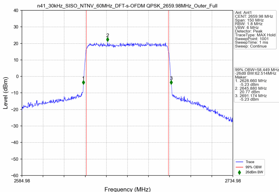
n41_30kHz_SISO_NTNV_60MHz_DFT-s-OFDM QPSK_2659.98MHz_Outer_Full
