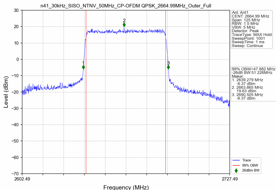
n41_30kHz_SISO_NTNV_50MHz_CP-OFDM QPSK_2664.99MHz_Outer_Full
