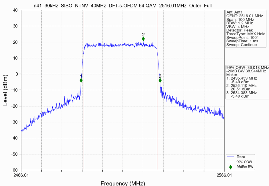
n41_30kHz_SISO_NTNV_40MHz_DFT-s-OFDM 64 QAM_2516.01MHz_Outer_Full
