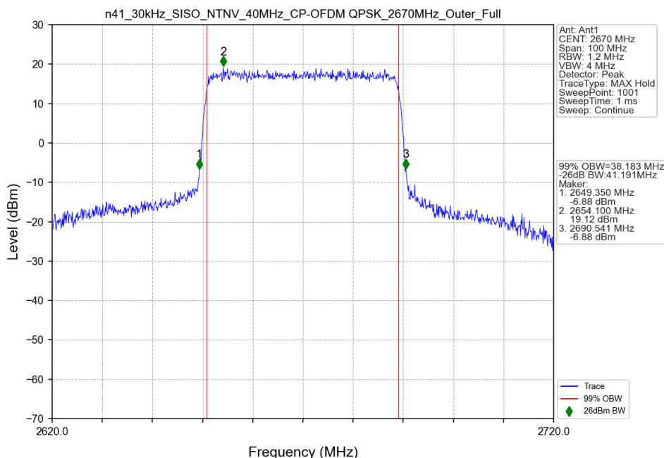
n41_30kHz_SISO_NTNV_40MHz_CP-OFDM QPSK_2670MHz_Outer_Full
