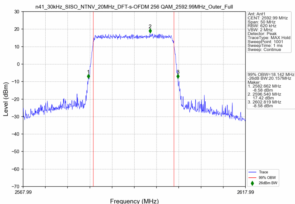
n41_30kHz_SISO_NTNV_20MHz_DFT-s-OFDM 256 QAM_2592.99MHz_Outer_Full
