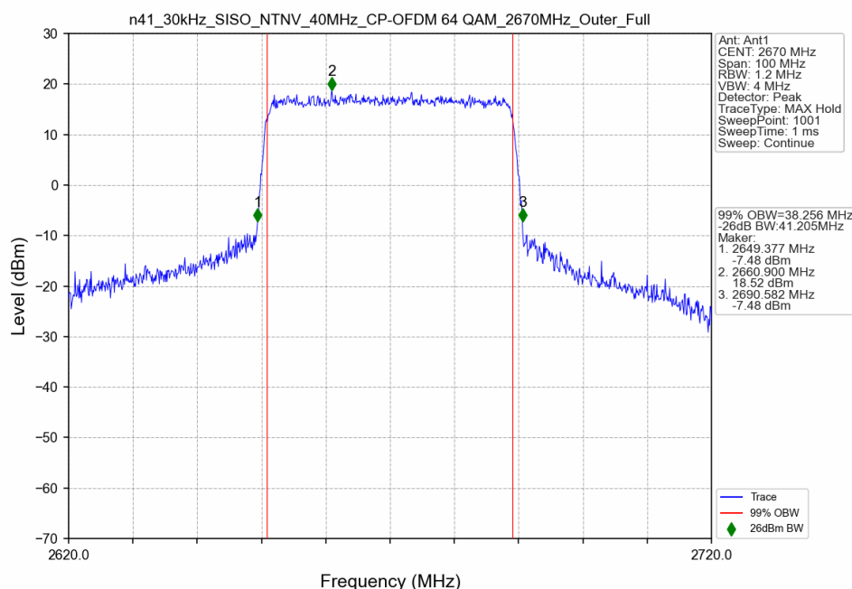
n41_30kHz_SISO_NTNV_40MHz_CP-OFDM 64 QAM_2670MHz_Outer_Full
