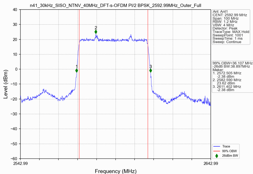
n41_30kHz_SISO_NTNV_40MHz_DFT-s-OFDM PI/2 BPSK_2592.99MHz_Outer_Full
