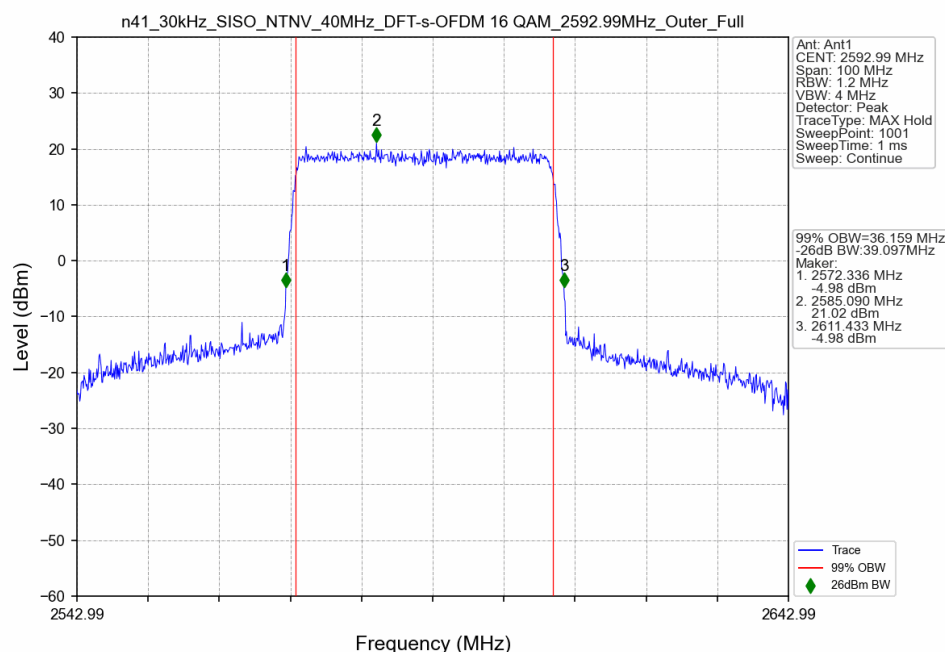
n41_30kHz_SISO_NTNV_40MHz_DFT-s-OFDM 16 QAM_2592.99MHz_Outer_Full
