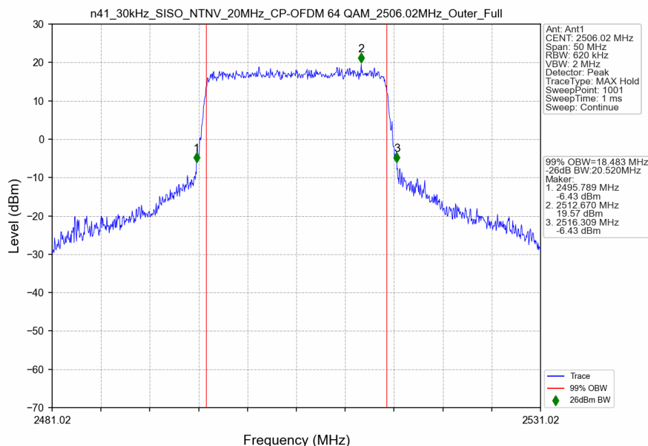
n41_30kHz_SISO_NTNV_20MHz_CP-OFDM 64 QAM_2506.02MHz_Outer_Full
