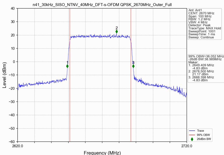
n41_30kHz_SISO_NTNV_40MHz_DFT-s-OFDM QPSK_2670MHz_Outer_Full
