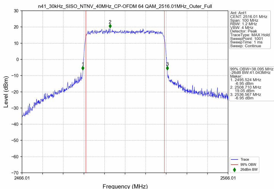
n41_30kHz_SISO_NTNV_40MHz_CP-OFDM 64 QAM_2516.01MHz_Outer_Full
