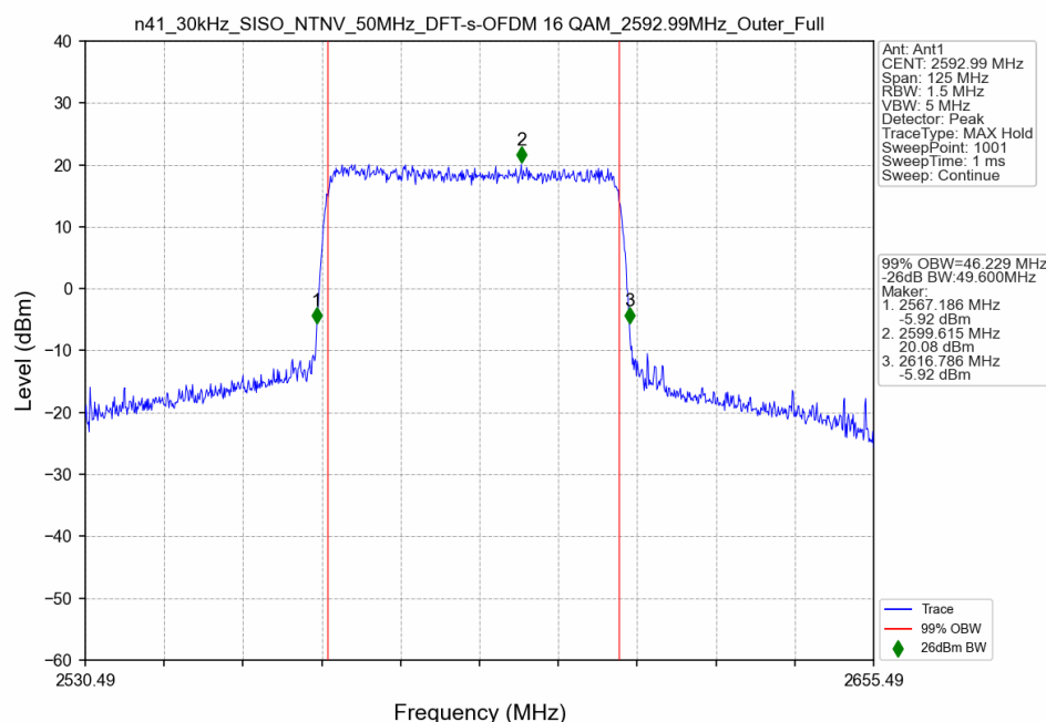
n41_30kHz_SISO_NTNV_50MHz_DFT-s-OFDM 16 QAM_2592.99MHz_Outer_Full
