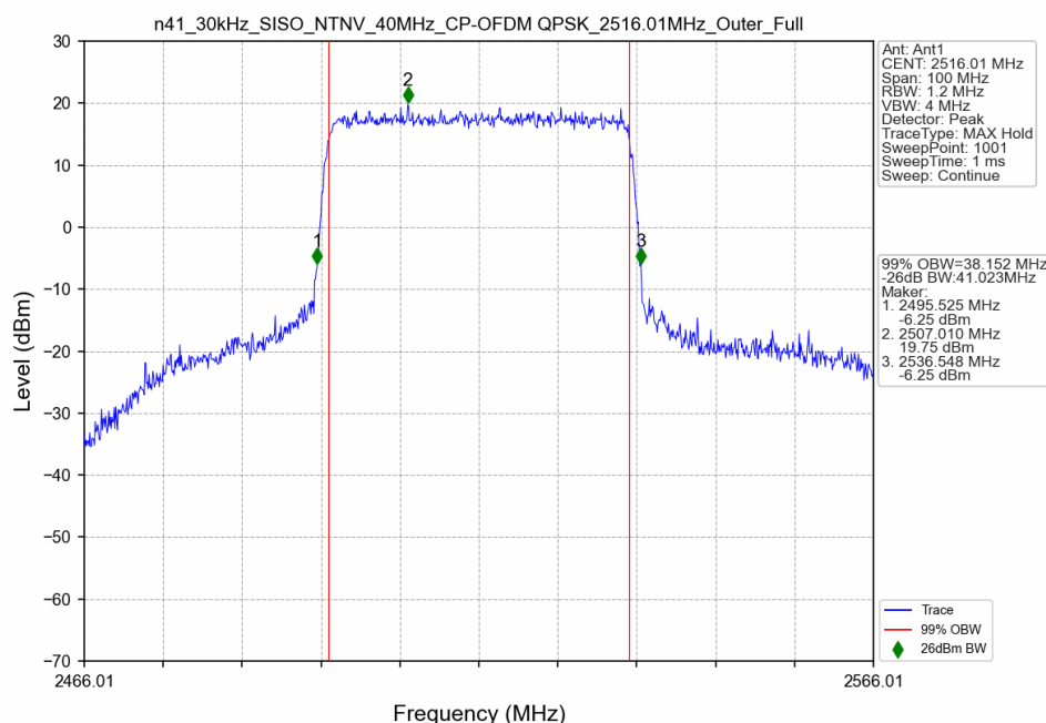
n41_30kHz_SISO_NTNV_40MHz_CP-OFDM QPSK_2516.01MHz_Outer_Full
