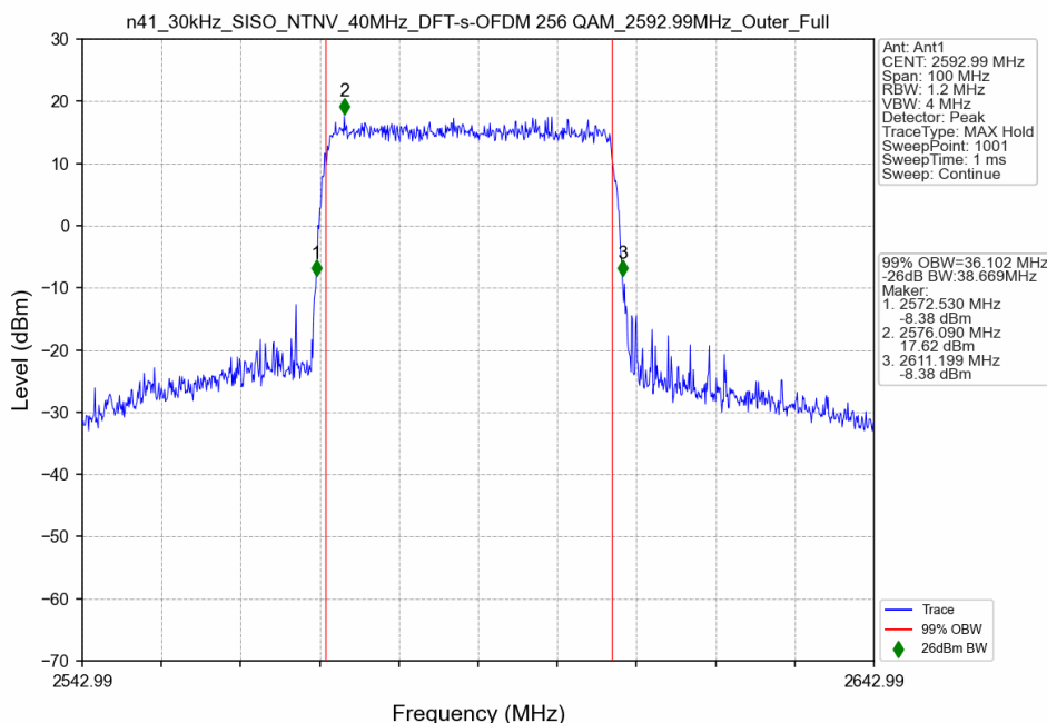
n41_30kHz_SISO_NTNV_40MHz_DFT-s-OFDM 256 QAM_2592.99MHz_Outer_Full
