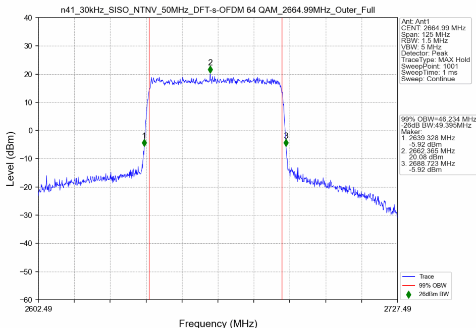
n41_30kHz_SISO_NTNV_50MHz_DFT-s-OFDM 64 QAM_2664.99MHz_Outer_Full
