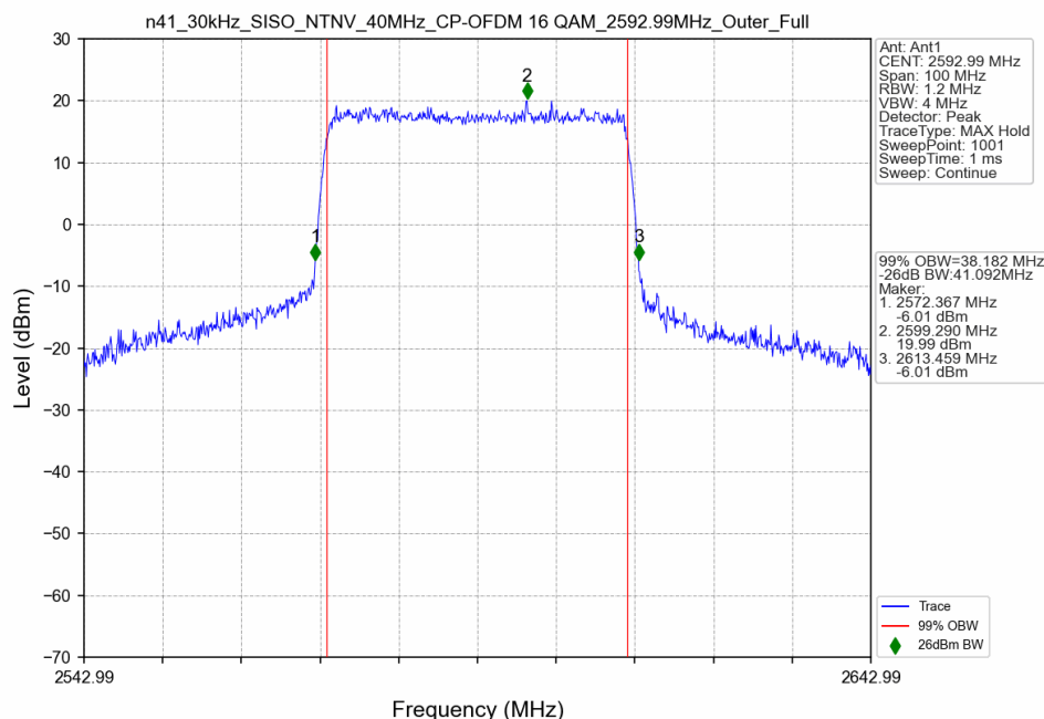
n41_30kHz_SISO_NTNV_40MHz_CP-OFDM 16 QAM_2592.99MHz_Outer_Full
