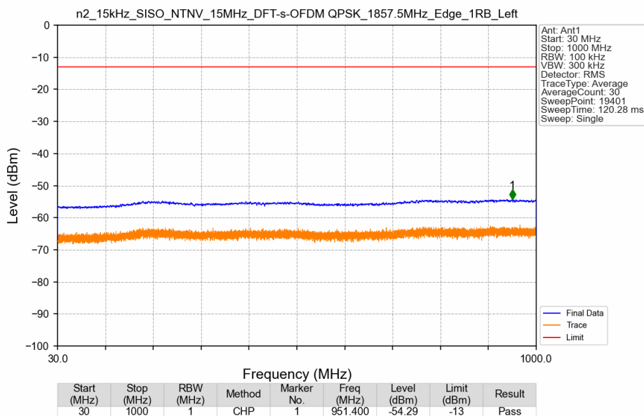
n2_15kHz_SISO_NTNV_15MHz_DFT-s-OFDM QPSK_1857.5MHz_Edge_1RB_Left
