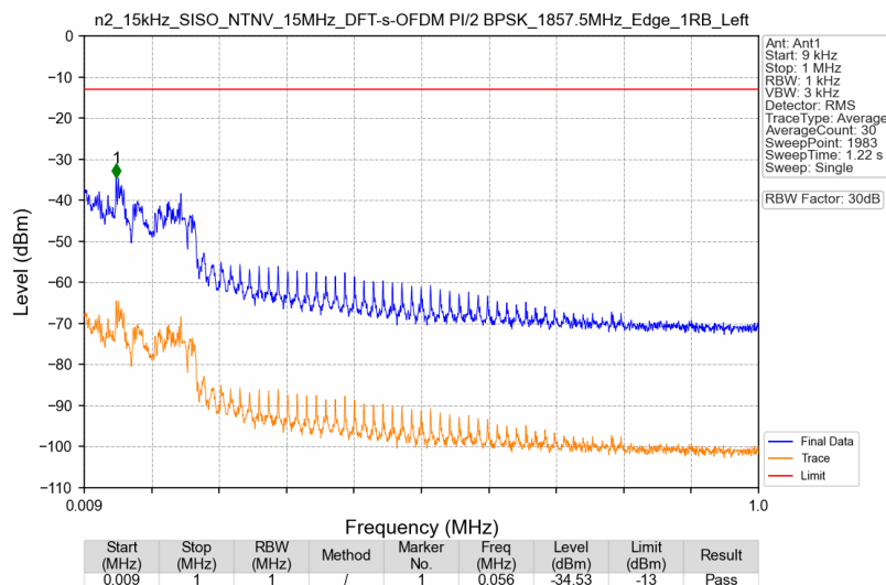
n2_15kHz_SISO_NTNV_15MHz_DFT-s-OFDM PI/2 BPSK_1857.5MHz_Edge_1RB_Left
