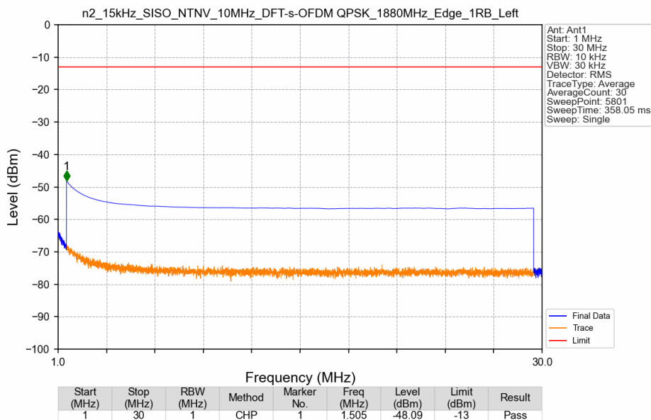
n2_15kHz_SISO_NTNV_10MHz_DFT-s-OFDM QPSK_1880MHz_Edge_1RB_Left
