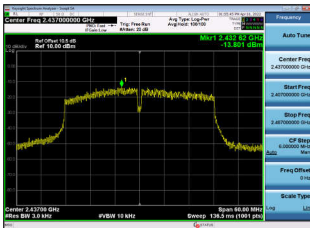
Power spectral density-802.11ax(HE40) ,2437MHz,Ant1
