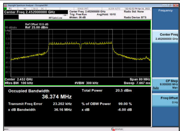
6dB Bandwidth-802.11ax(HE40),2452MHz ,Ant0
