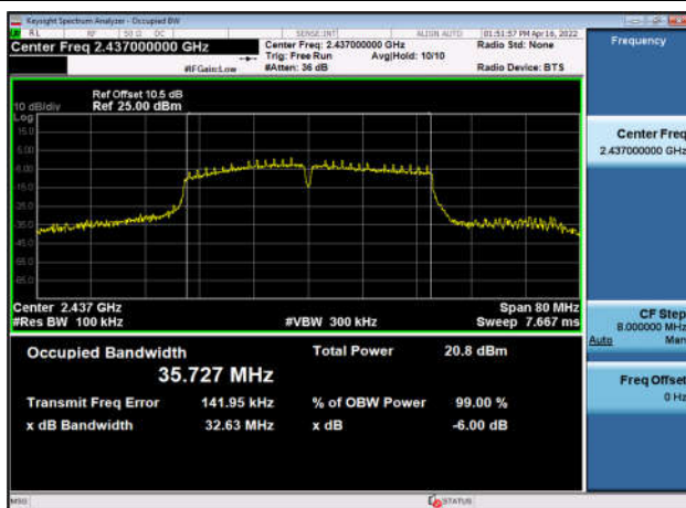
6dB Bandwidth-802.11ax(HE40),2437MHz ,Ant1
