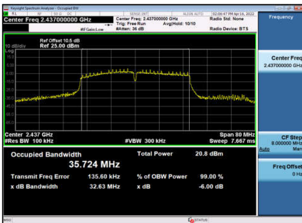
6dB Bandwidth-802.11n(HT40),2437MHz ,Ant1
