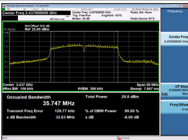
6dB Bandwidth-802.11ax(HE40),2437MHz ,Ant0
