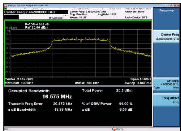
6dB Bandwidth-802.11g,2462MHz,Ant1
