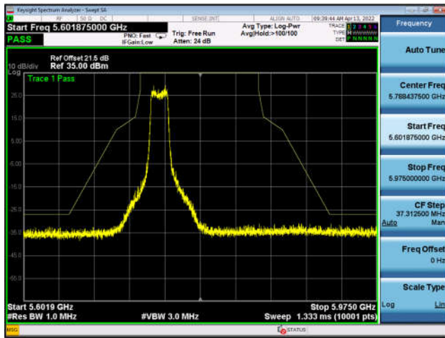
U-NII-3 ,802.11ac-VHT20, 5785MHz, Ant5
