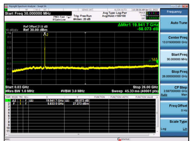
U-NII-3 ,802.11ac-VHT20, 5825MHz, Ant5
