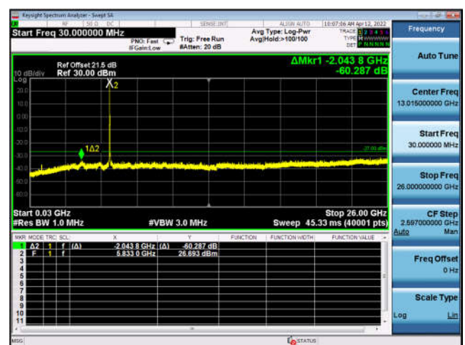
U-NII-3 ,802.11n-HT20, 5825MHz, Ant4
