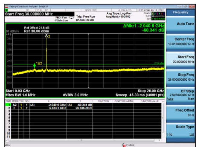
U-NII-3 ,802.11a, 5825MHz, Ant5
