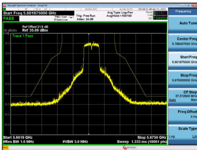
U-NII-3 ,802.11ac-VHT40, 5755MHz, Ant5
