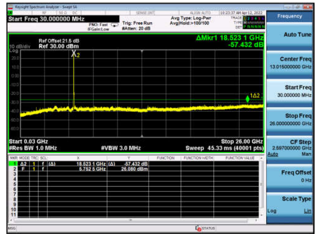
U-NII-3 ,802.11a, 5785MHz, Ant5
