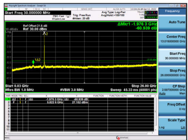
U-NII-3 ,802.11a, 5825MHz, Ant4
