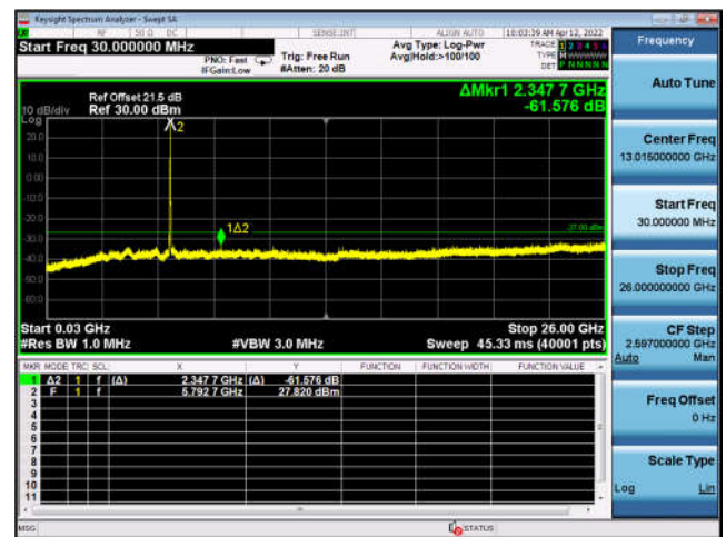
U-NII-3 ,802.11a, 5825MHz, Ant4
