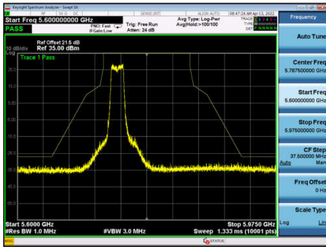
U-NII-3 ,802.11n-HT20, 5785MHz, Ant4
