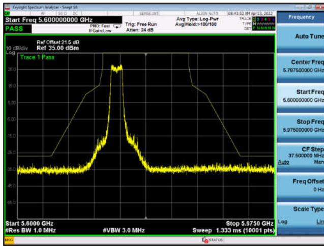
U-NII-3 ,802.11a, 5785MHz, Ant4
