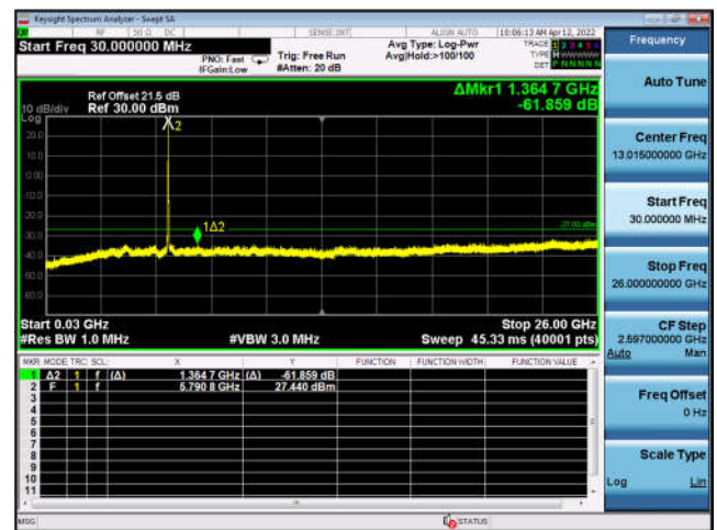
U-NII-3 ,802.11n-HT20, 5825MHz, Ant4
