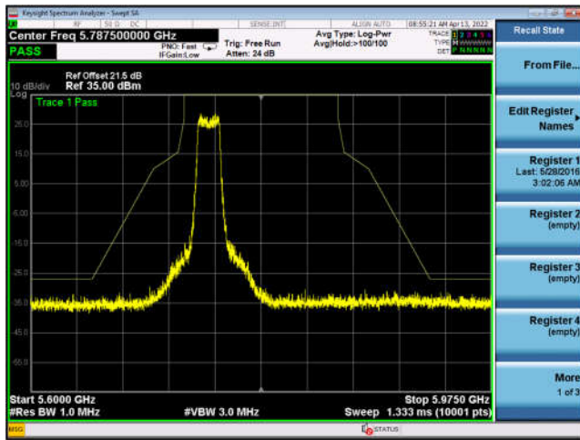
U-NII-3 ,802.11ac-VHT20, 5785MHz, Ant4
