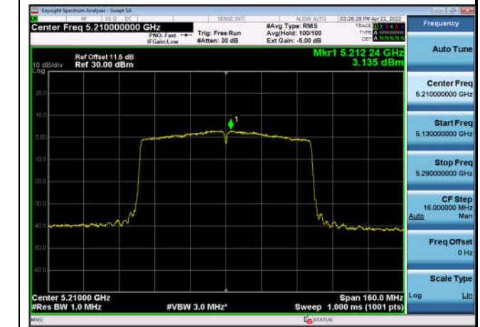
U-NII-1 Power spectral density-802.11 ac(80MHz),5210MHz,Ant1
