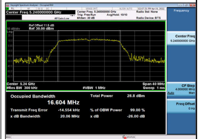
U-NII-1 99% OBW & 26 EBW-802.11a(20MHz) ,5240MHz,Ant5
