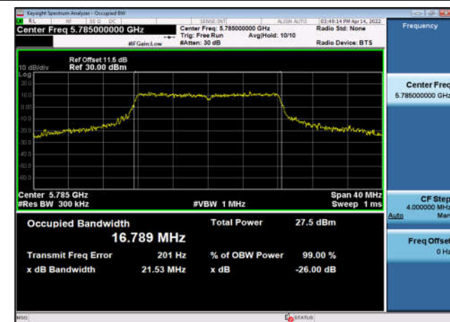
U-NII-3 99% OBW & 26 EBW-802.11a(20MHz) ,5785MHz,Ant2
