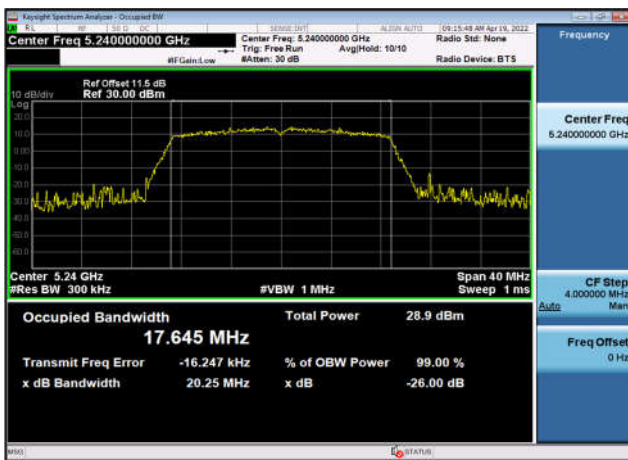
U-NII-1 99% OBW & 26 EBW-802.11ax(20MHz) ,5240MHz,Ant3
