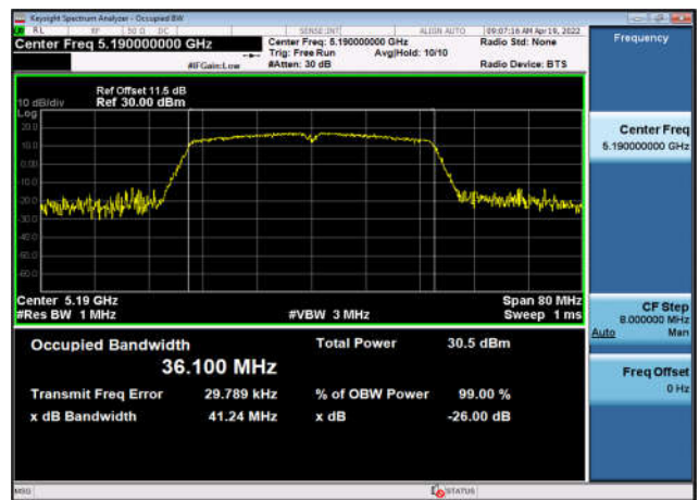
U-NII-1 99% OBW & 26 EBW-802.11ax(40MHz) ,5190MHz,Ant3
