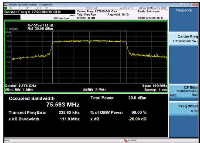
U-NII-3 99% OBW & 26 EBW-802.11ax(80MHz) ,5775MHz,Ant2
