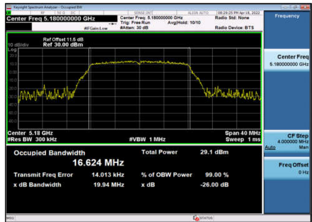
U-NII-1 99% OBW & 26 EBW-802.11a(20MHz) ,5180MHz,Ant3
