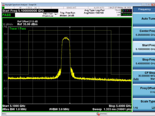
U-NII-1 ,802.11n-HT20, 5240MHz, Ant4
