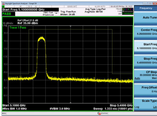
U-NII-1 ,802.11ac-VHT20, 5220MHz, Ant4
