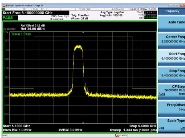
U-NII-1 ,802.11ax-HE20, 5240MHz, Ant4
