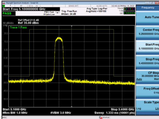
U-NII-1 ,802.11ac-VHT20, 5240MHz, Ant4
