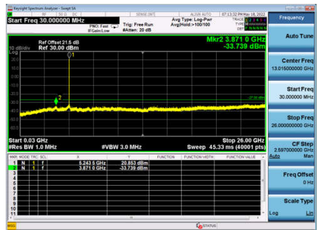
U-NII-1 ,802.11ac-VHT20, 5240MHz, Ant5
