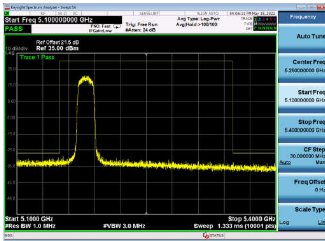
U-NII-1 ,802.11ac-VHT20, 5220MHz, Ant5
