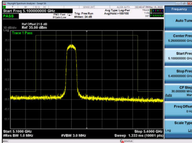
U-NII-1 ,802.11ac-VHT20, 5240MHz, Ant5
