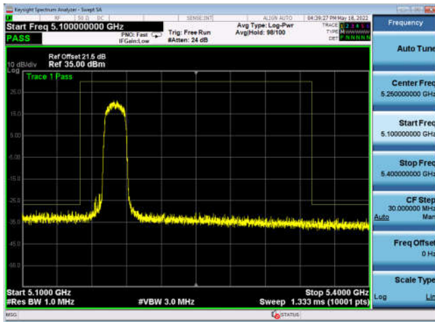
U-NII-1 ,802.11n-HT20, 5220MHz, Ant4
