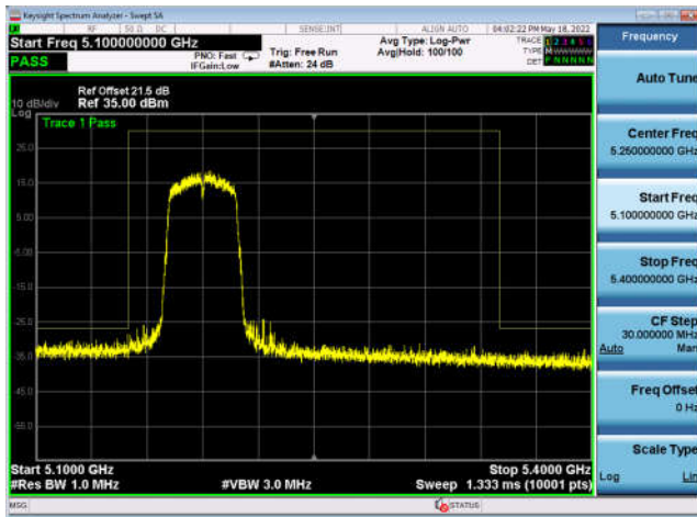
U-NII-1 ,802.11n-HT40, 5230MHz, Ant5
