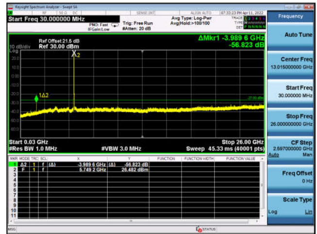
U-NII-3 ,802.11n-HT20, 5785MHz, Ant2
