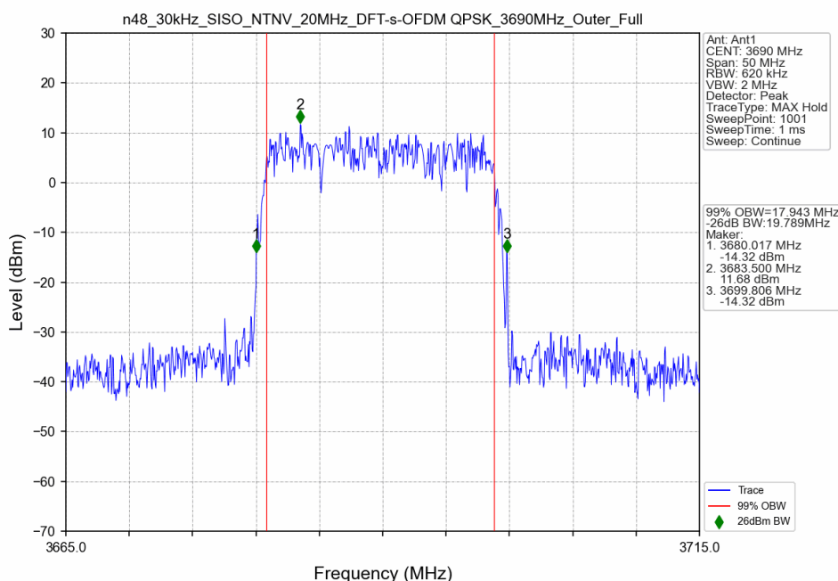
n48_30kHz_SISO_NTNV_20MHz_DFT-s-OFDM QPSK_3690MHz_Outer_Full_Ant1
