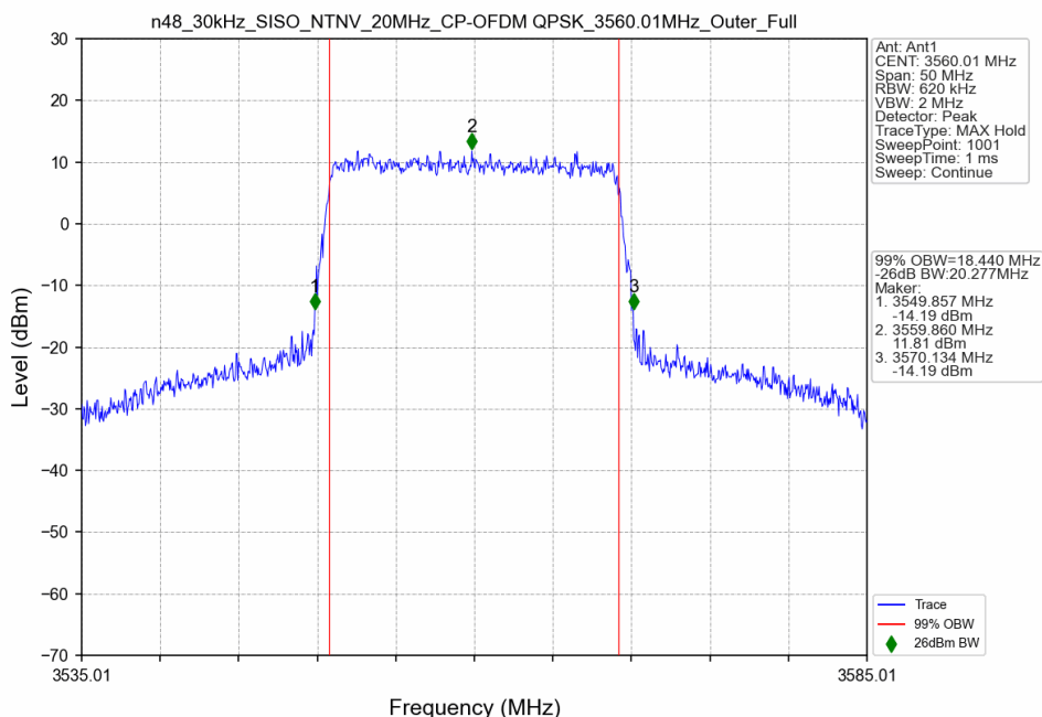
n48_30kHz_SISO_NTNV_20MHz_CP-OFDM QPSK_3560.01MHz_Outer_Full_Ant1
