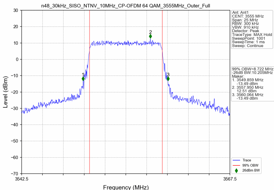
n48_30kHz_SISO_NTNV_10MHz_CP-OFDM 64 QAM_3555MHz_Outer_Full_Ant1
