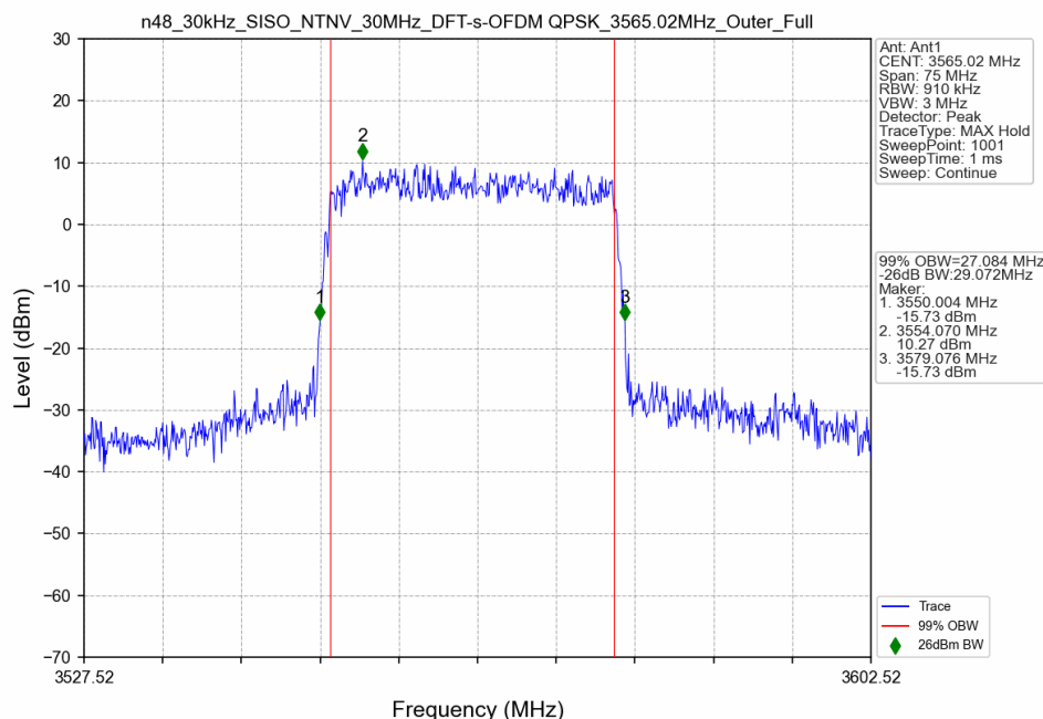
n48_30kHz_SISO_NTNV_30MHz_DFT-s-OFDM QPSK_3565.02MHz_Outer_Full_Ant1
