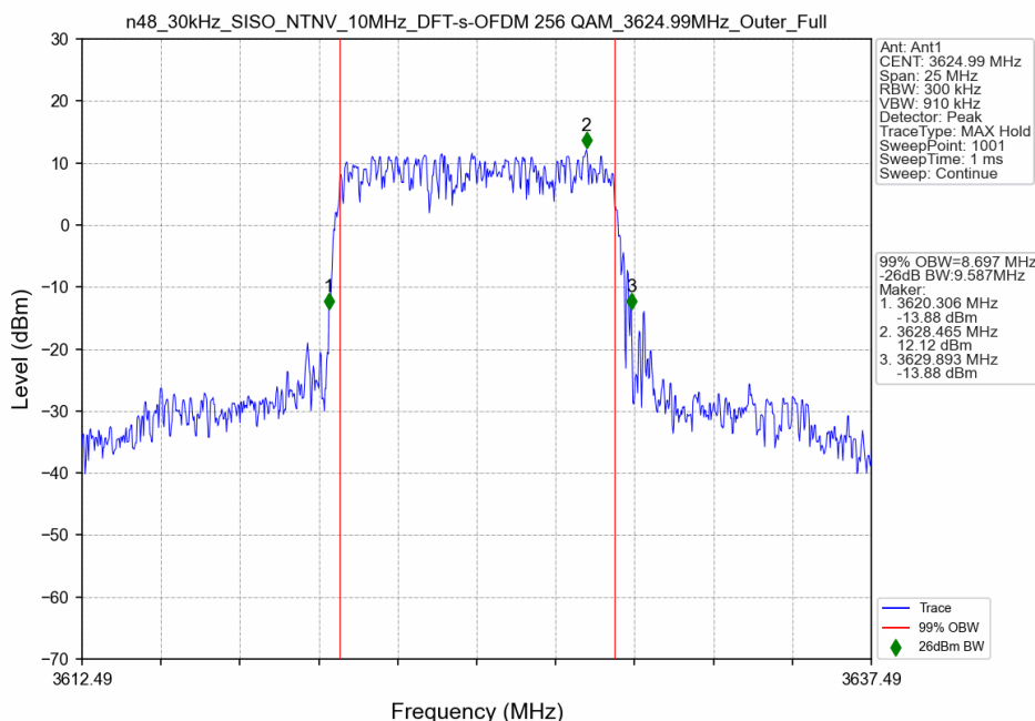
n48_30kHz_SISO_NTNV_10MHz_DFT-s-OFDM 256 QAM_3624.99MHz_Outer_Full_Ant1
