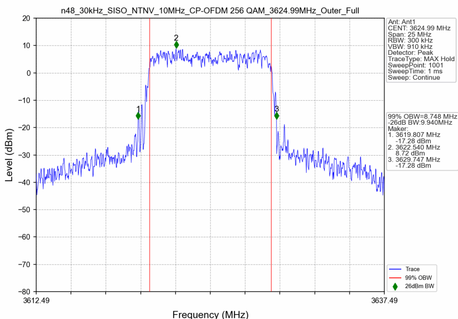
n48_30kHz_SISO_NTNV_10MHz_CP-OFDM 256 QAM_3624.99MHz_Outer_Full_Ant1
