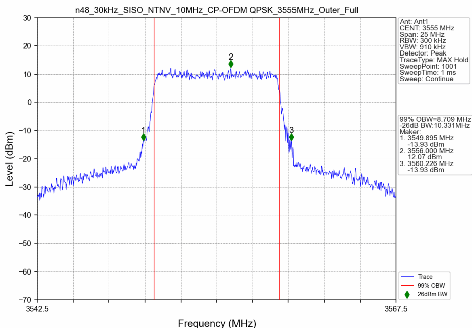
n48_30kHz_SISO_NTNV_10MHz_CP-OFDM QPSK_3555MHz_Outer_Full_Ant1
