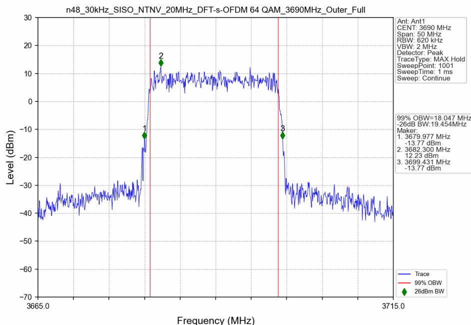
n48_30kHz_SISO_NTNV_20MHz_DFT-s-OFDM 64 QAM_3690MHz_Outer_Full_Ant1
