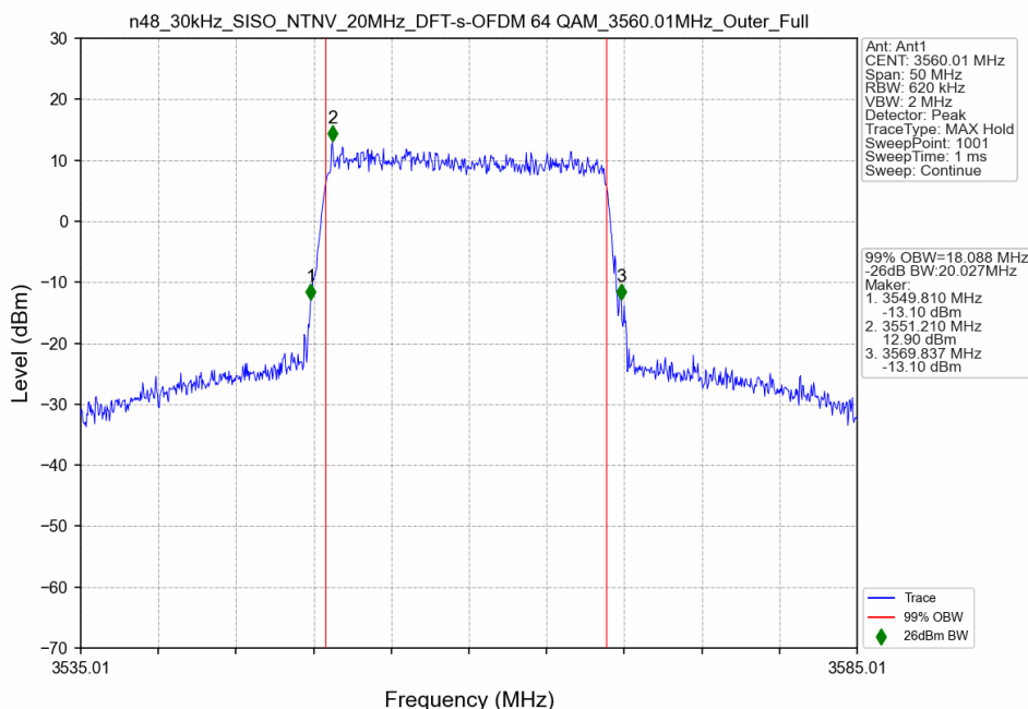
n48_30kHz_SISO_NTNV_20MHz_DFT-s-OFDM 64 QAM_3560.01MHz_Outer_Full_Ant1
