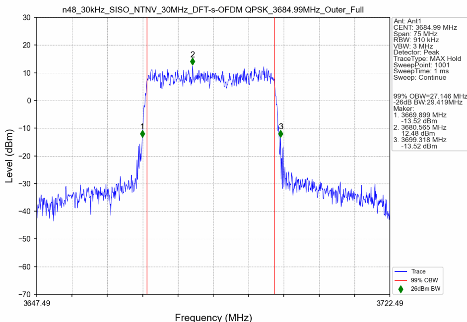
n48_30kHz_SISO_NTNV_30MHz_DFT-s-OFDM QPSK_3684.99MHz_Outer_Full_Ant1
