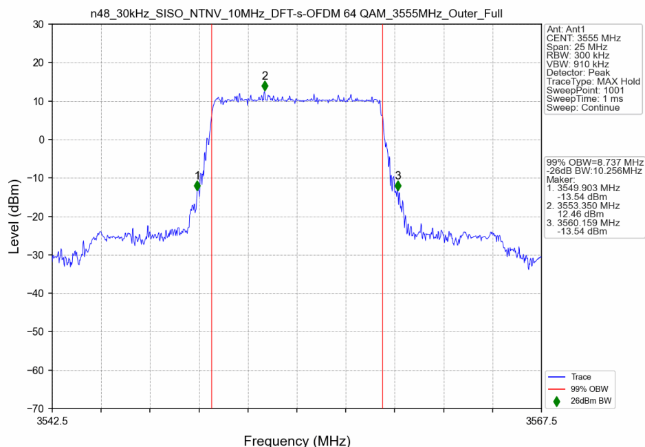
n48_30kHz_SISO_NTNV_10MHz_DFT-s-OFDM 64 QAM_3555MHz_Outer_Full_Ant1
