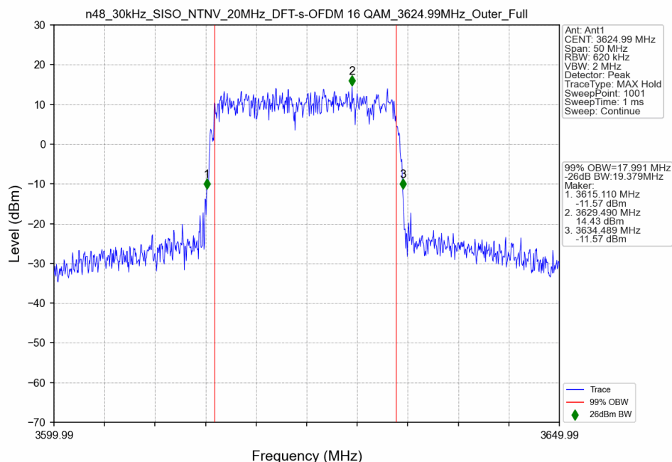
n48_30kHz_SISO_NTNV_20MHz_DFT-s-OFDM 16 QAM_3624.99MHz_Outer_Full_Ant1
