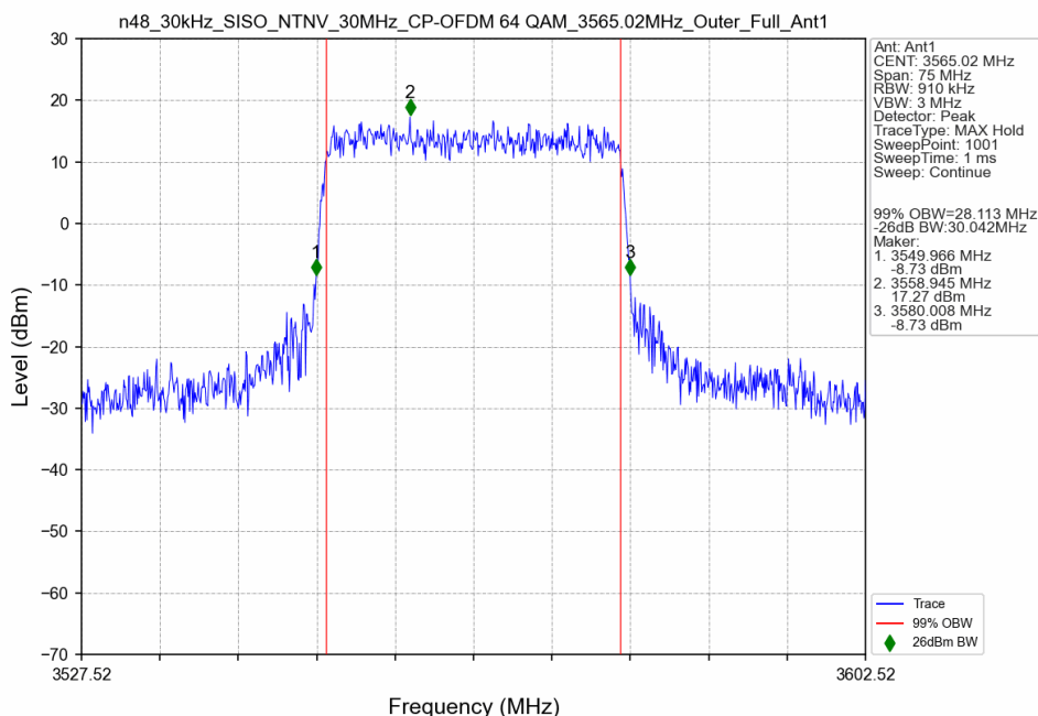
n48_30kHz_SISO_NTNV_30MHz_CP-OFDM 64 QAM_3565.02MHz_Outer_Full_Ant1
