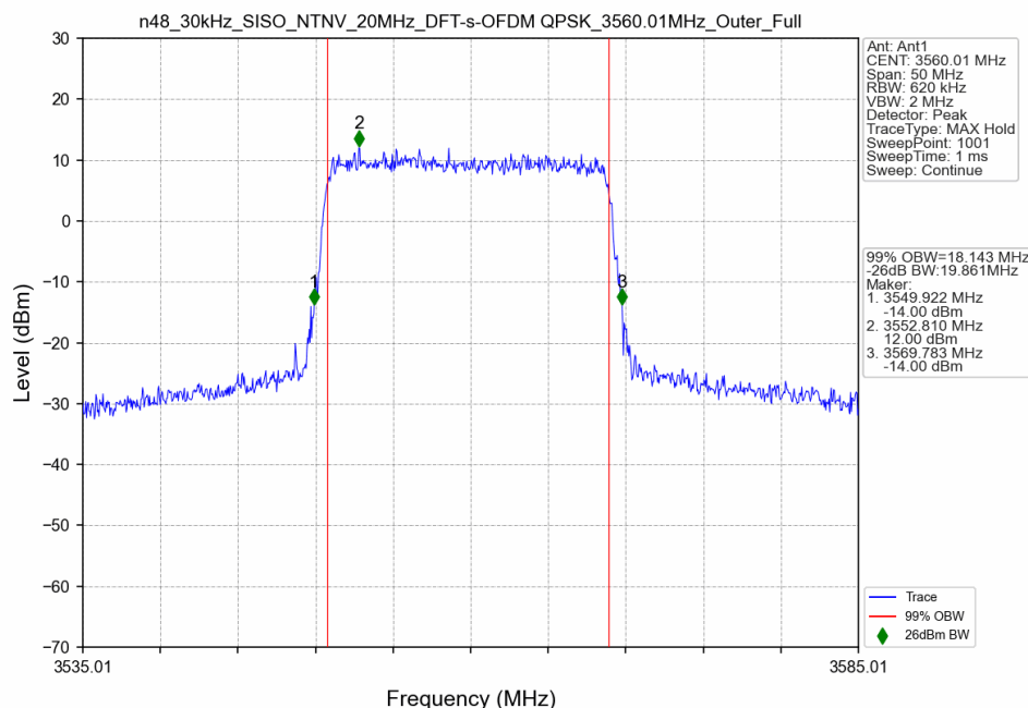
n48_30kHz_SISO_NTNV_20MHz_DFT-s-OFDM QPSK_3560.01MHz_Outer_Full_Ant1
