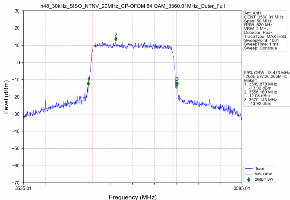
n48_30kHz_SISO_NTNV_20MHz_CP-OFDM 64 QAM_3560.01MHz_Outer_Full_Ant1
