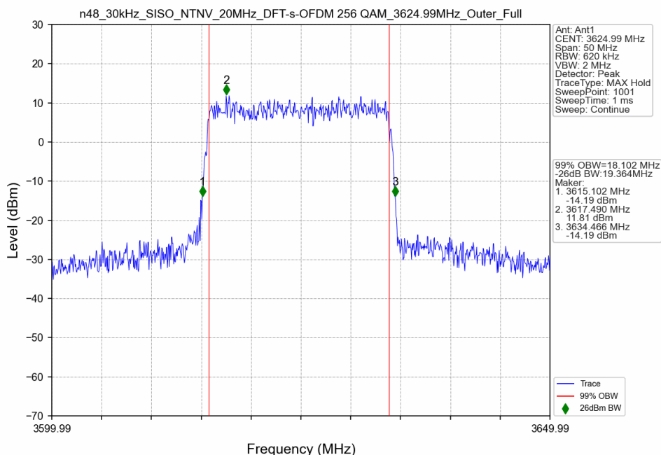
n48_30kHz_SISO_NTNV_20MHz_DFT-s-OFDM 256 QAM_3624.99MHz_Outer_Full_Ant1
