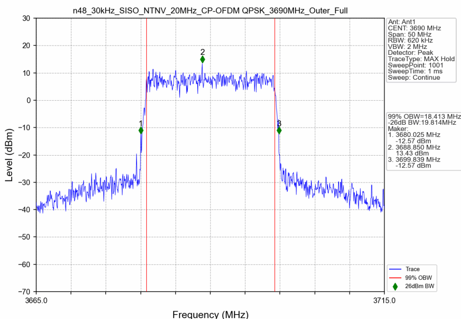
n48_30kHz_SISO_NTNV_20MHz_CP-OFDM QPSK_3690MHz_Outer_Full_Ant1
