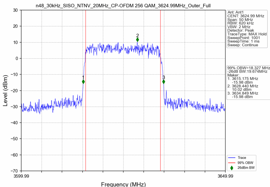
n48_30kHz_SISO_NTNV_20MHz_CP-OFDM 256 QAM_3624.99MHz_Outer_Full_Ant1
