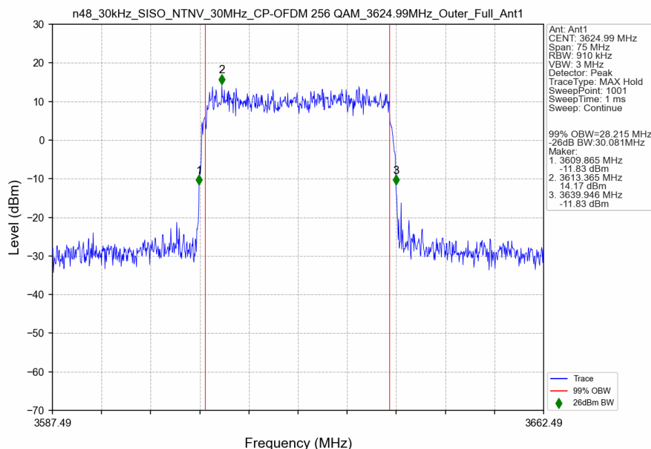
n48_30kHz_SISO_NTNV_30MHz_CP-OFDM 256 QAM_3624.99MHz_Outer_Full_Ant1
