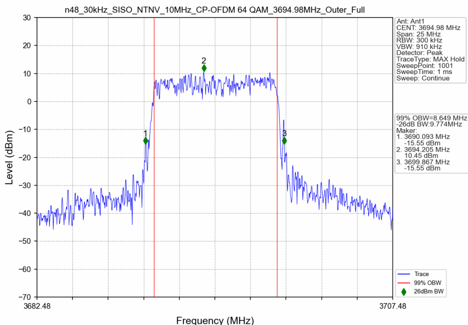
n48_30kHz_SISO_NTNV_10MHz_CP-OFDM 64 QAM_3694.98MHz_Outer_Full_Ant1
