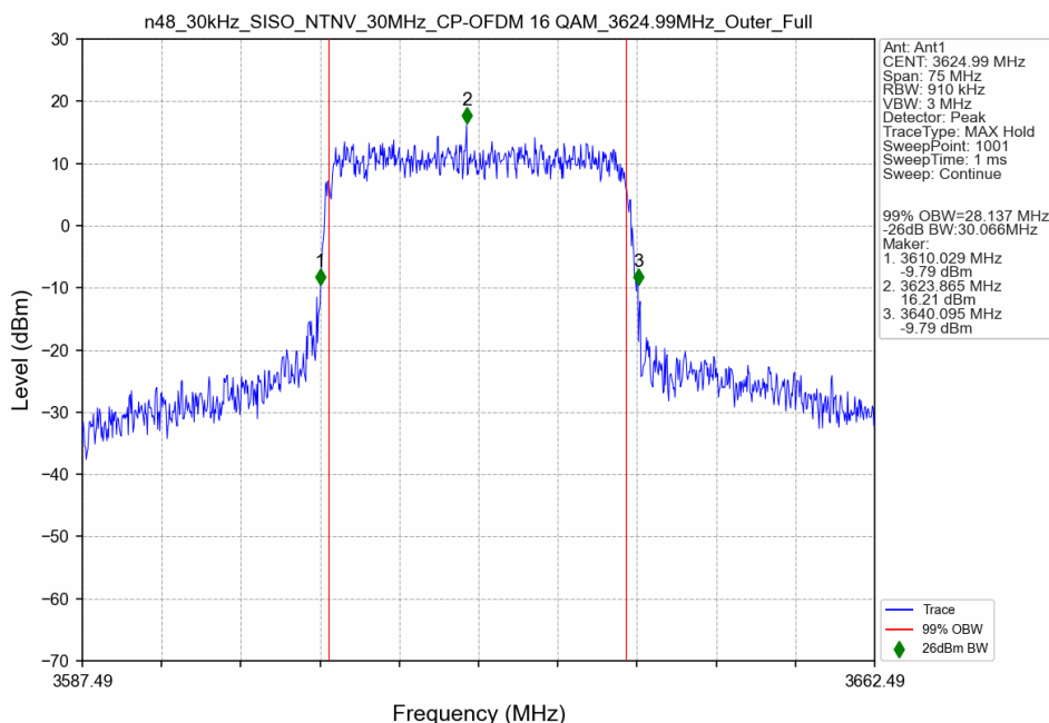
n48_30kHz_SISO_NTNV_30MHz_CP-OFDM 16 QAM_3624.99MHz_Outer_Full_Ant1
