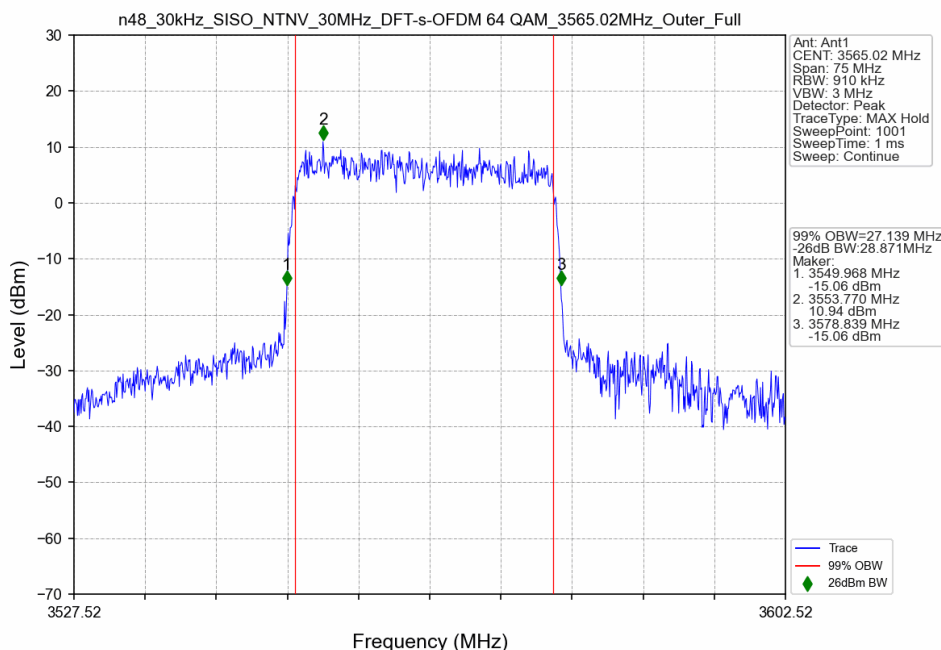
n48_30kHz_SISO_NTNV_30MHz_DFT-s-OFDM 64 QAM_3565.02MHz_Outer_Full_Ant1
