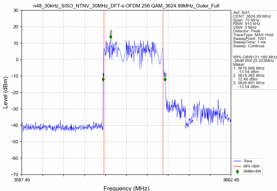
n48_30kHz_SISO_NTNV_30MHz_DFT-s-OFDM 256 QAM_3624.99MHz_Outer_Full_Ant1
