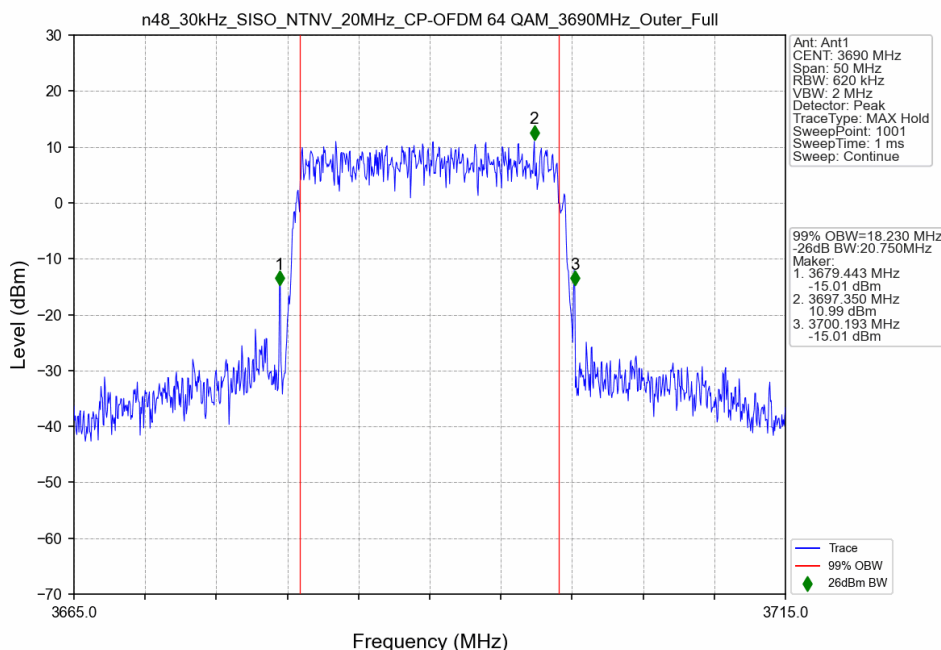
n48_30kHz_SISO_NTNV_20MHz_CP-OFDM 64 QAM_3690MHz_Outer_Full_Ant1
