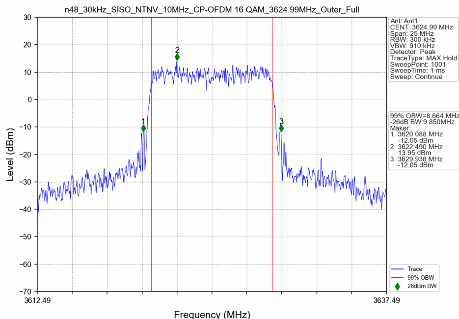
n48_30kHz_SISO_NTNV_10MHz_CP-OFDM 16 QAM_3624.99MHz_Outer_Full_Ant1
