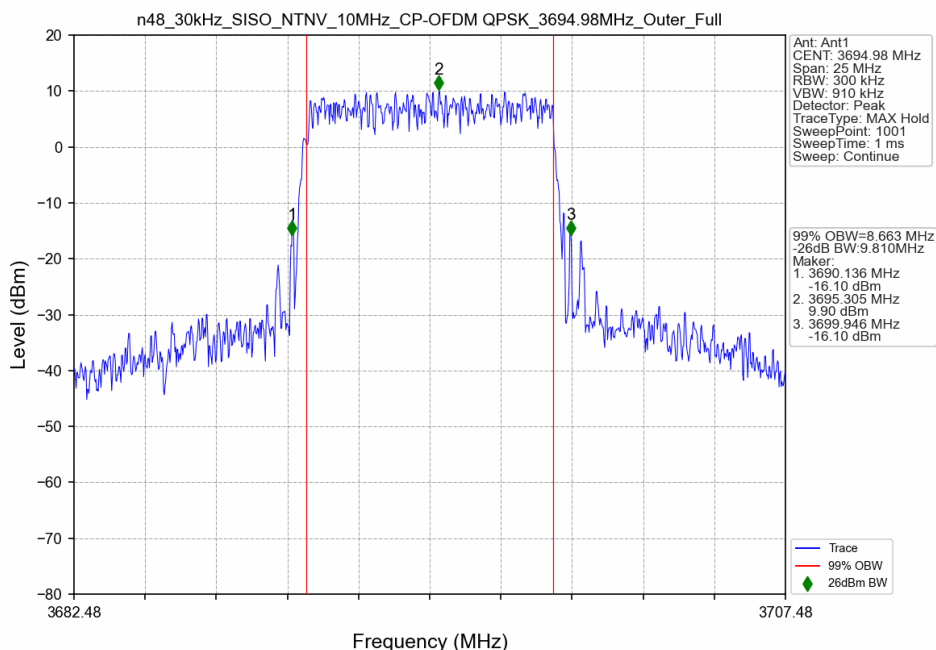
n48_30kHz_SISO_NTNV_10MHz_CP-OFDM QPSK_3694.98MHz_Outer_Full_Ant1
