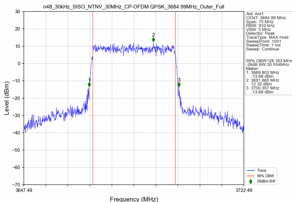
n48_30kHz_SISO_NTNV_30MHz_CP-OFDM QPSK_3684.99MHz_Outer_Full_Ant1
