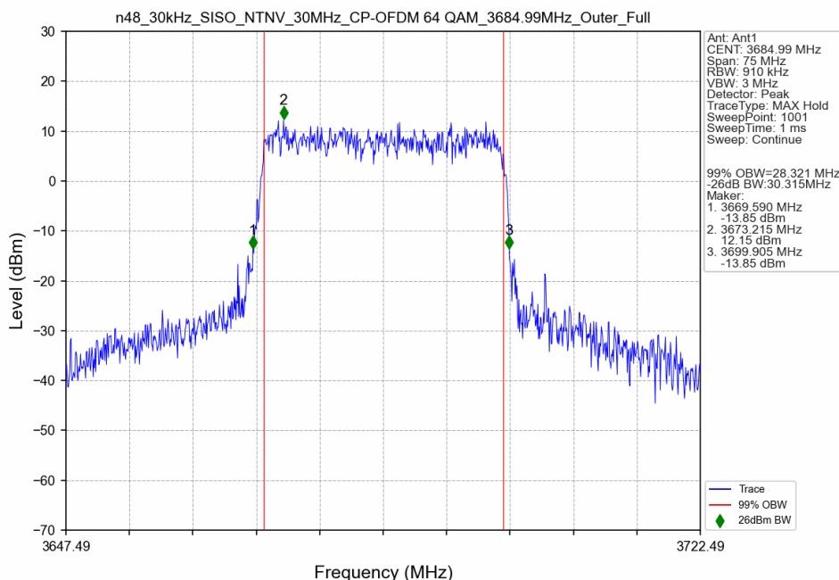
n48_30kHz_SISO_NTNV_30MHz_CP-OFDM 64 QAM_3684.99MHz_Outer_Full_Ant1
