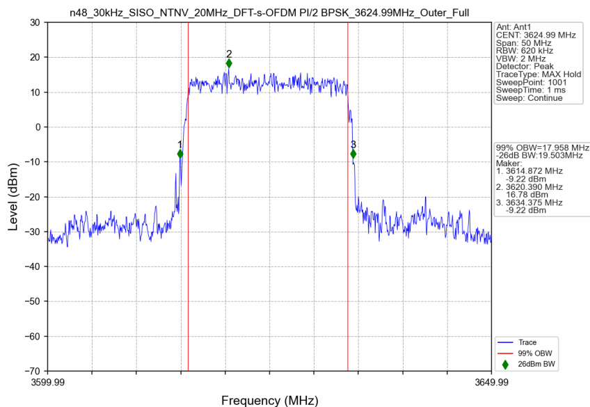
n48_30kHz_SISO_NTNV_20MHz_DFT-s-OFDM PI/2 BPSK_3624.99MHz_Outer_Full_Ant1
