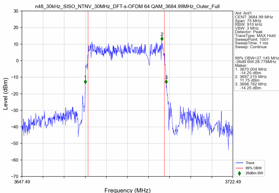
n48_30kHz_SISO_NTNV_30MHz_DFT-s-OFDM 64 QAM_3684.99MHz_Outer_Full_Ant1
