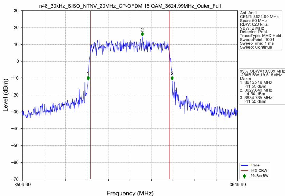
n48_30kHz_SISO_NTNV_20MHz_CP-OFDM 16 QAM_3624.99MHz_Outer_Full_Ant1
