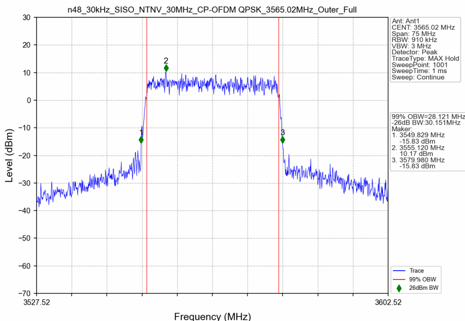
n48_30kHz_SISO_NTNV_30MHz_CP-OFDM QPSK_3565.02MHz_Outer_Full_Ant1
