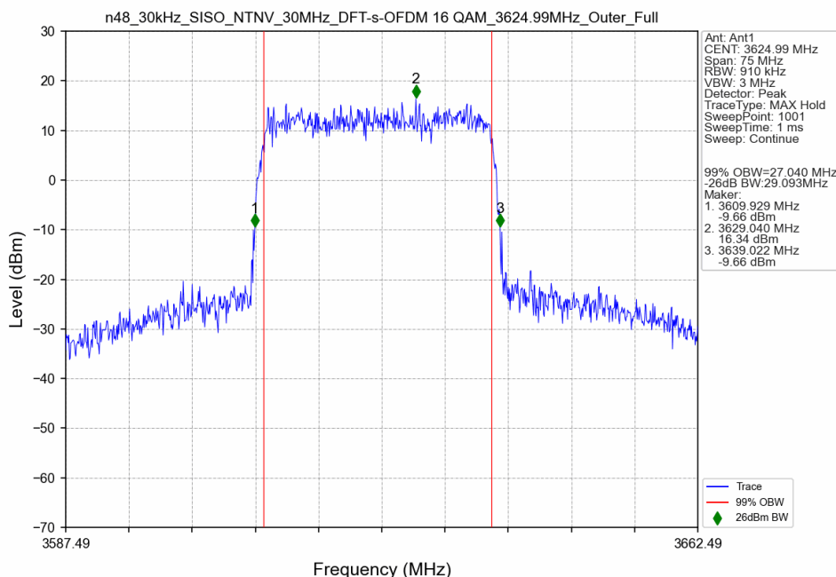
n48_30kHz_SISO_NTNV_30MHz_DFT-s-OFDM 16 QAM_3624.99MHz_Outer_Full_Ant1
