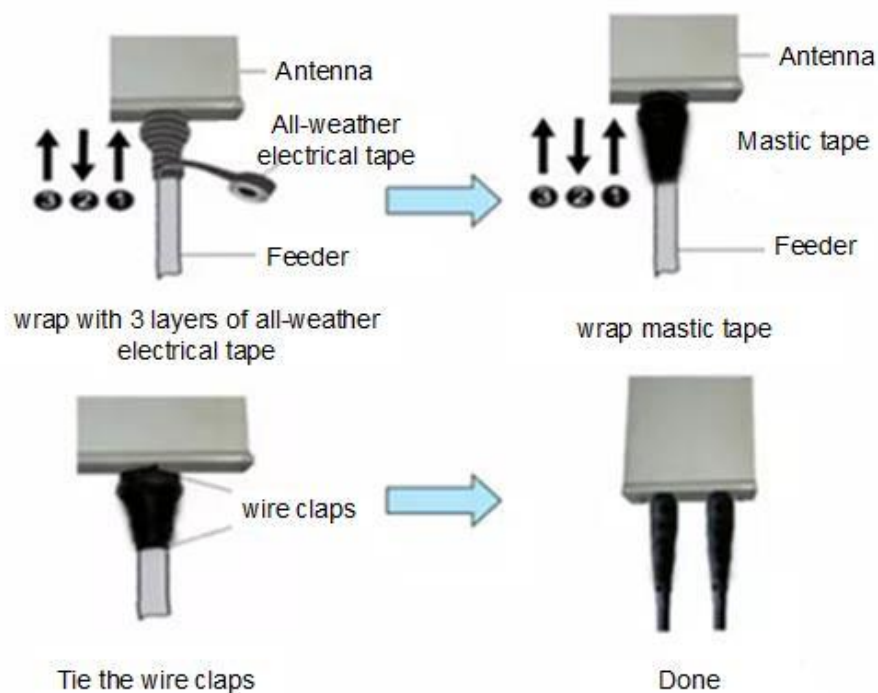
Figure 3-1 Antenna Weatherproofing
