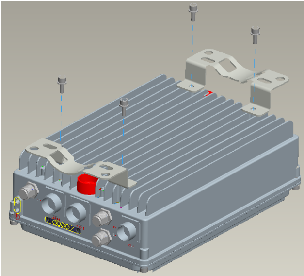
Figure 4-19 Install the Mounting Bracket
