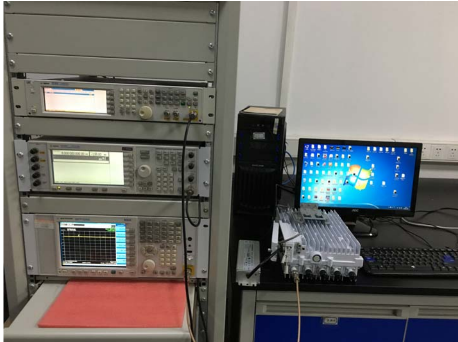
Conducted Measurements
