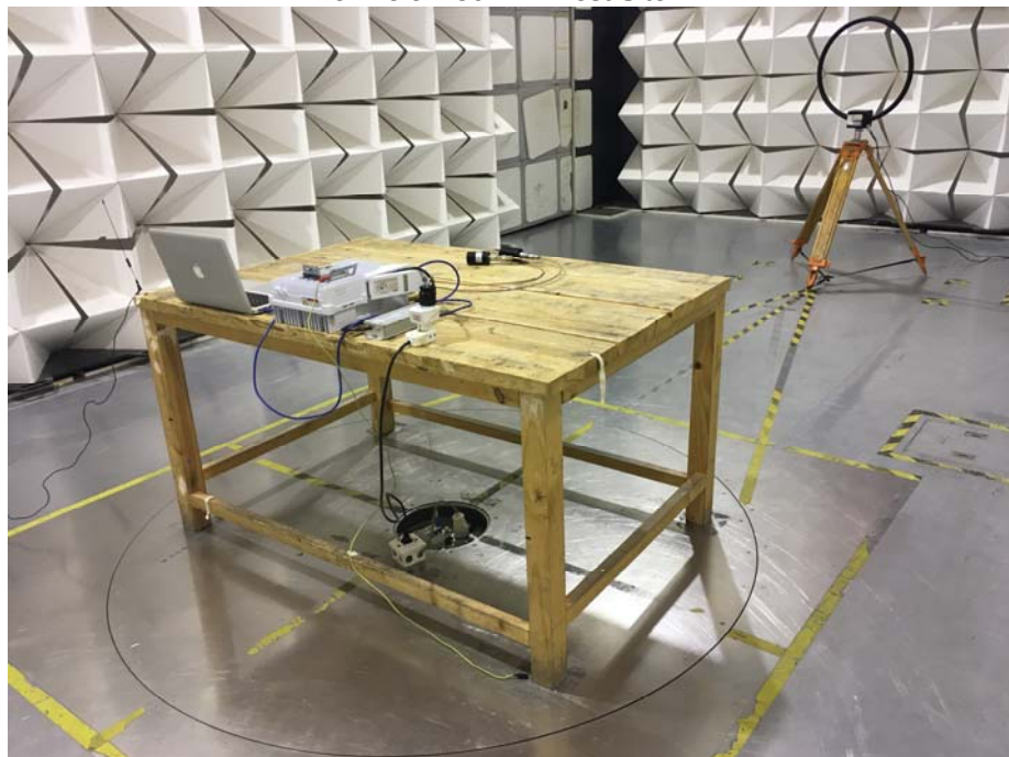
For Below 30MHz Test Site 2#
